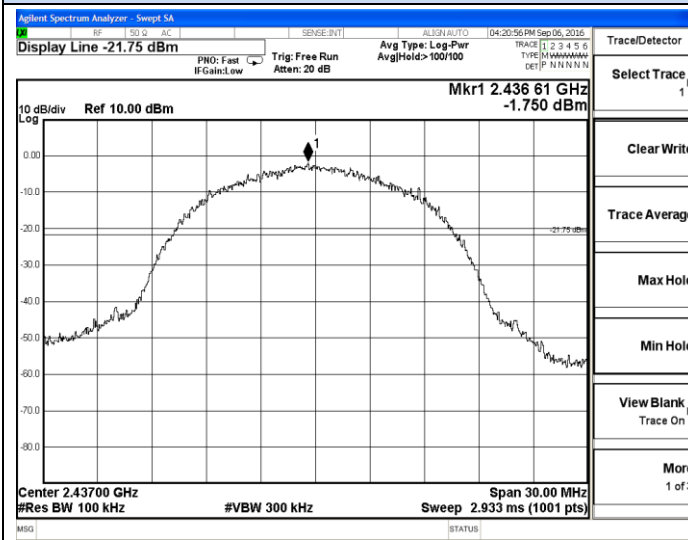
802.11b-Middle channel Reference
