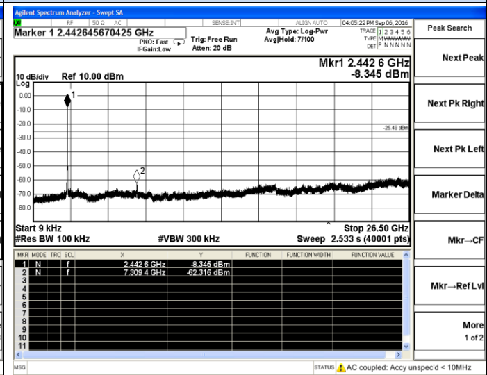
802.11n(HT20)-Middle channel
