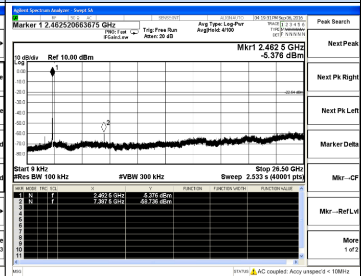
802.11b-High channel
