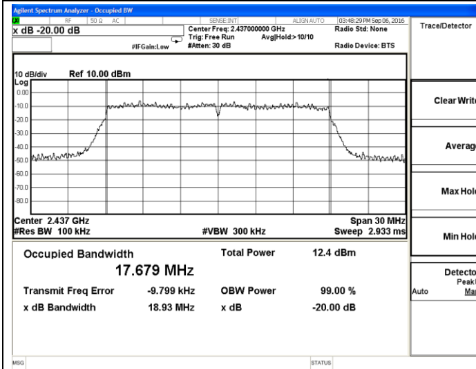
802.11n(HT20)-Middle channel
