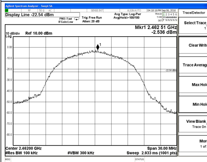
802.11b-High channel Reference
