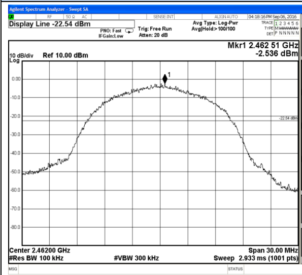
802.11b-High channel
