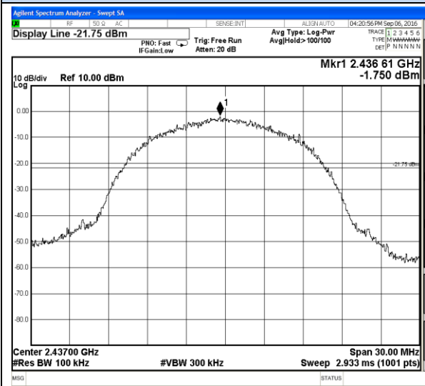
802.11b-Middle channel
