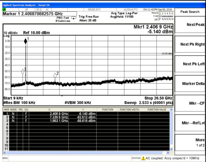
802.11g-Low channel
