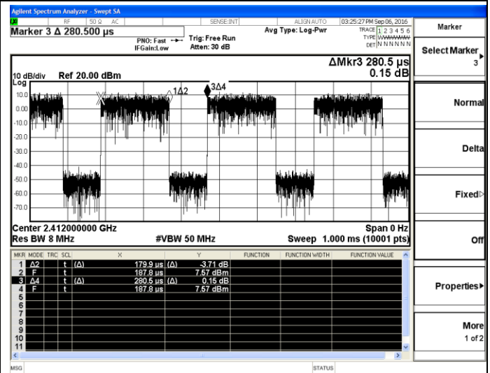
802.11g
