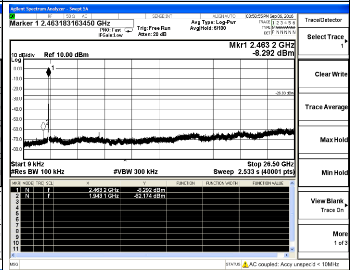
802.11n(HT20)-High channel
