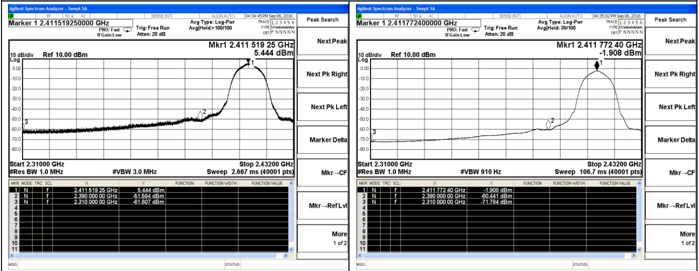
802.11b-Low channel(Peak)
