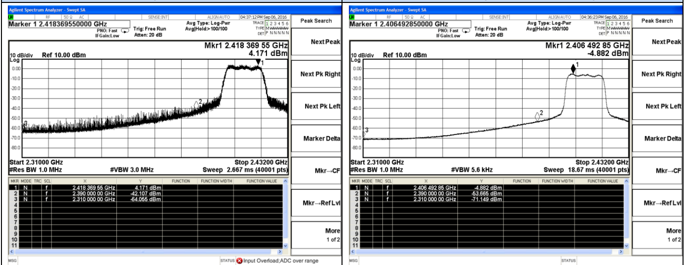
802.11g-Low channel(Peak)
