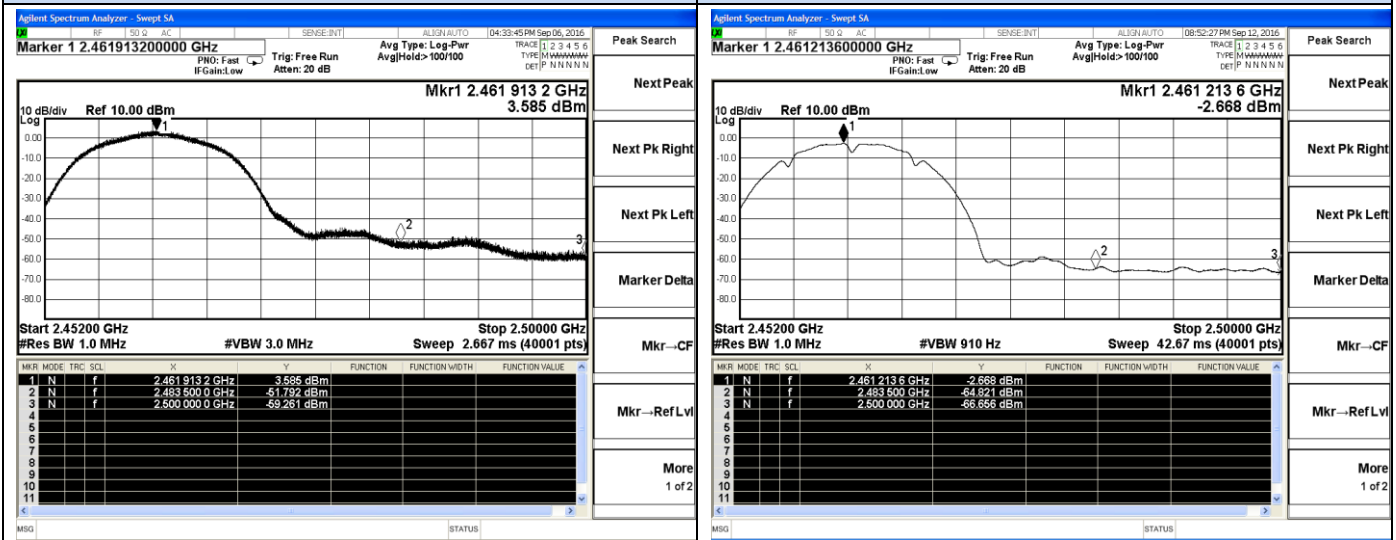
802.11b-High channel(Peak)
