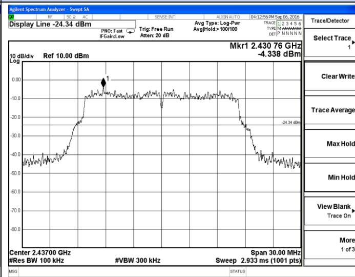
802.11g-Middle channel
