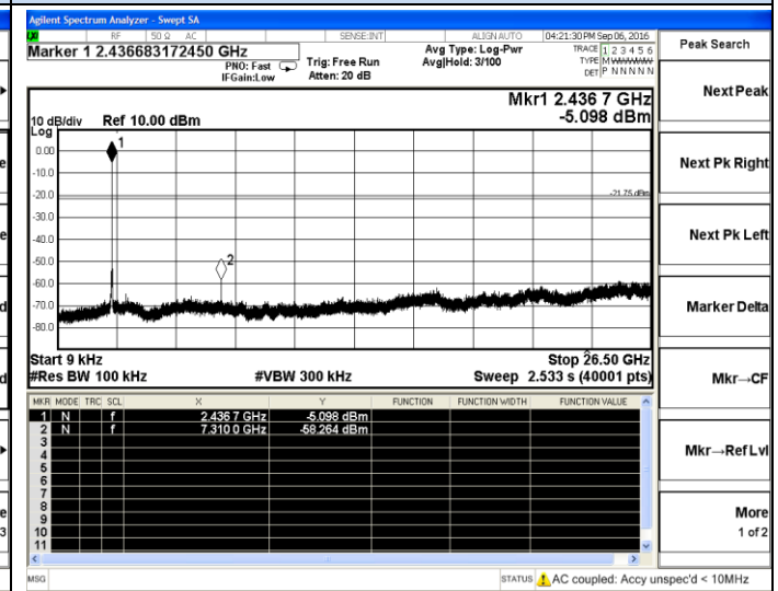
802.11b-Middle channel
