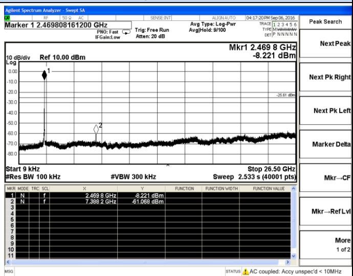
802.11g-High channel
