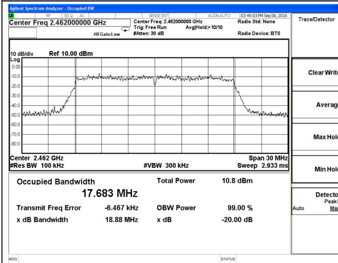
802.11n(HT20)-High channel
