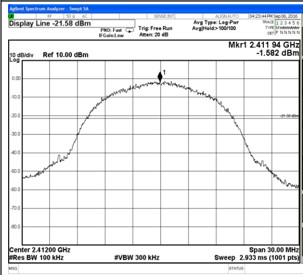
802.11b-Low channel
