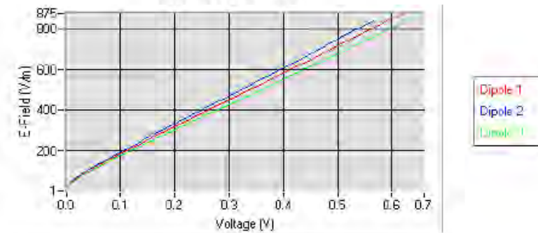
Calibration curves
