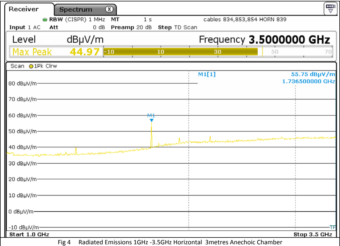
Fig 4 Radiated Emissions 1GHz -3.5GHz Horizontal 3metres Anechoic Chamber
