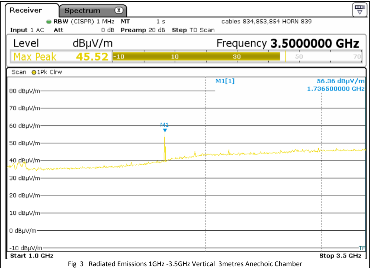
Fig 3 Radiated Emissions 1GHz -3.5GHz Vertical 3metres Anechoic Chamber
