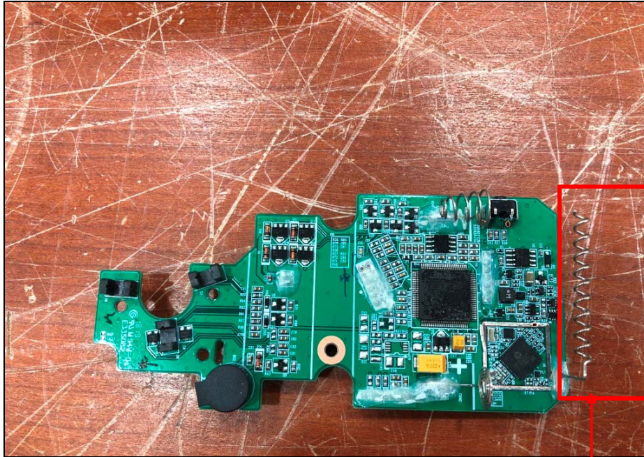
Helical Antenna
