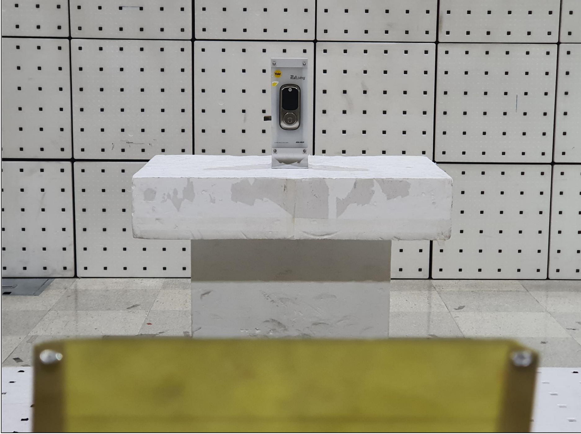
Radiated Emission (Above 1 GHz) _ Front_ (Test Model : YRD622-ACC)
