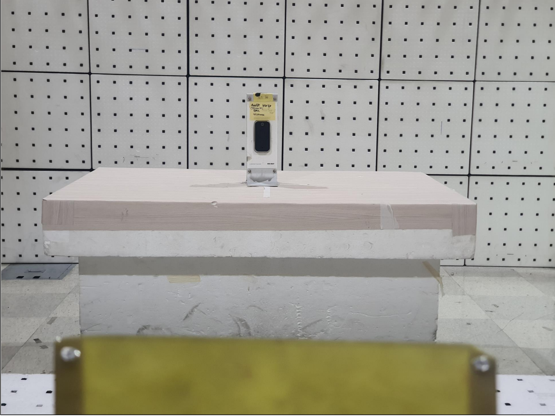
Radiated Emission (Above 1 GHz) _ Front [Alt. Model : YRD420 FP]
