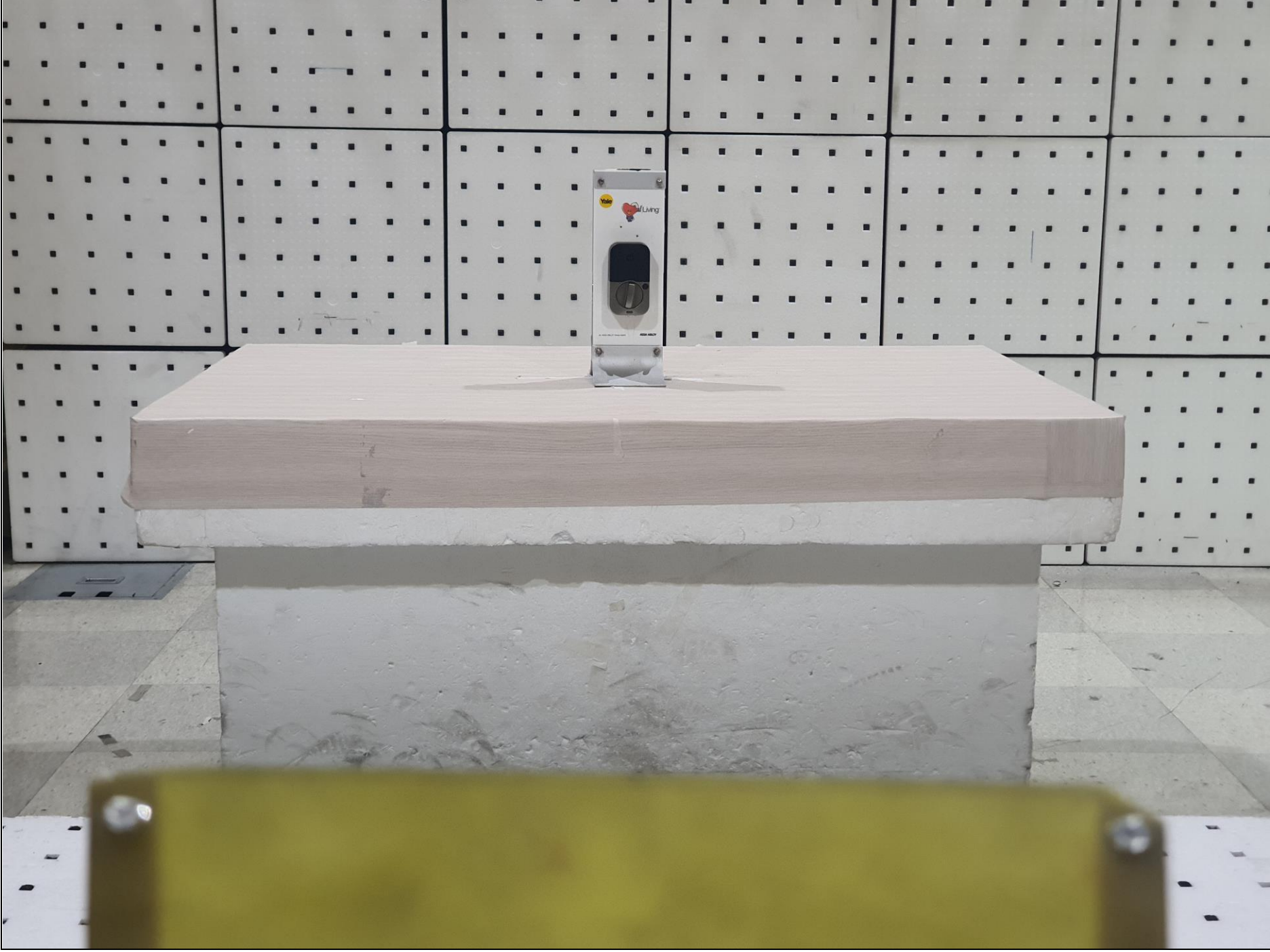
Radiated Emission (Above 1 GHz) _ Rear [Alt. Model : YRD420 FP]
