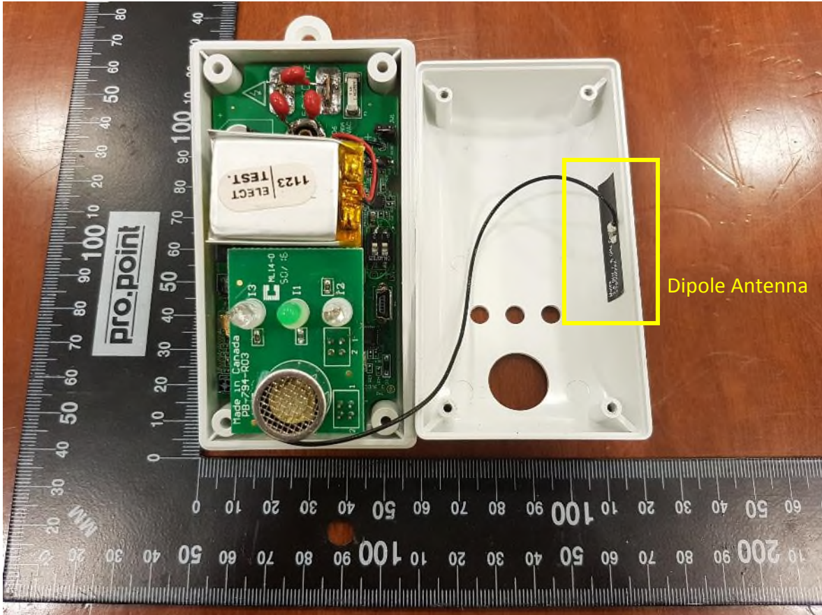
Figure 1 – EUT Internal Photo
