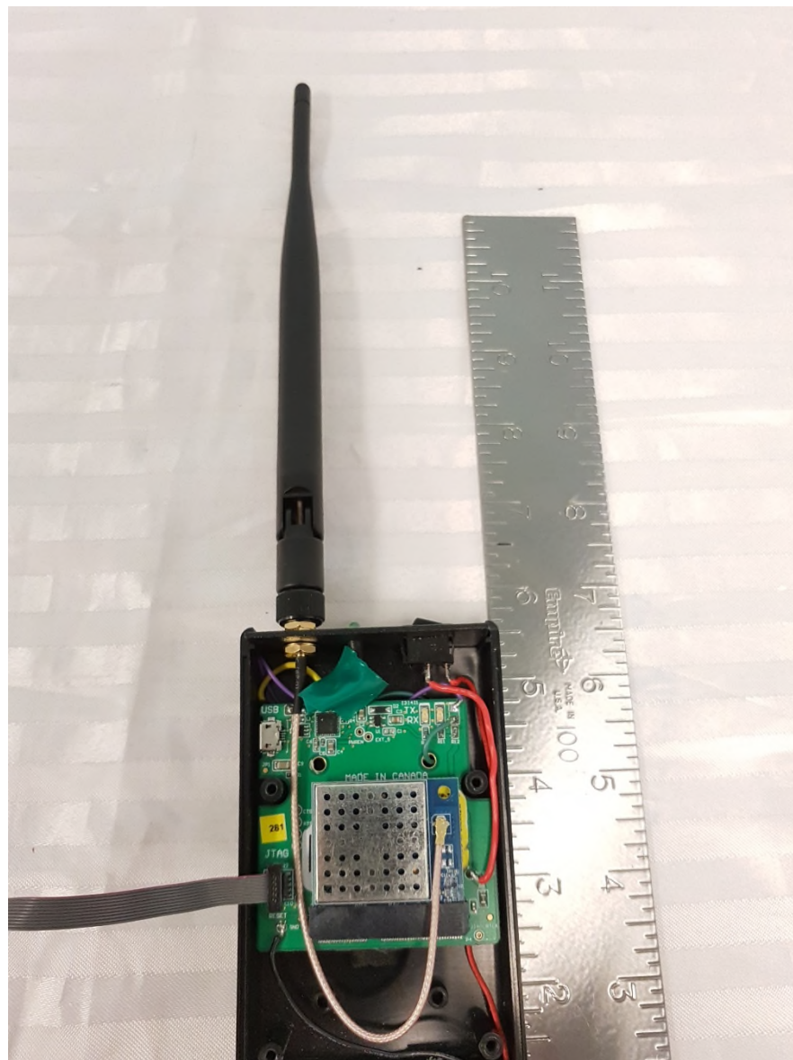
Figure 3 – EUT Internal Photo - Antenna
