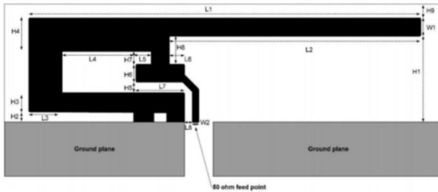
Figure 1. IFA Dimensions
