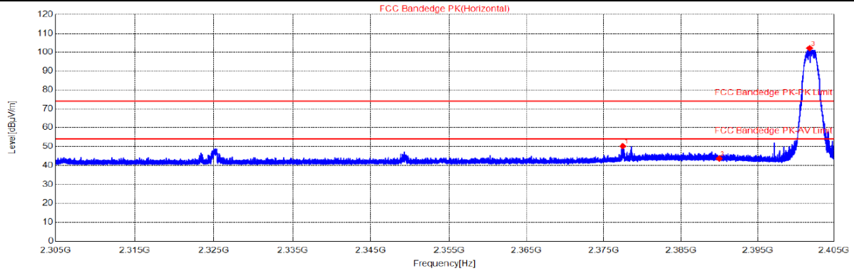
BLE_2402/ Horizontal
