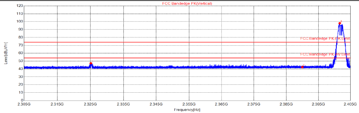
BLE_2402/ Vertical
