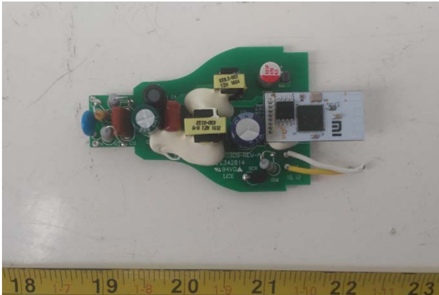
EUT - Main Board Top View
