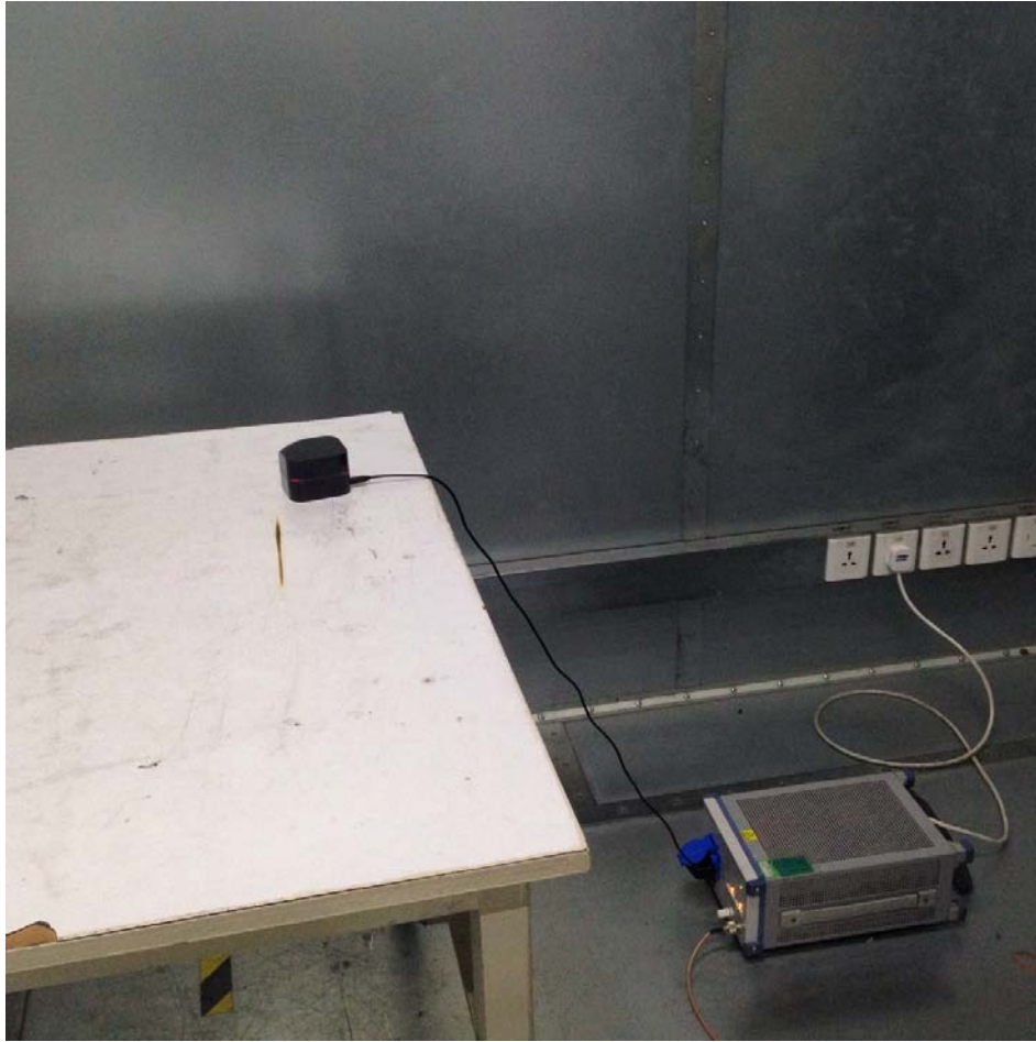
Radiated emissions test
