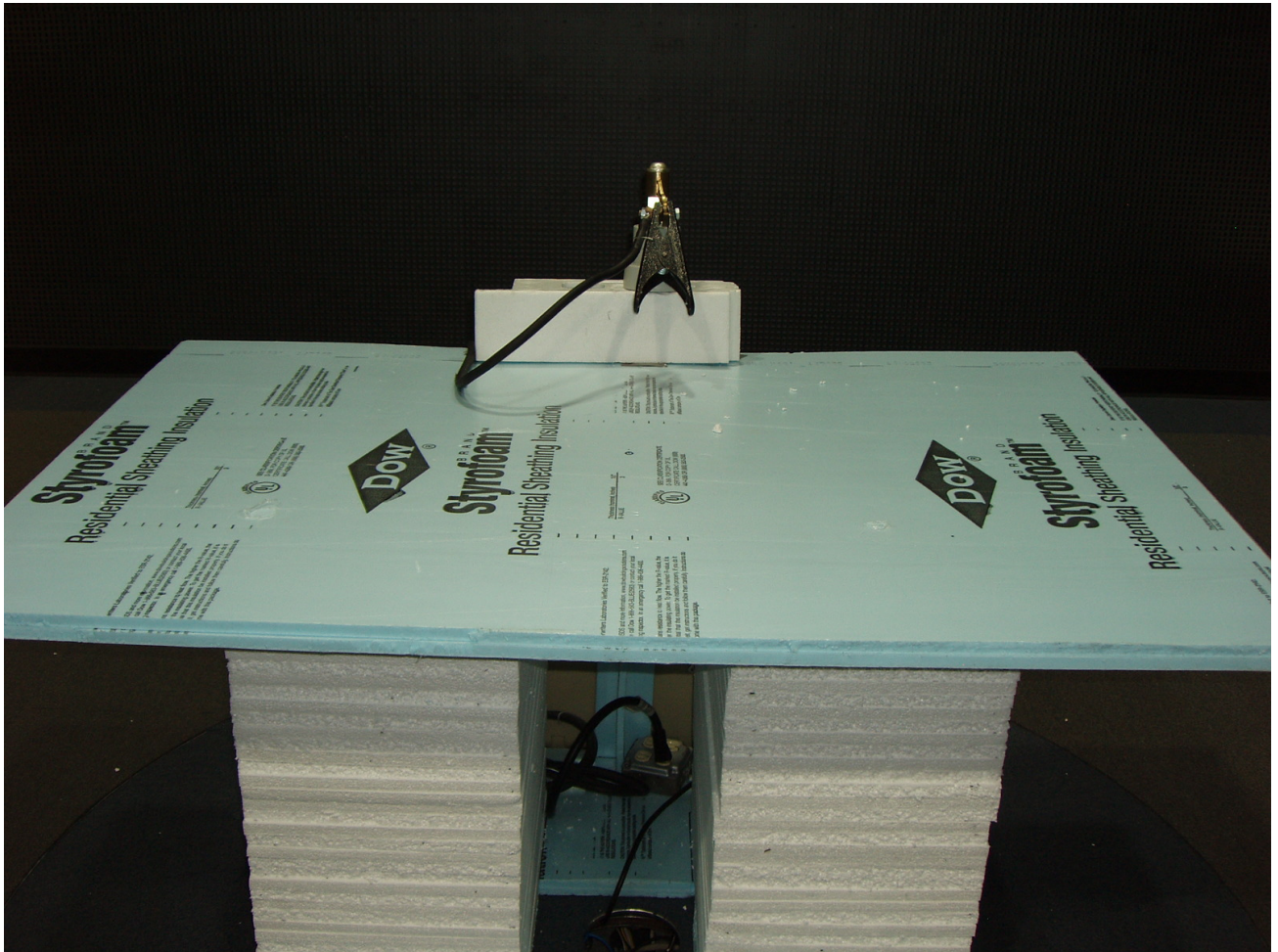
Photo 1 – Front View of the Radiated Emissions Test Set-up
