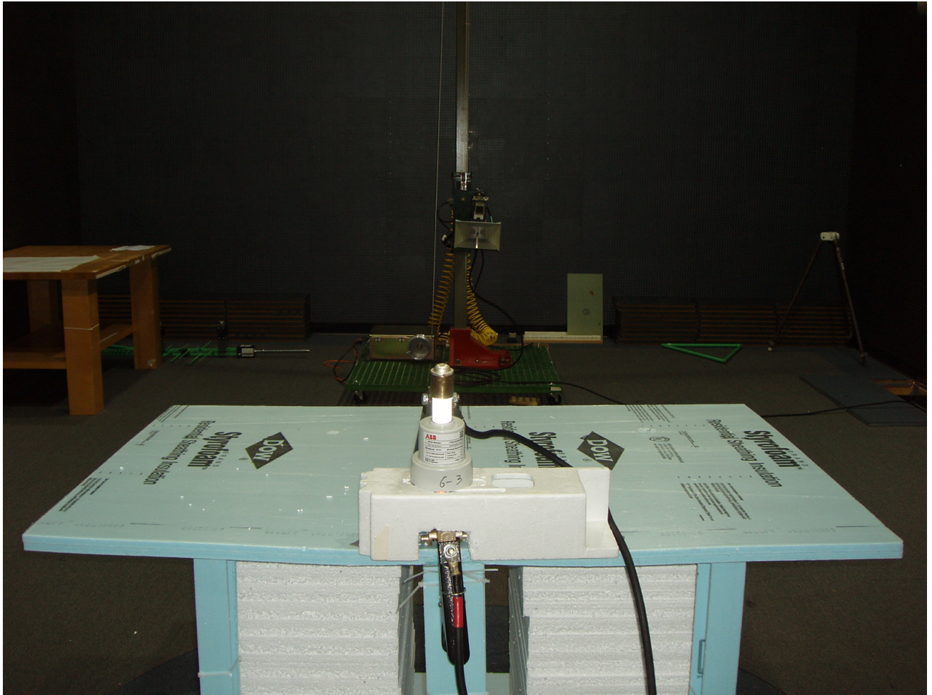
Photo 3 – Rear View of the Radiated Emissions Test Set-up above 1 GHz
