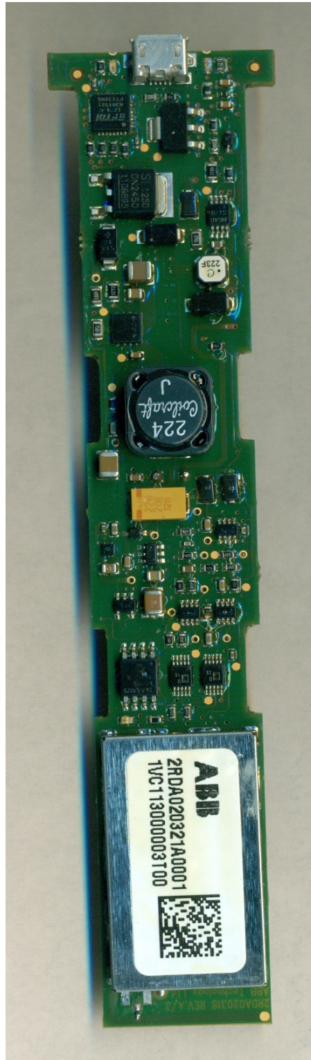
Photo 1 – Top View of the Radio Board
