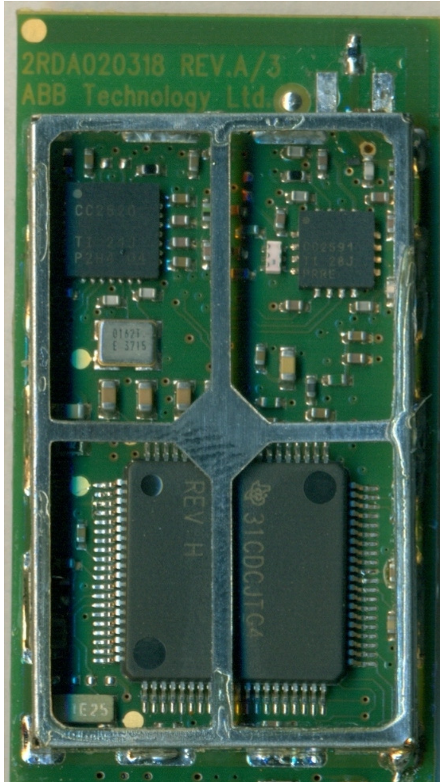
Photo 3 – Top View of the Radio with the Shield Removed
