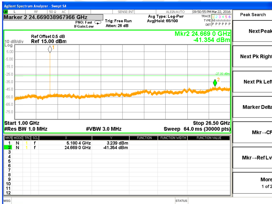
TX Spurious Emissions /802.11a Mode CH 36 (1G-26.5G)
