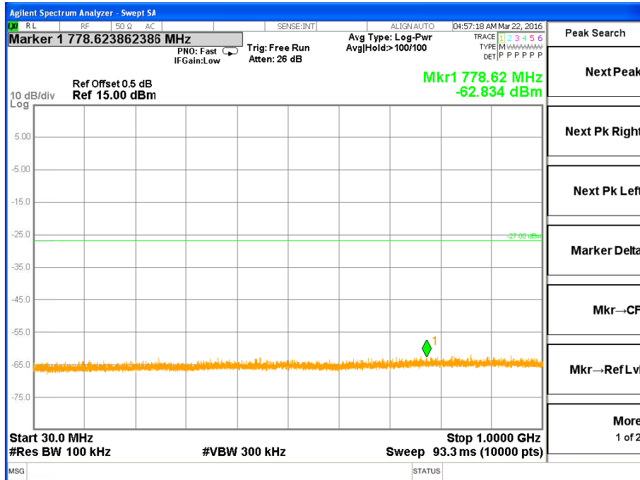
TX Spurious Emissions /802.11a Mode CH 36 (30M-1G)
