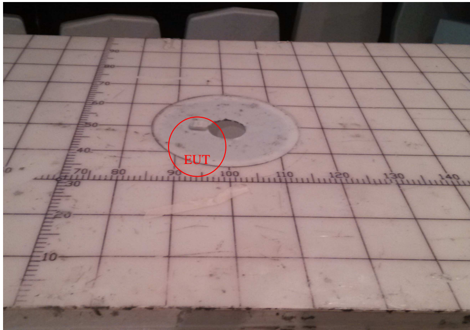
Test Setup Photo –Radiated Emission
