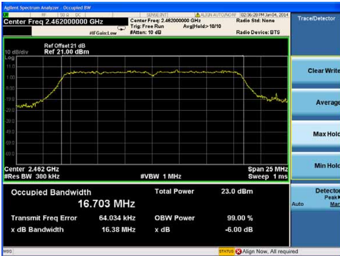
Test Mode: IEEE 802.11n HT20 TX
