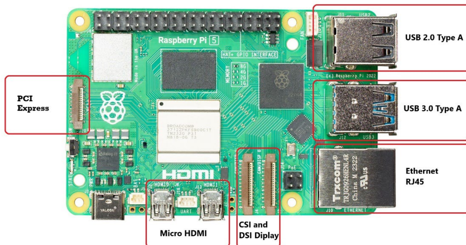
Figure 5 - Peripheral Connections
