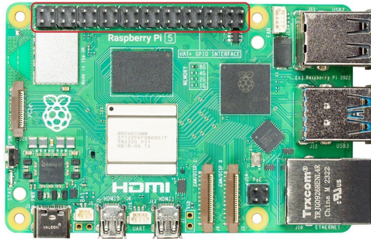
Figure 3 - 40 Pin GPIO Header J8
