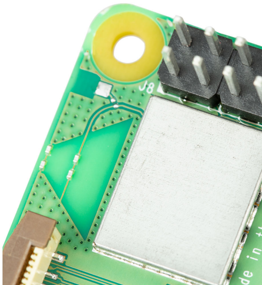
Radio Module and Antenna. Antenna integrated into PCB.
