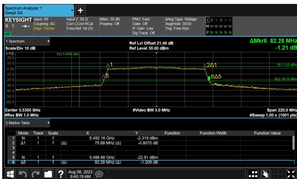
SP1-C0 (1) 5530 MHz (CH106) 26 dB and 99% Bandwidth
