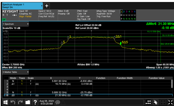
SP1-C0 (1) 5700 MHz (CH140) 26 dB and 99% Bandwidth
