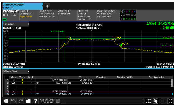
SP1-C0 (1) 5260 MHz (CH52) 26 dB and 99% Bandwidth
