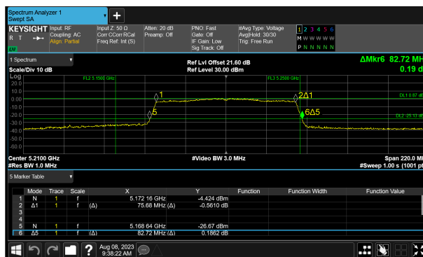
SP1-C0 (1) 5210 MHz (CH42) 26 dB and 99% Bandwidth
