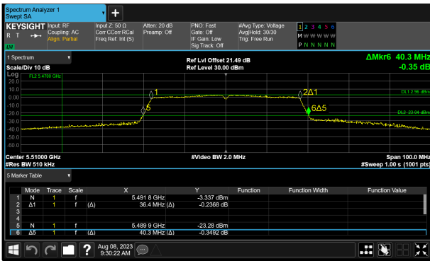
SP1-C0 (1) 5510 MHz (CH102) 26 dB and 99% Bandwidth
