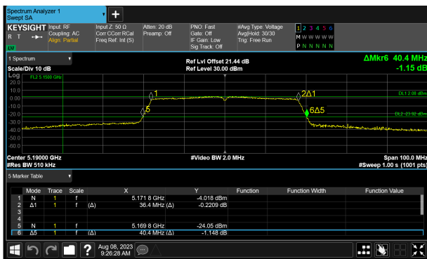
SP1-C0 (1) 5190 MHz (CH38) 26 dB and 99% Bandwidth
