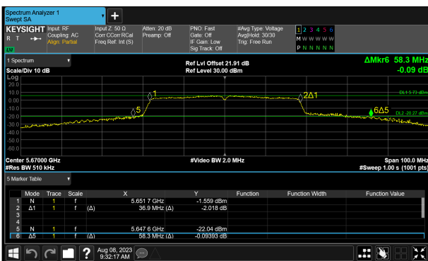
SP1-C0 (1) 5670 MHz (CH134) 26 dB and 99% Bandwidth
