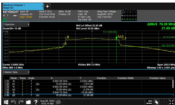
SP1-C0 (1) 5690 MHz (CH138) 26 dB and 99% Bandwidth
