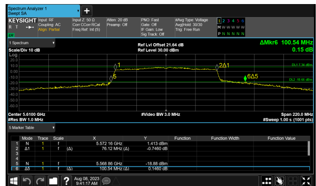
SP1-C0 (1) 5610 MHz (CH122) 26 dB and 99% Bandwidth
