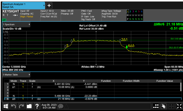
SP1-C0 (1) 5500 MHz (CH100) 26 dB and 99% Bandwidth
