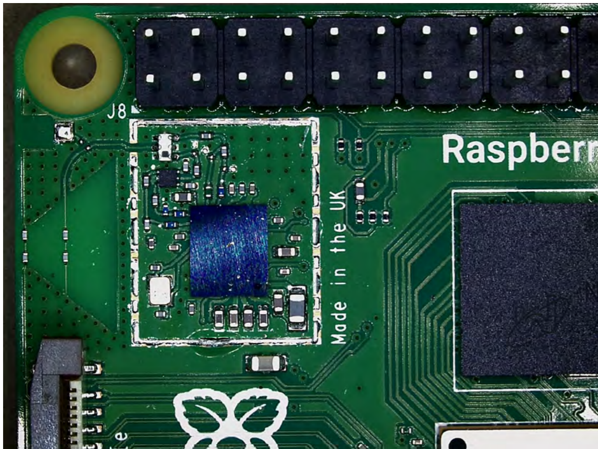
Radio Module Shield Removed Closeup
