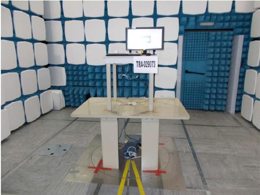
11.5 Test Set-up Photograph
