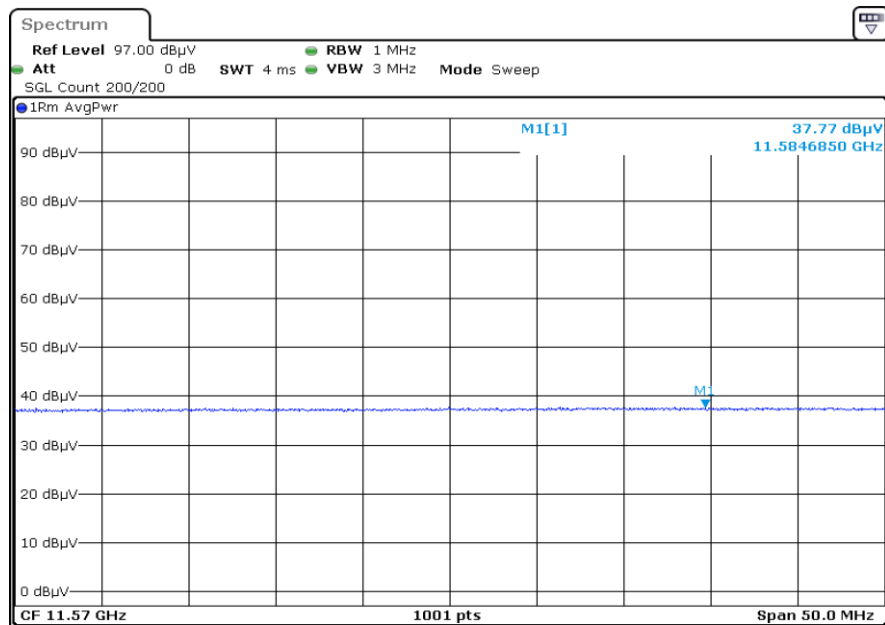
F2 X2 11570.0 Harmonic Vertical AVG
