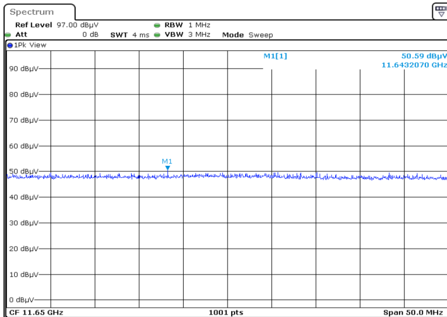
F3 X2 11650.0 Harmonic Horizontal PEAK
