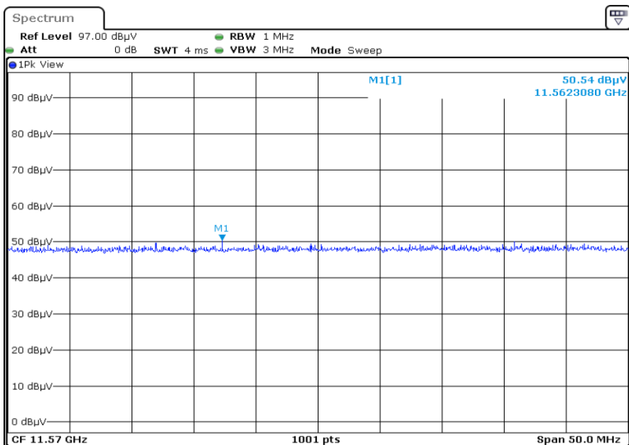
F2 X2 11570.0 Harmonic Vertical PEAK
