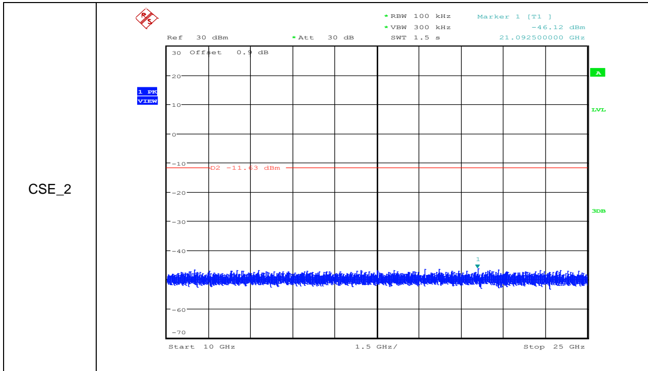
RF Conducted Spurious Emissions_11G_2412_Ant1
