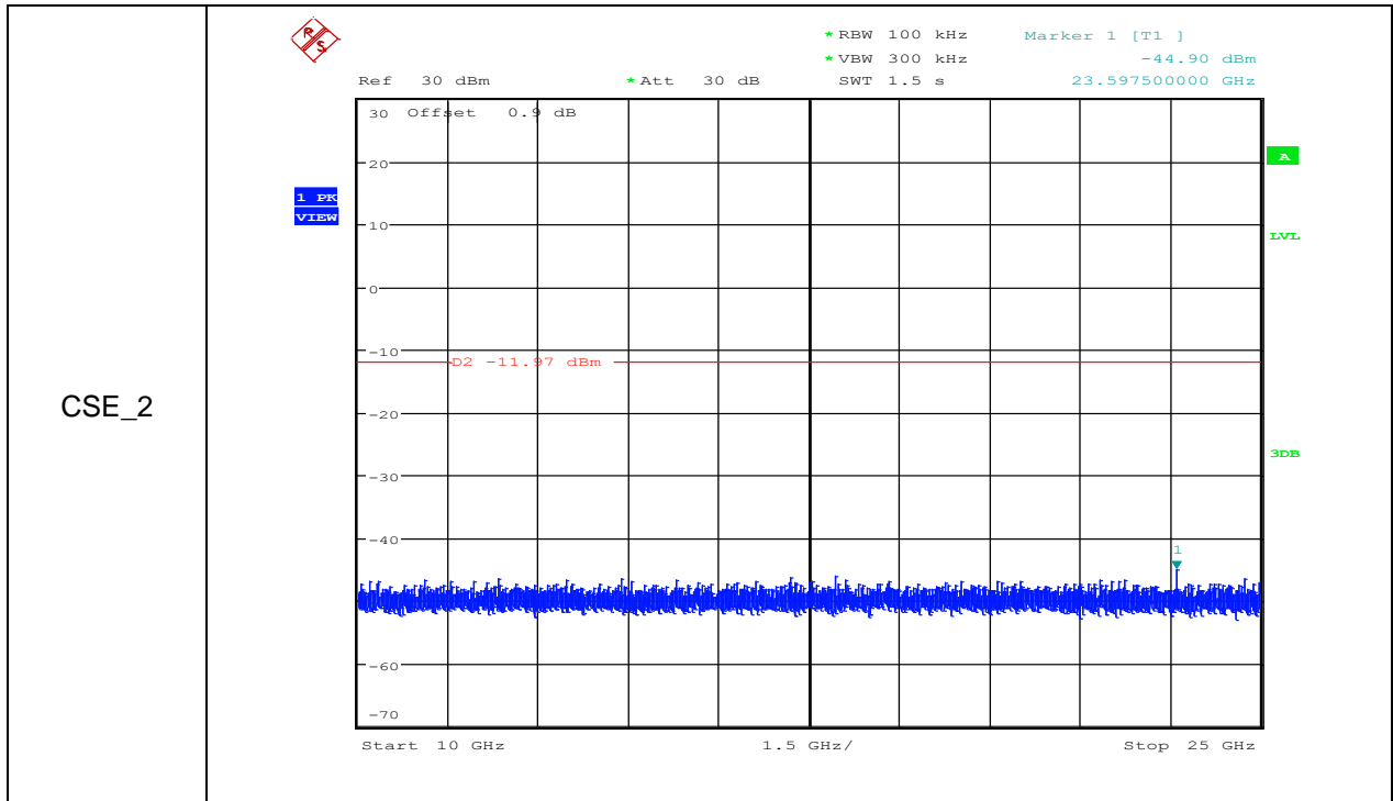
RF Conducted Spurious Emissions_11B_2437_Ant1
