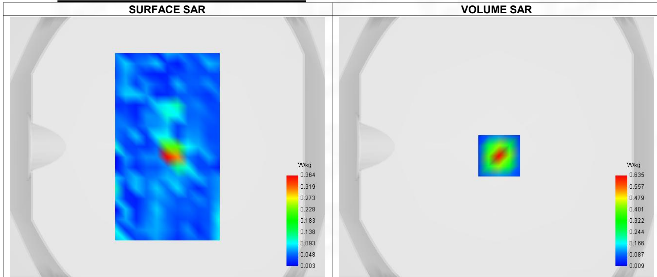
Maximum location: X=2.00, Y=-7.00 ; SAR Peak: 1.02 W/kg
