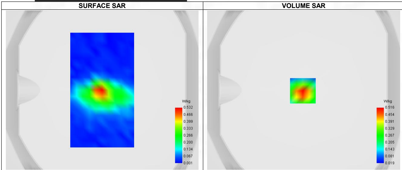
Maximum location: X=-1.00, Y=-1.00 ; SAR Peak: 0.92 W/kg
