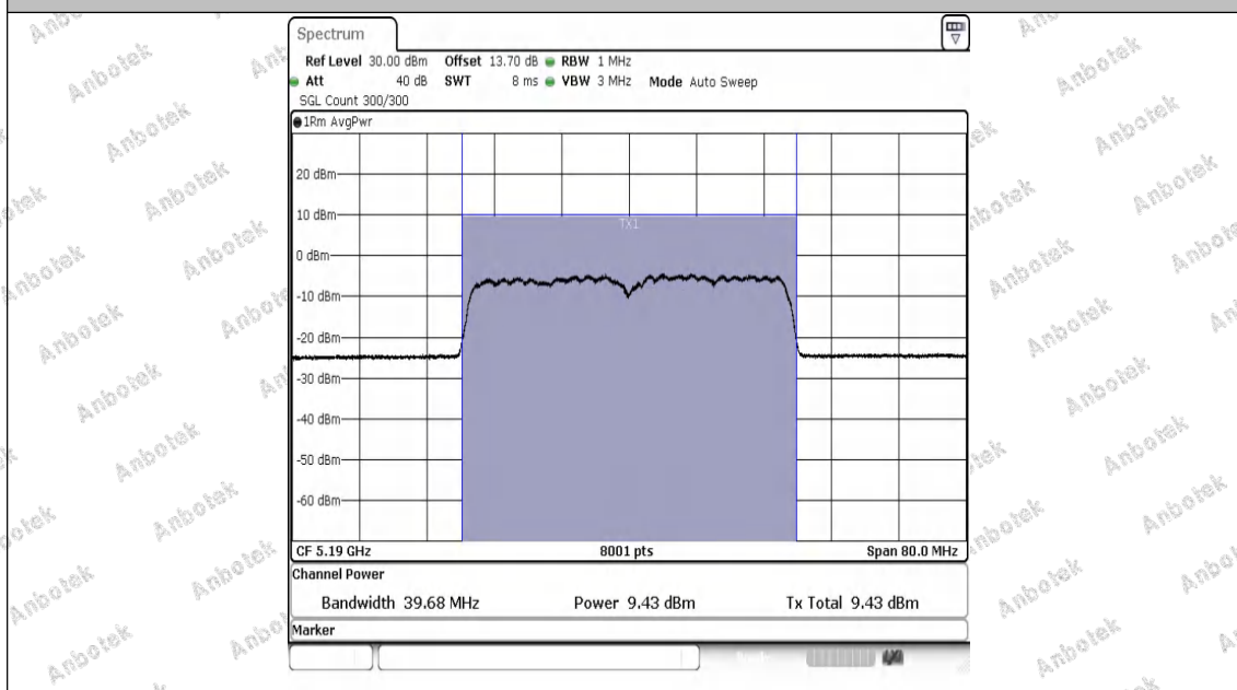
11AX40MIMO-Ant2-5190-PASS
