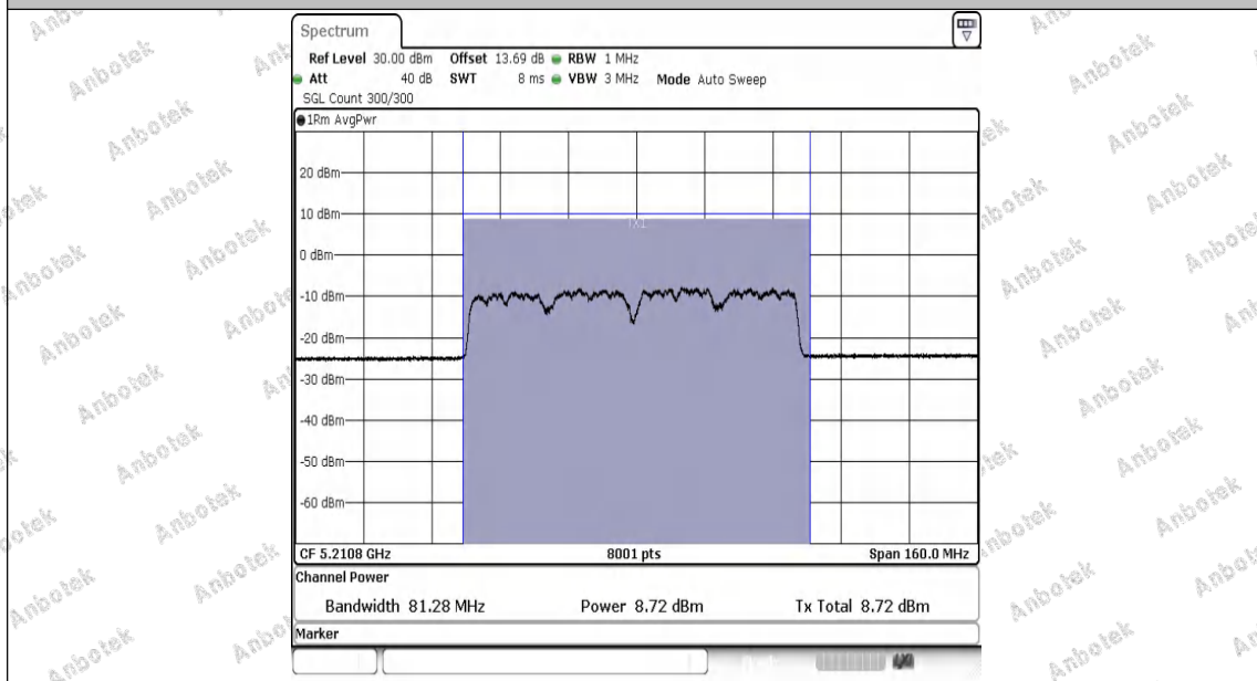
11AC80MIMO-Ant2-5210-PASS
