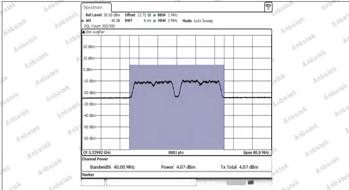
11N40MIMO-Ant1-5230-PASS
