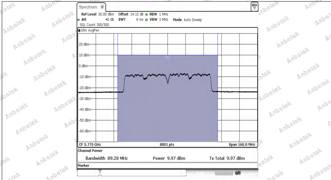
11AC80MIMO-Ant1-5775-PASS
