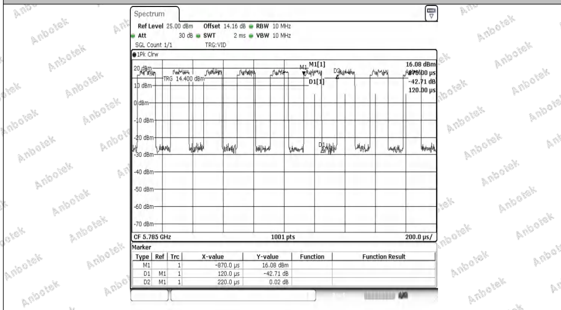
NTNV-11AX20MIMO-Ant2-5785
