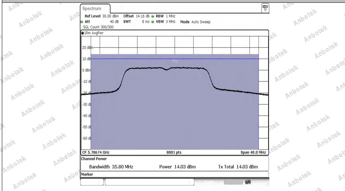
11N20MIMO-Ant2-5785-PASS
