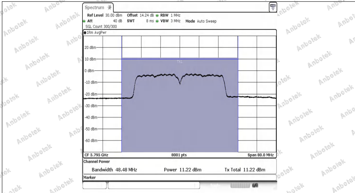
11AC40MIMO-Ant1-5795-PASS
