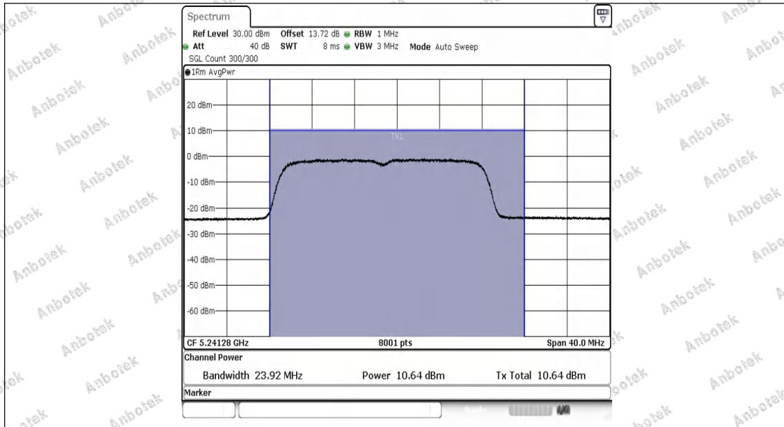
11AX20MIMO-Ant1-5240-PASS
