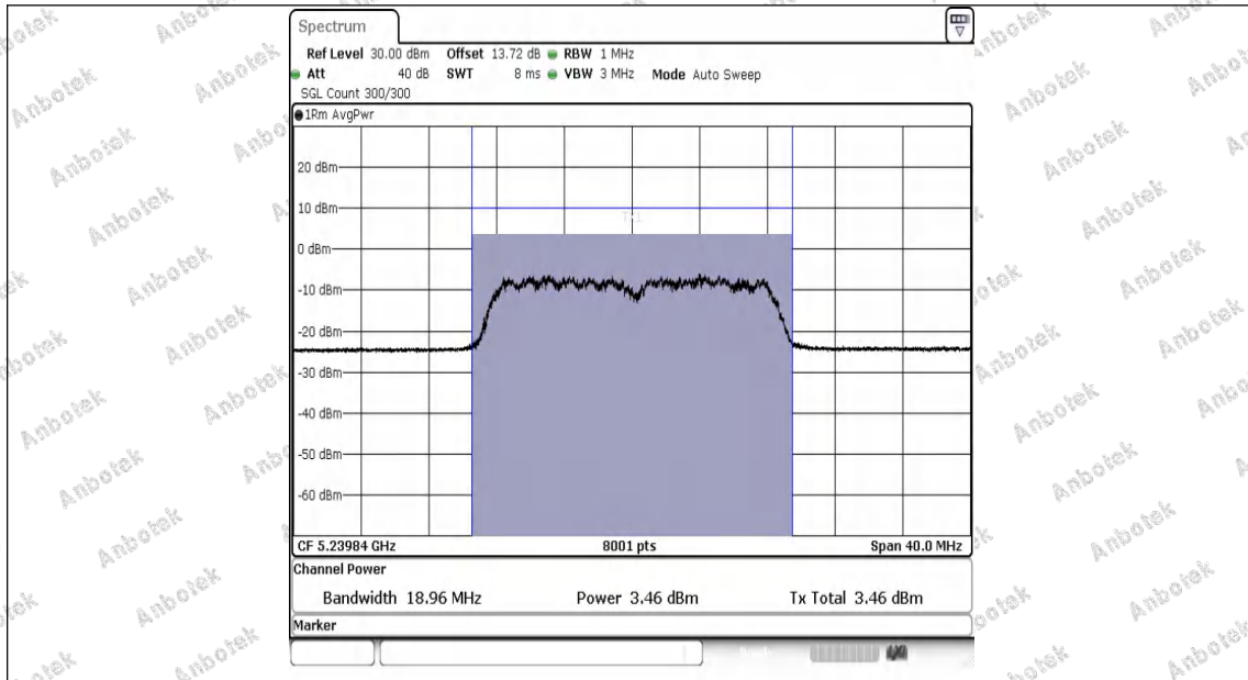
11AC20MIMO-Ant1-5240-PASS
