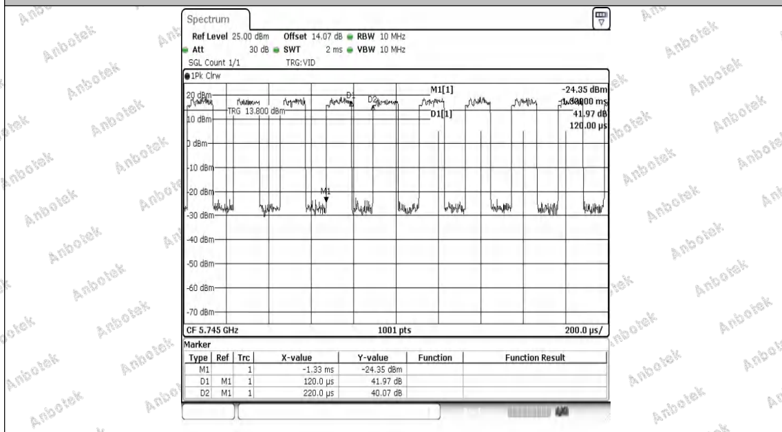
NTNV-11AX20MIMO-Ant2-5745
