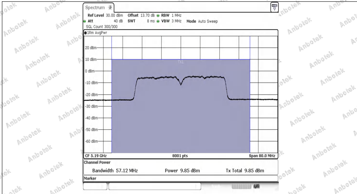
11N40MIMO-Ant1-5190-PASS
