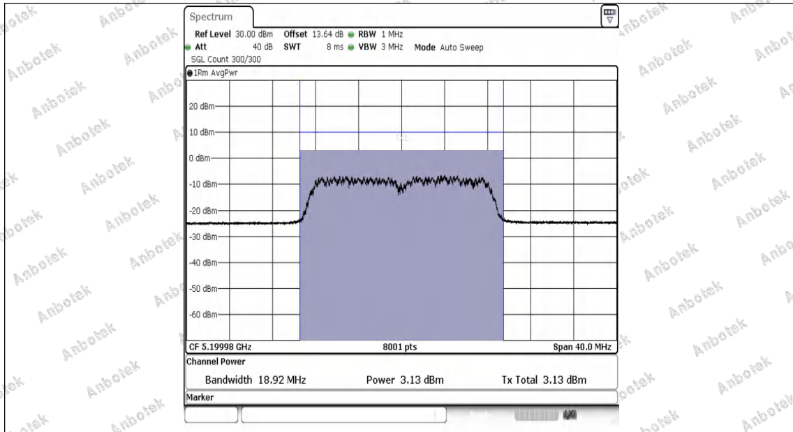
11AC20MIMO-Ant1-5200-PASS
