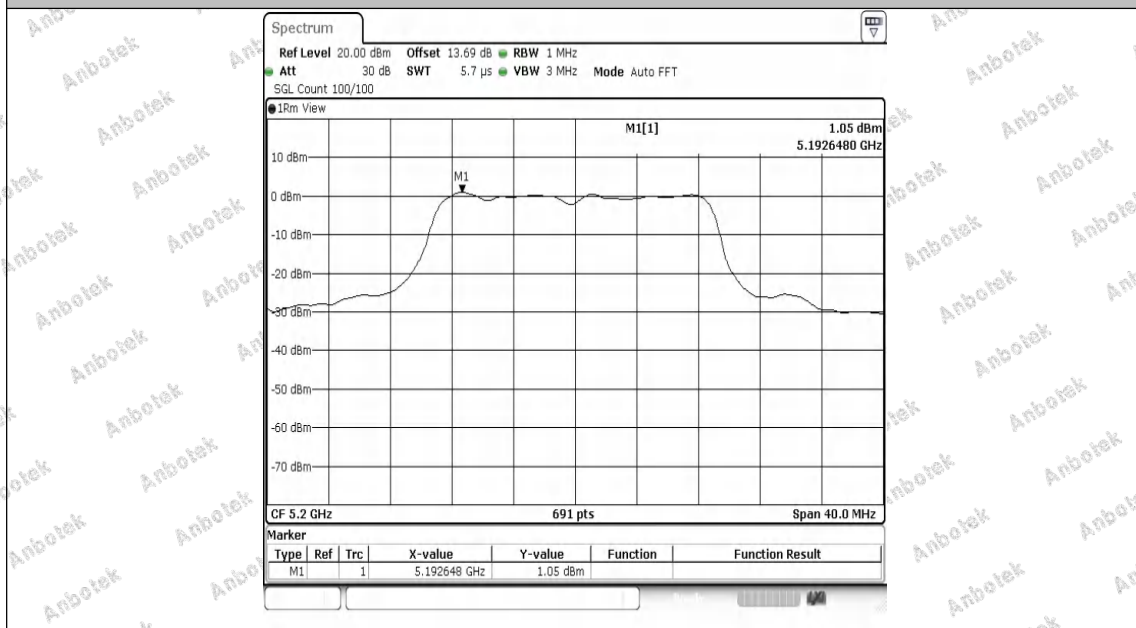
11N20MIMO-Ant2-5200-PASS
