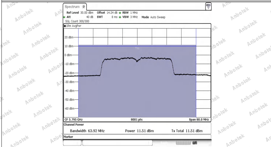
11AX40MIMO-Ant2-5795-PASS
