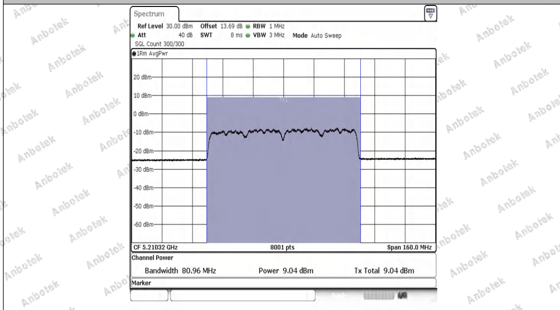
11AX80MIMO-Ant2-5210-PASS
