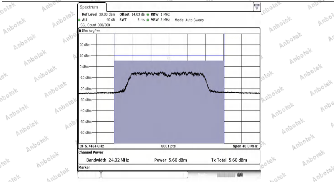
11N20MIMO-Ant1-5745-PASS
