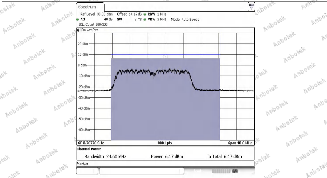
11AC20MIMO-Ant1-5785-PASS
