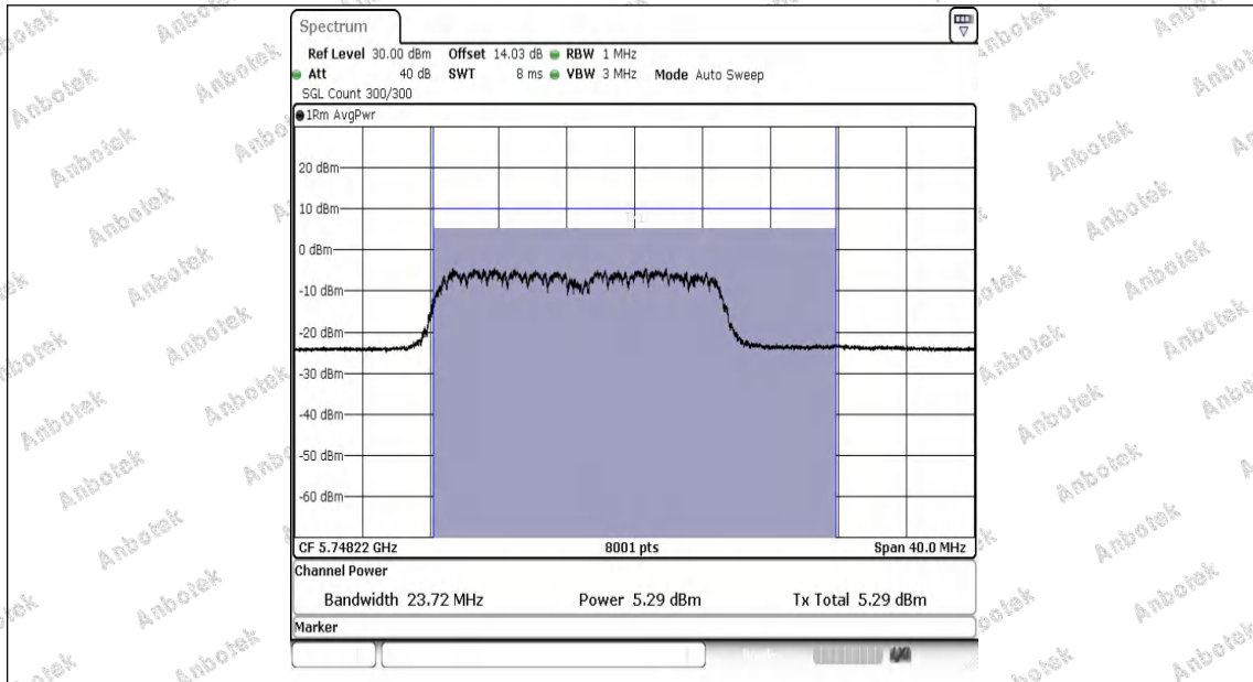
11AC20MIMO-Ant1-5745-PASS
