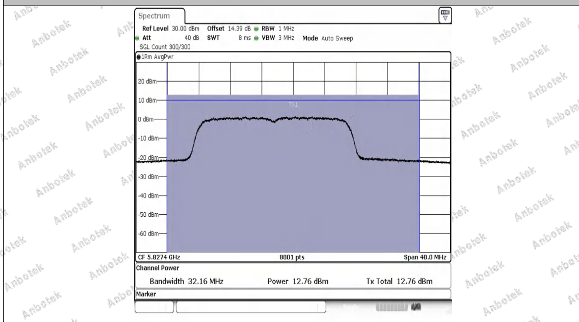
11AX20MIMO-Ant2-5825-PASS
