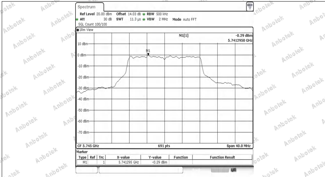
11A-Ant1-5745-PASS
