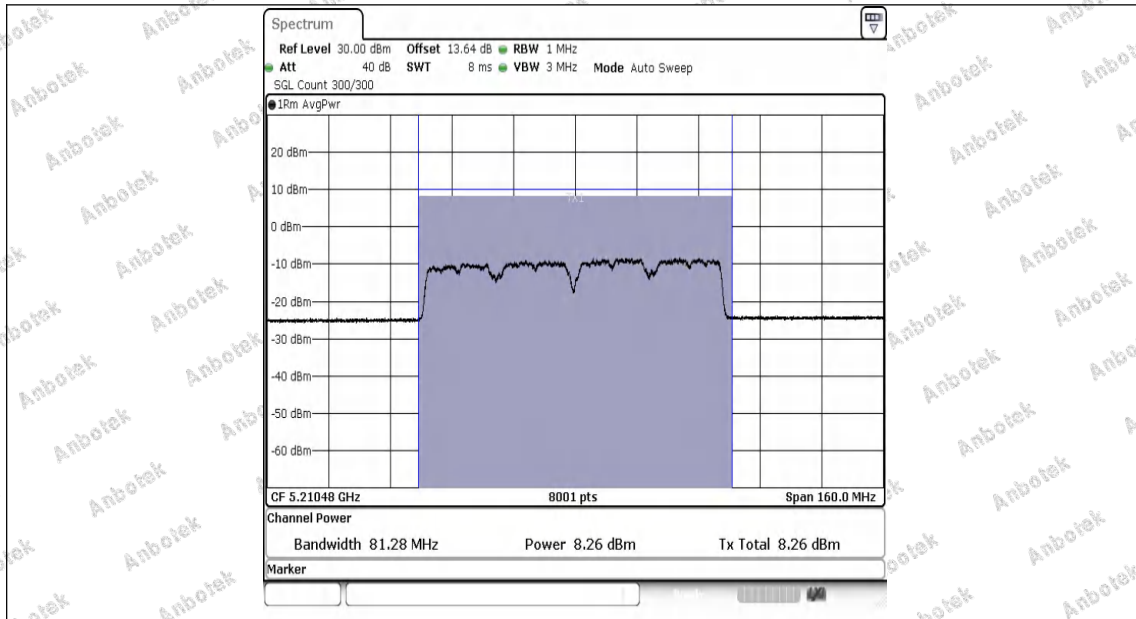
11AC80MIMO-Ant1-5210-PASS
