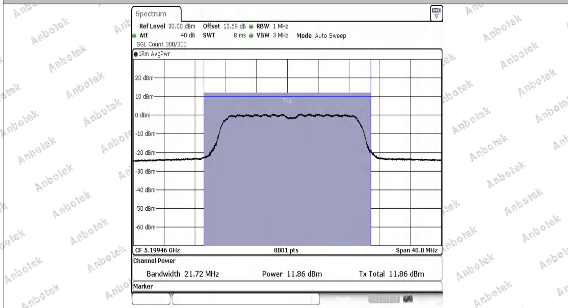
11AC20MIMO-Ant2-5200-PASS
