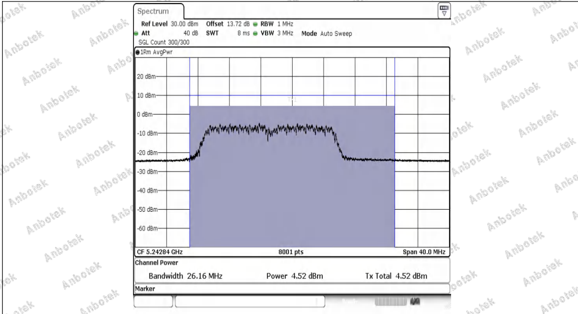
11N20MIMO-Ant1-5240-PASS
