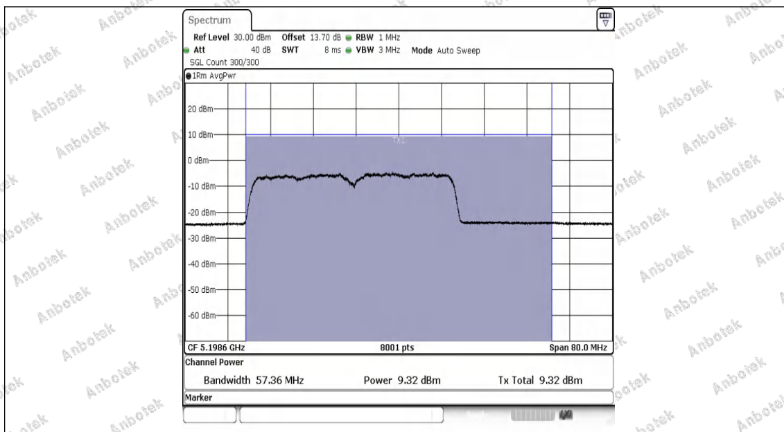
11AX40MIMO-Ant1-5190-PASS
