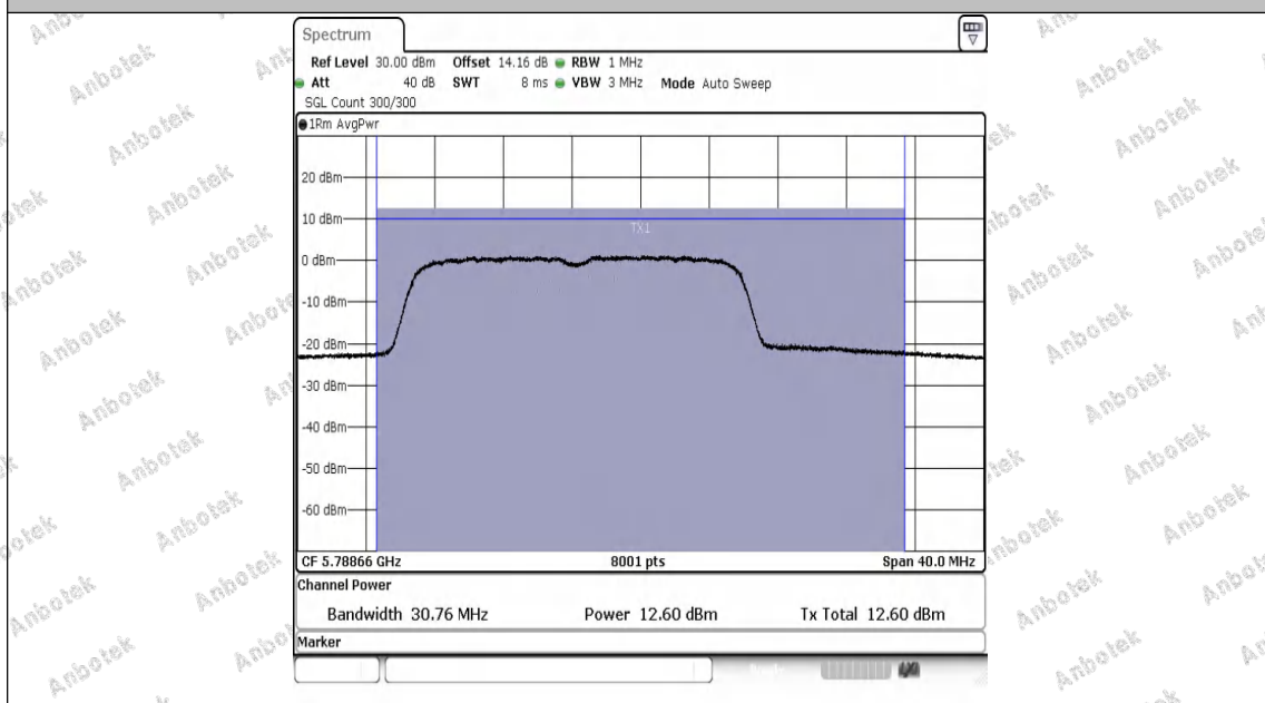
11AX20MIMO-Ant2-5785-PASS
