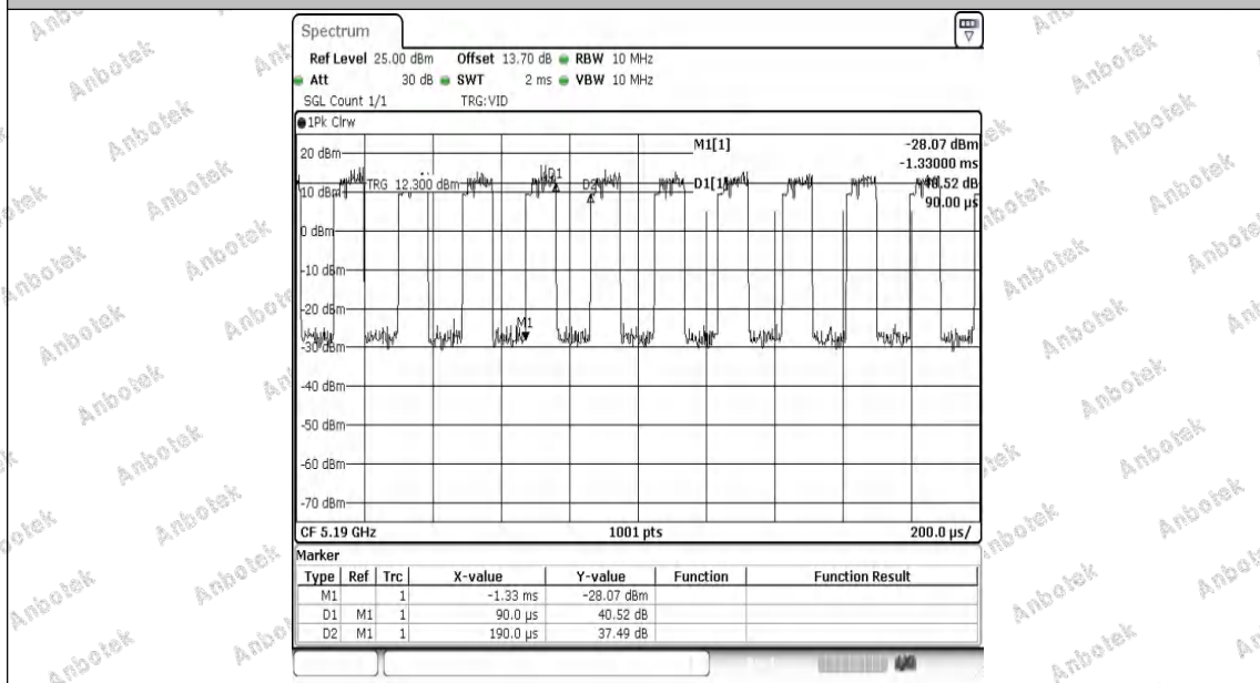
NTNV-11AX40MIMO-Ant2-5190
