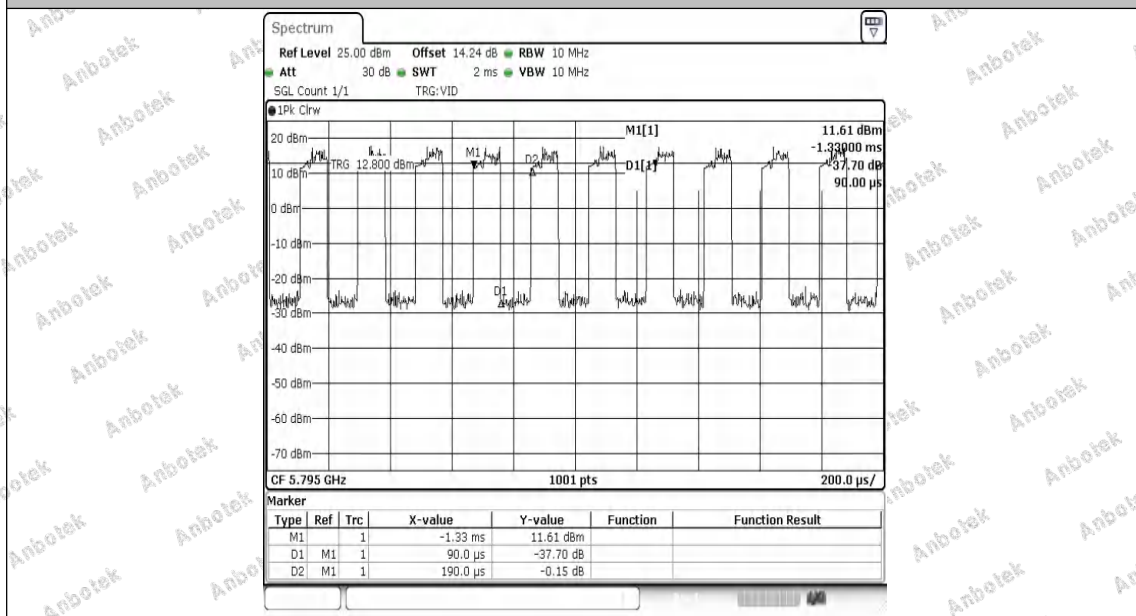
NTNV-11AC40MIMO-Ant2-5795
