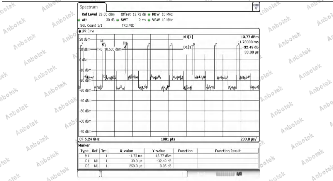
NTNV-11AC20MIMO-Ant1-5240
