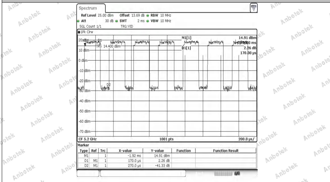
NTVN-11A-Ant2-5200
