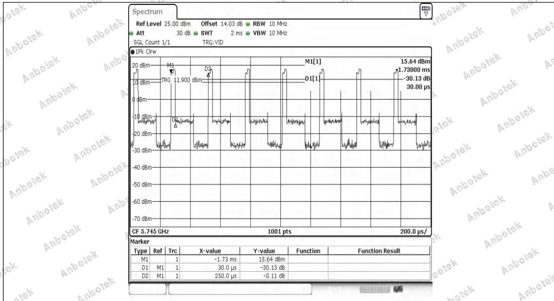
NTNV-11AC20MIMO-Ant1-5745
