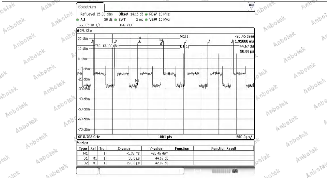
NTVN-11N20MIMO-Ant1-5785
