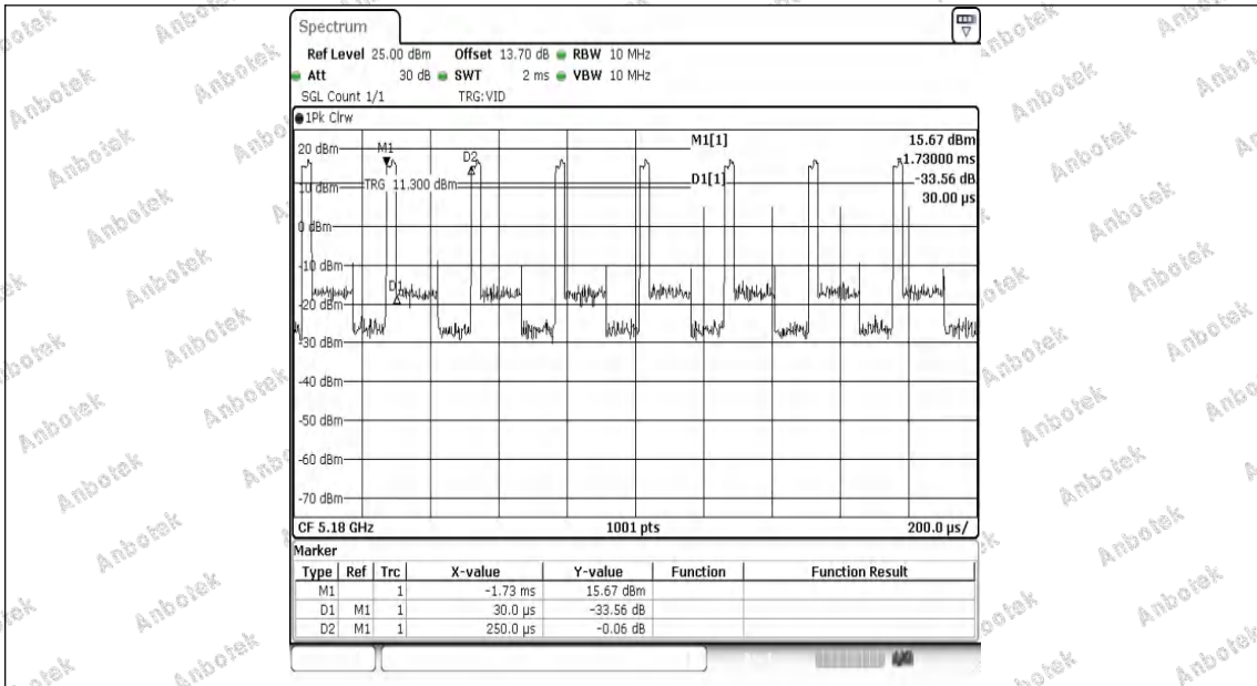
NTNV-11AC20MIMO-Ant1-5180
