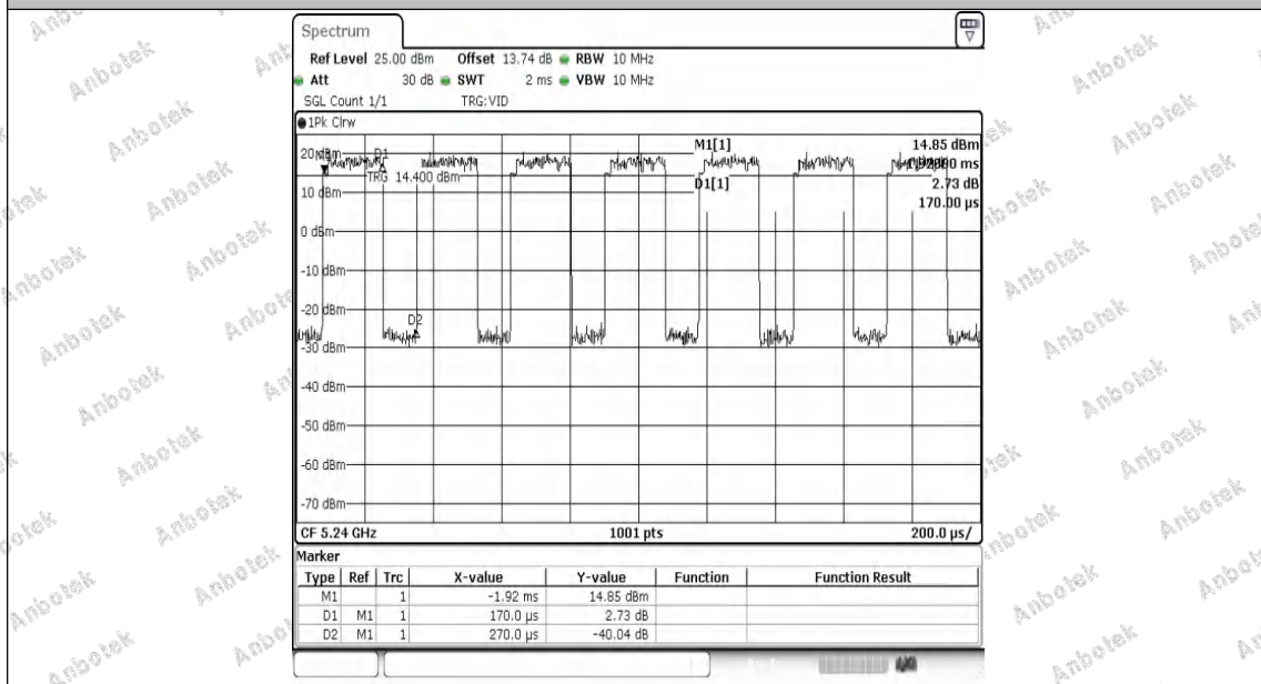
NTV-11A-Ant2-5240
