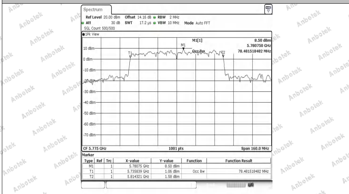
11AX80MIMO-Ant2-5775
