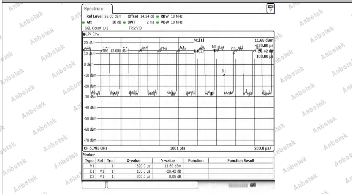
NTNV-11N40MIMO-Ant2-5795
