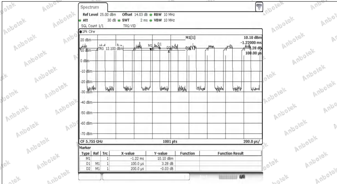
NTVN-11N40MIMO-Ant1-5755
