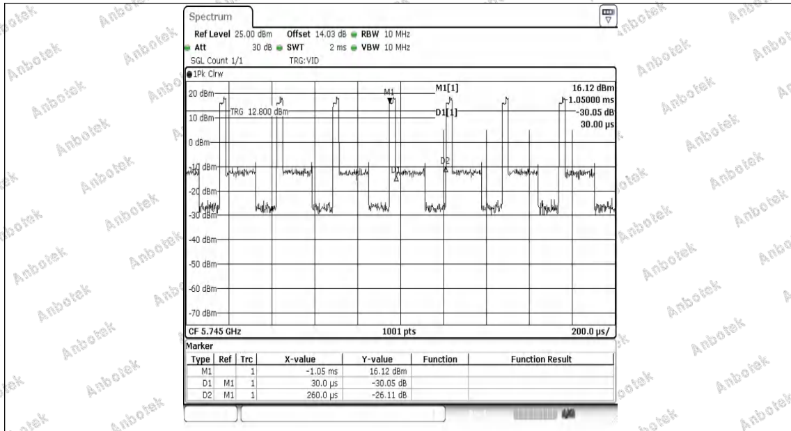
NTVN-11N20MIMO-Ant1-5745
