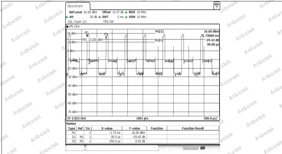
NTNV-11AC20MIMO-Ant1-5825
