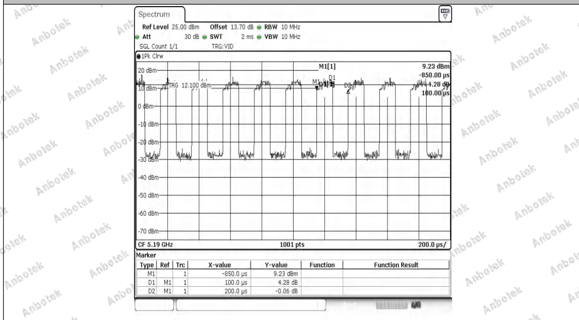
NTVN-11N40MIMO-Ant2-5190
