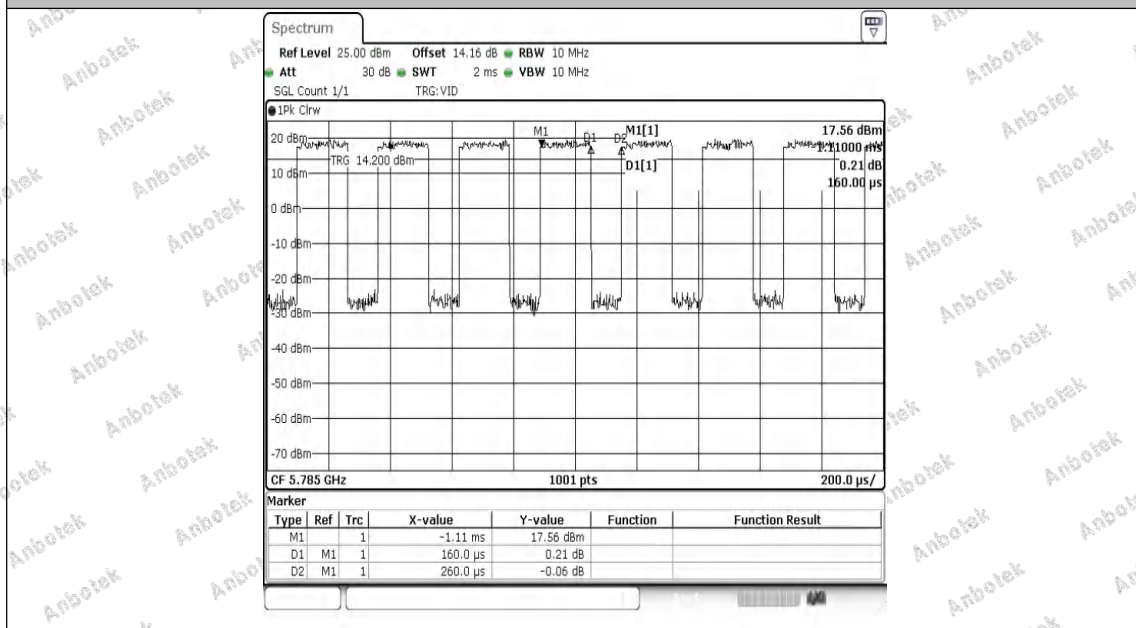
NTVN-11N20MIMO-Ant2-5785
