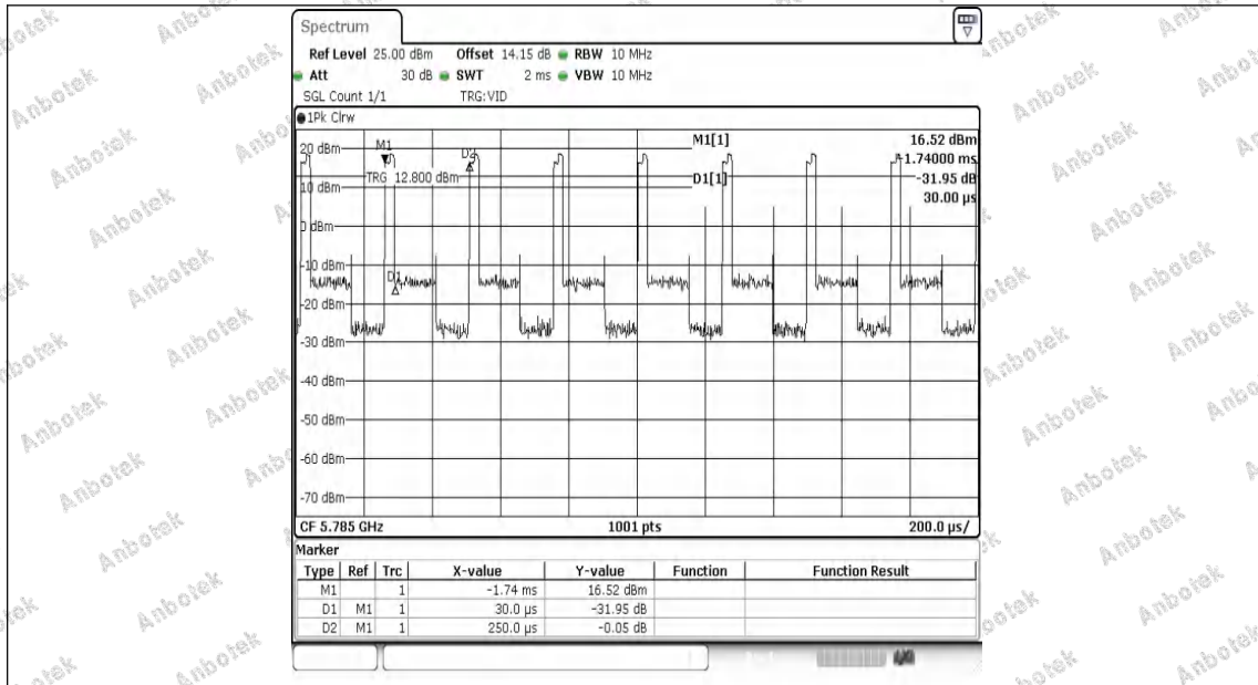
NTNV-11AC20MIMO-Ant1-5785
