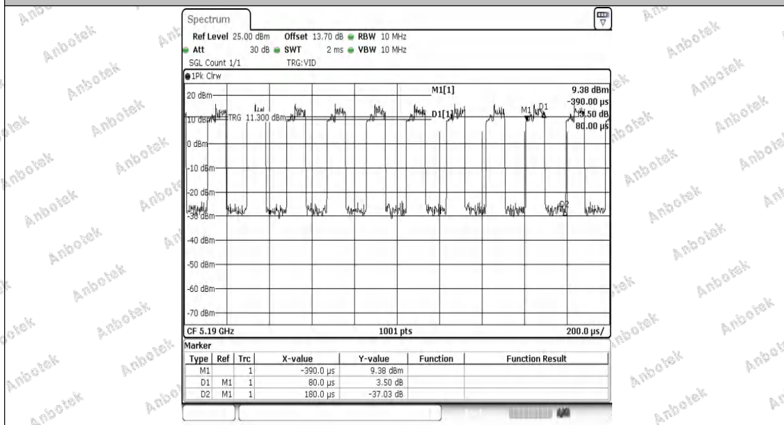
NTNV-11AC40MIMO-Ant2-5190
