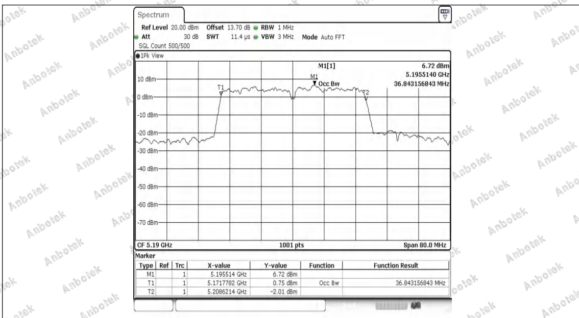
11AC40MIMO-Ant1-5190
