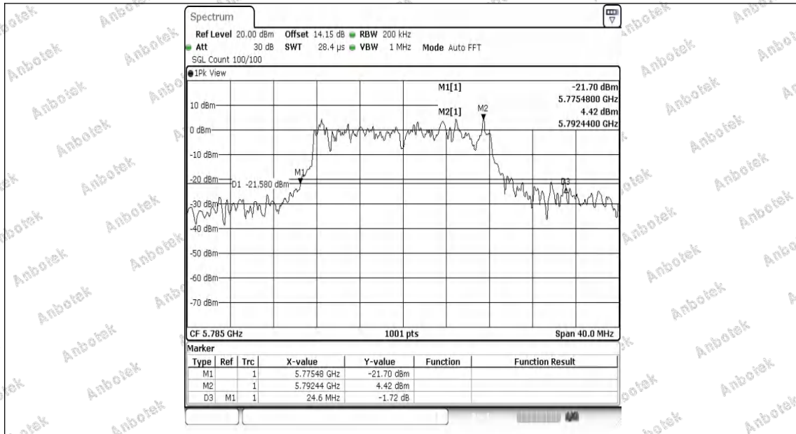
11AC20MIMO-Ant1-5785
