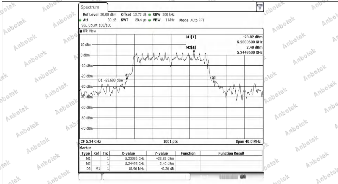
11AC20MIMO-Ant1-5240
