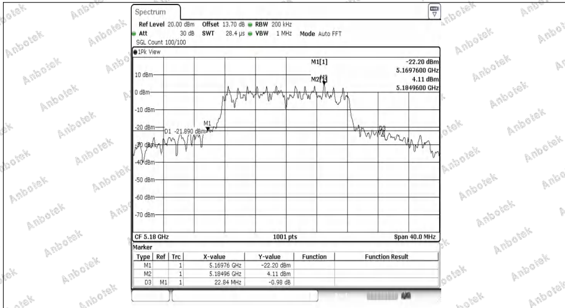
11N20MIMO-Ant1-5180
