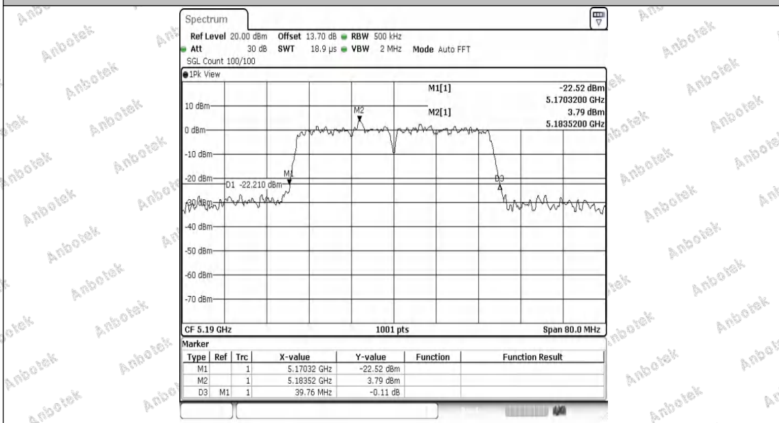
11AC40MIMO-Ant2-5190
