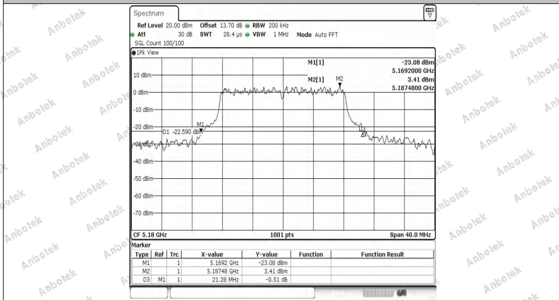
11A-Ant2-5180
