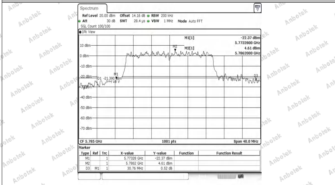
11AX20MIMO-Ant2-5785
