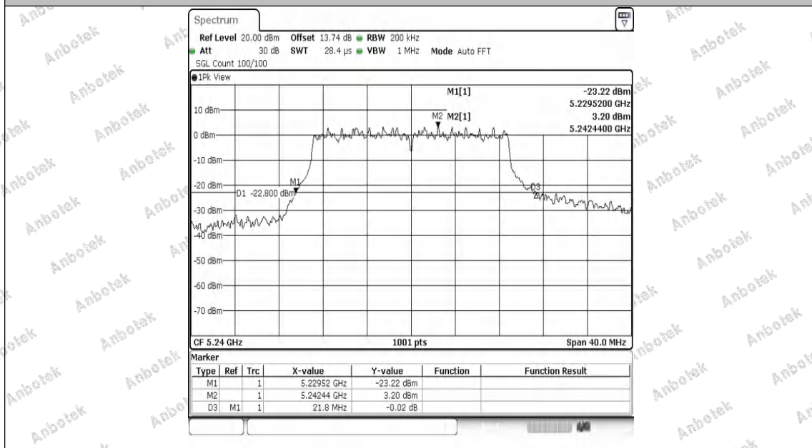
11AC20MIMO-Ant2-5240
