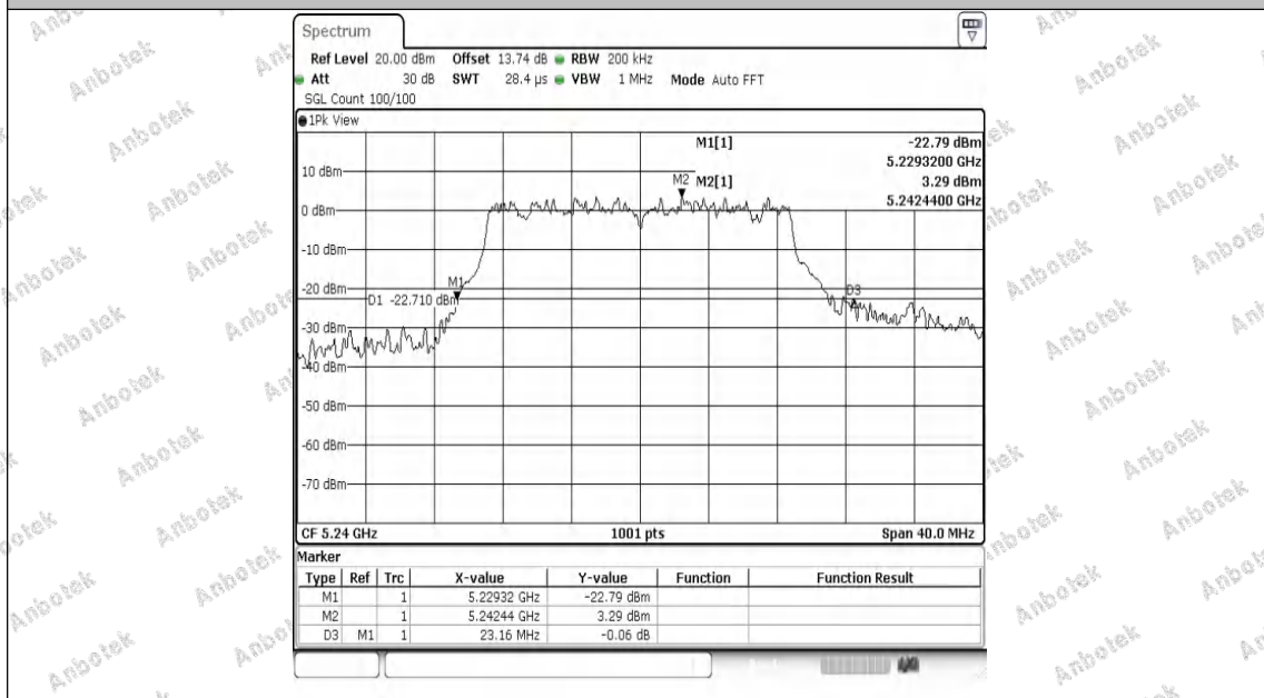
11N20MIMO-Ant2-5240
