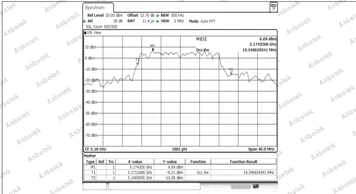
11AC20MIMO-Ant1-5180
