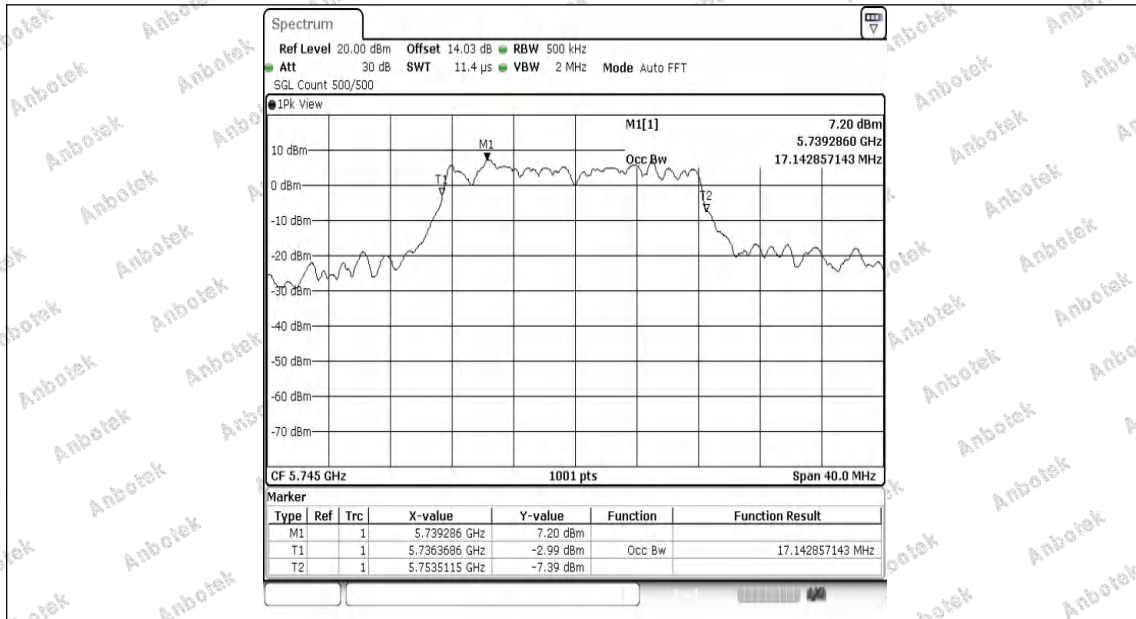
11AC20MIMO-Ant1-5745
