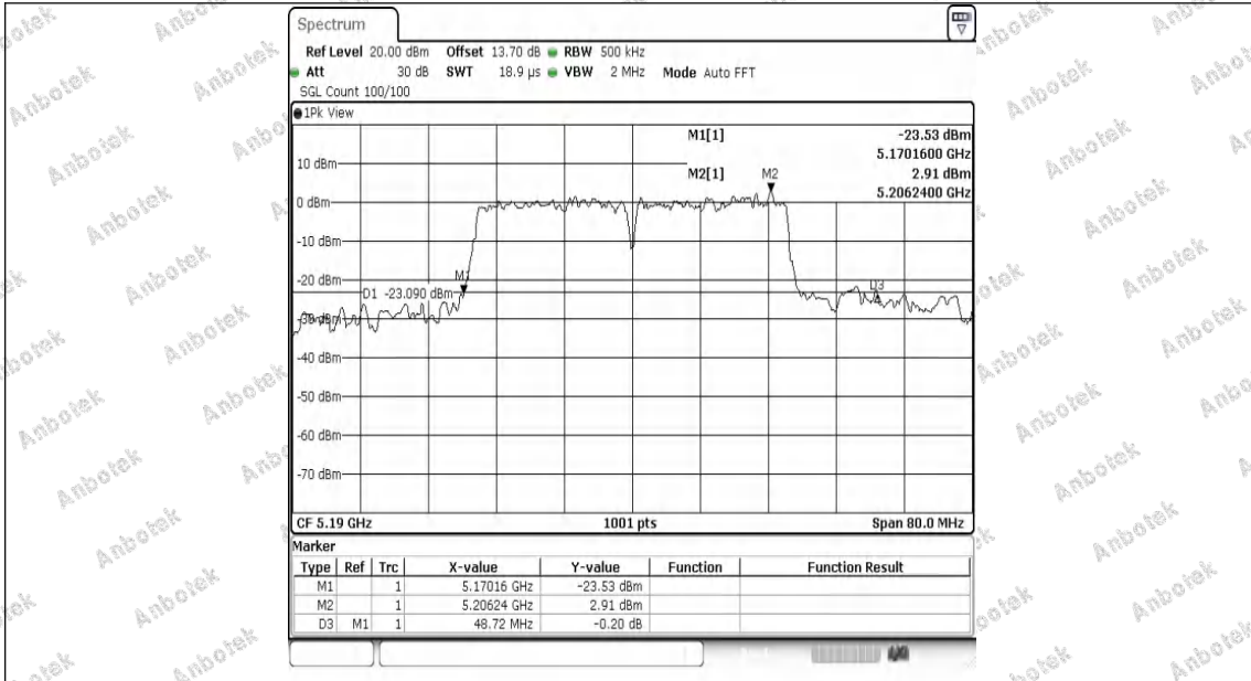
11AC40MIMO-Ant1-5190
