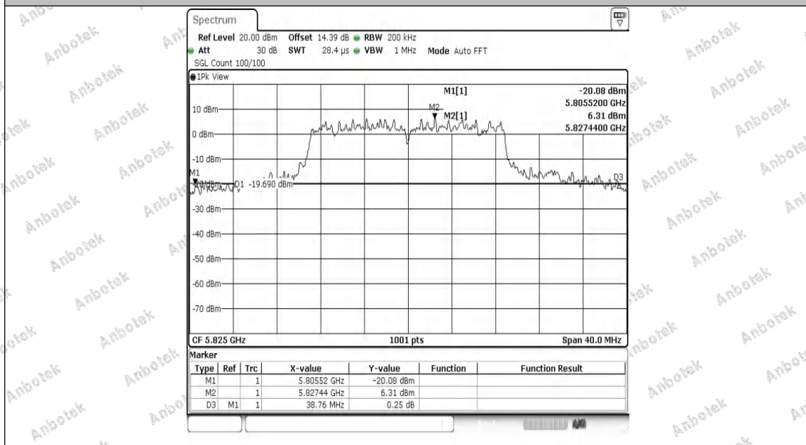
11N20MIMO-Ant2-5825
