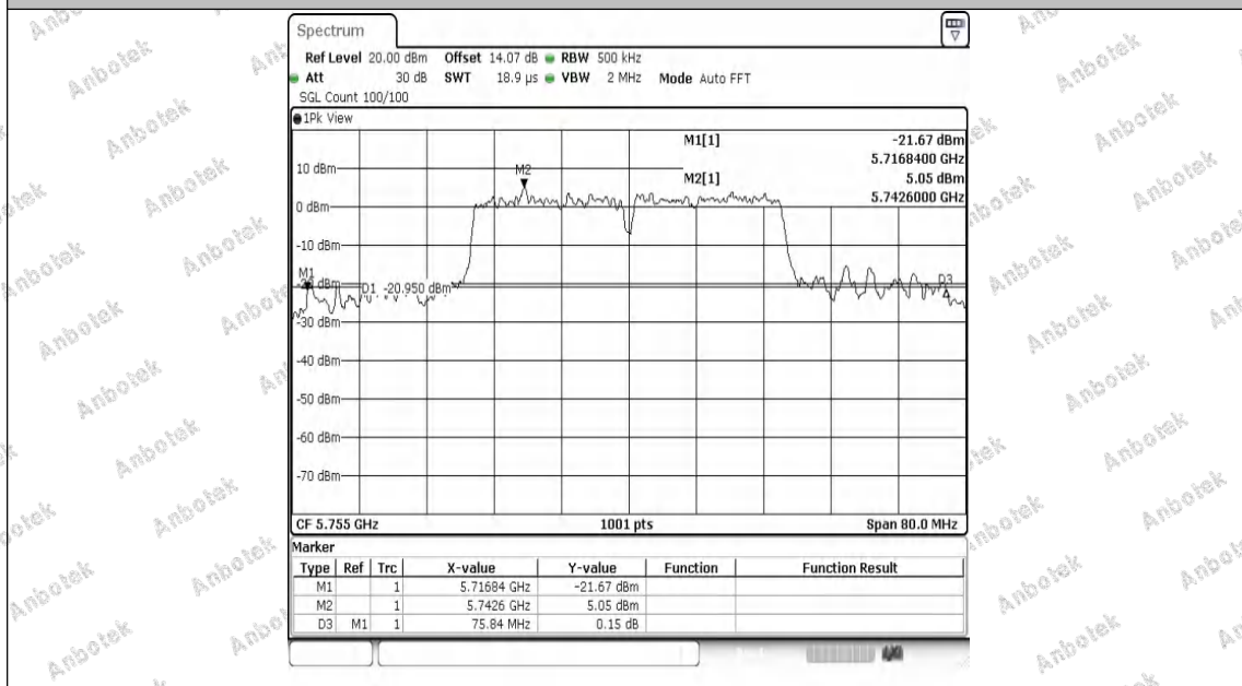
11N40MIMO-Ant2-5755
