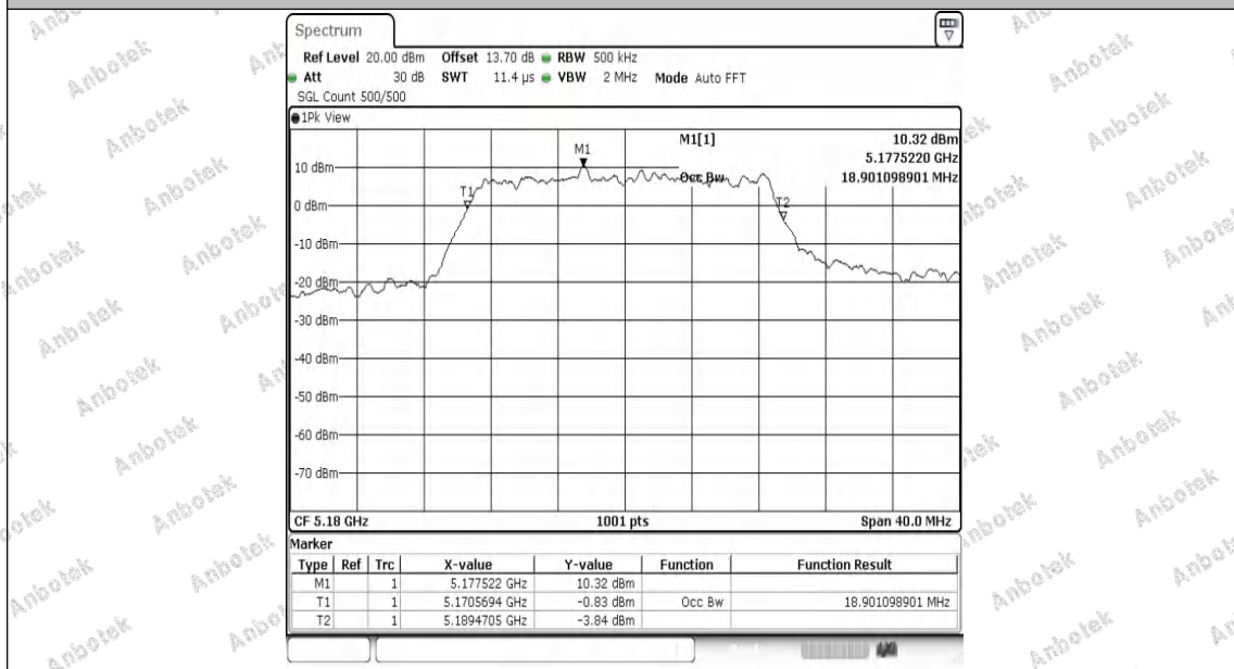
11AC20MIMO-Ant2-5180
