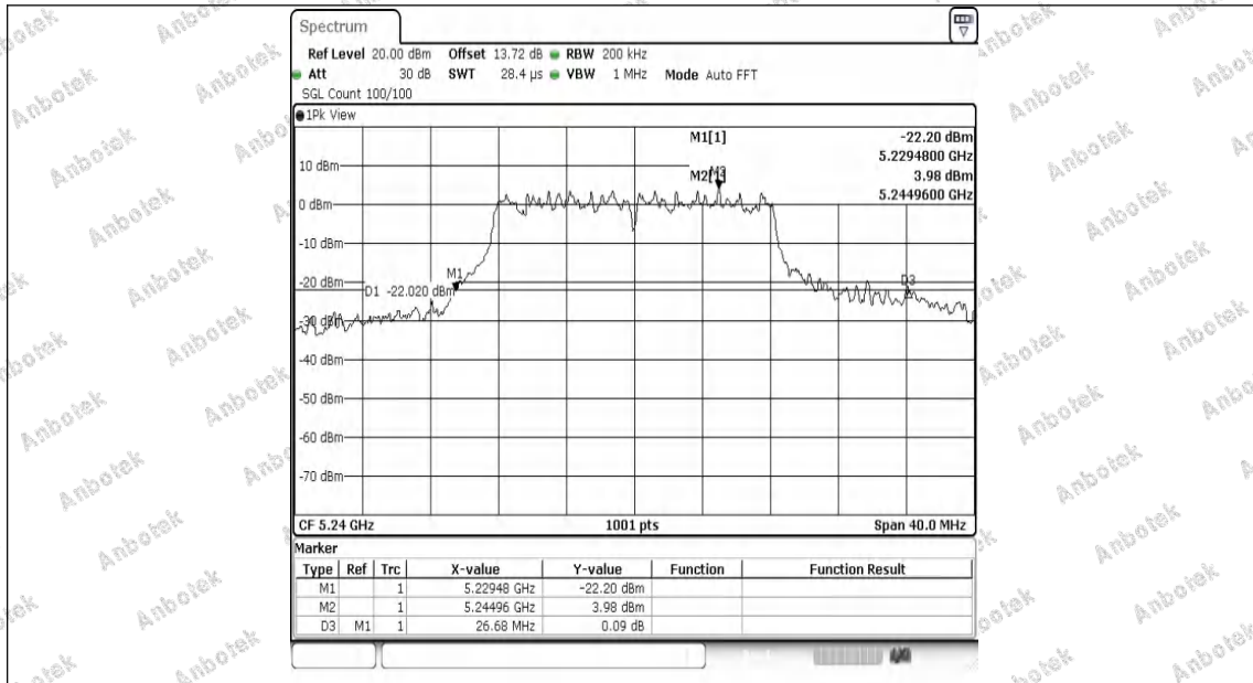
11A-Ant1-5240
