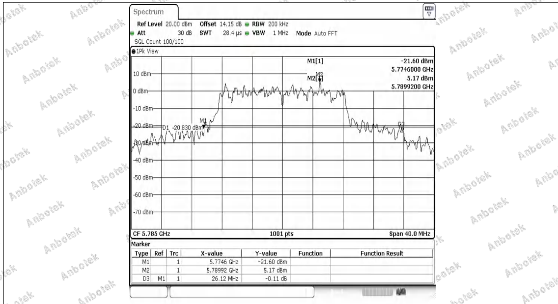
11N20MIMO-Ant1-5785
