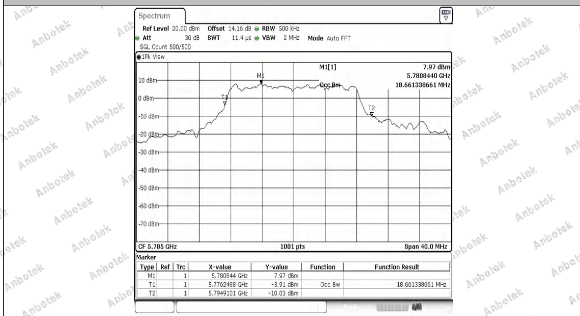
11A-Ant2-5785
