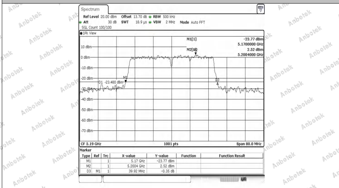
11N40MIMO-Ant2-5190
