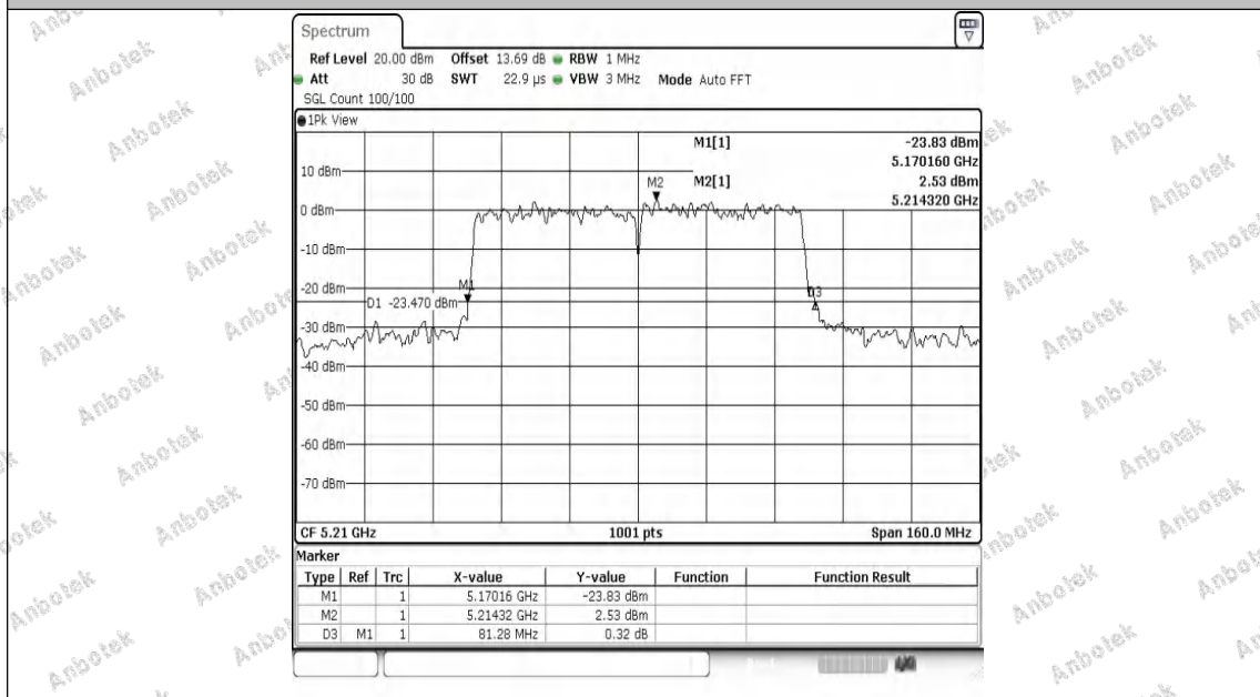
11AC80MIMO-Ant2-5210
