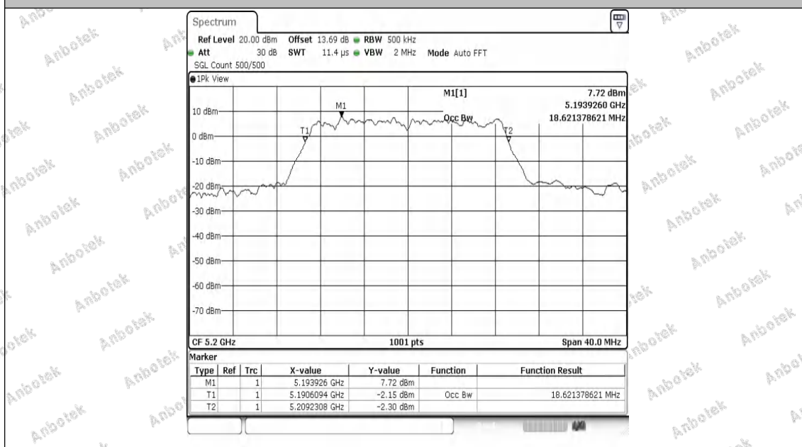
11AC20MIMO-Ant2-5200
