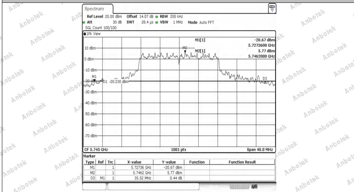
11A-Ant2-5745
