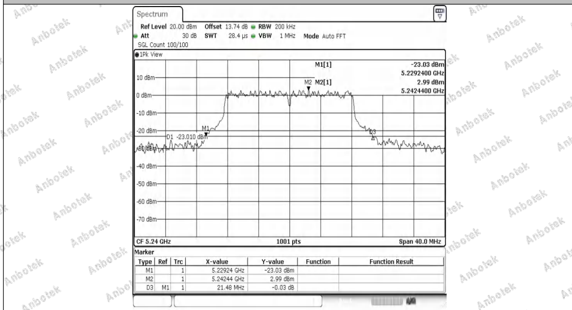
11A-Ant2-5240
