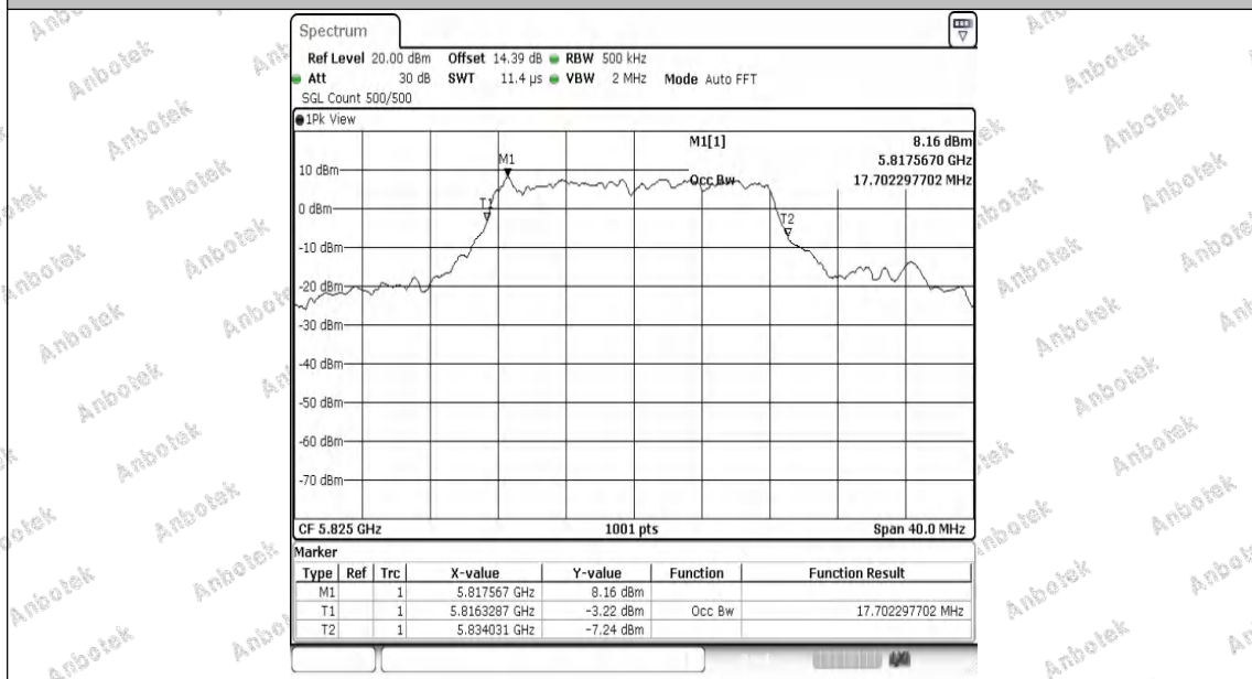
11A-Ant2-5825
