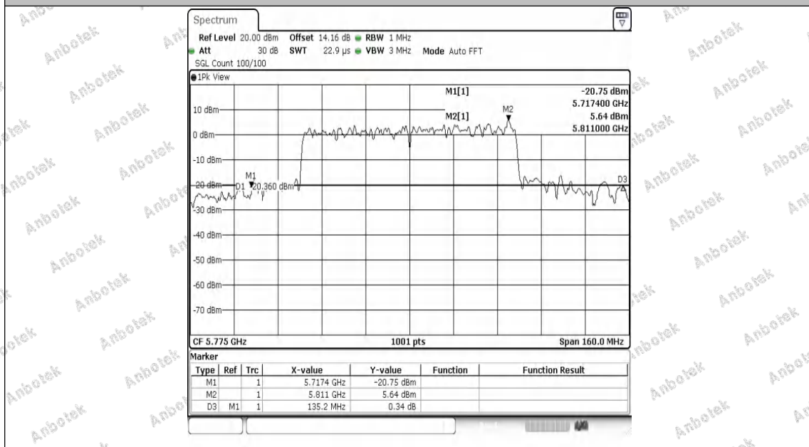
11AX80MIMO-Ant2-5775
