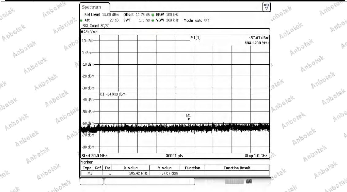
11AX20MIMO-Ant1-2437-30~1000-PASS
