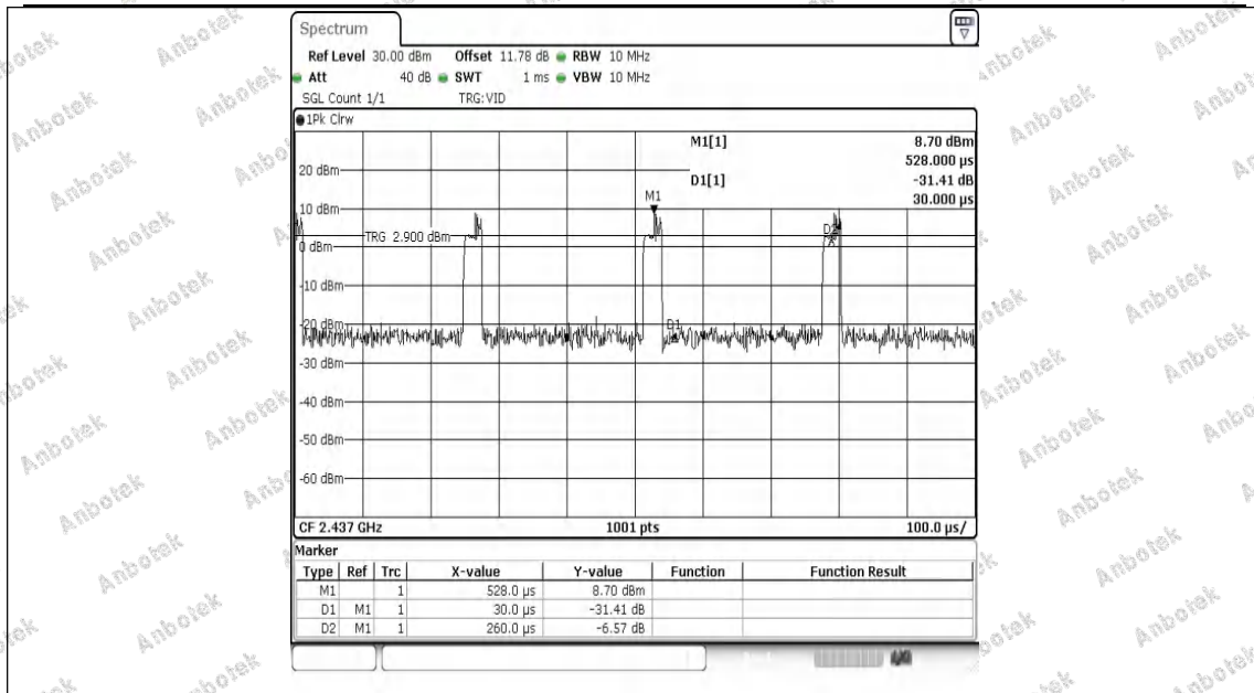
NTVN-11N20MIMO-Ant1-2437
