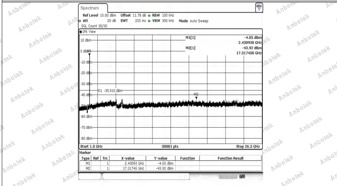
11N20MIMO-Ant2-2437-1000~26500-PASS
