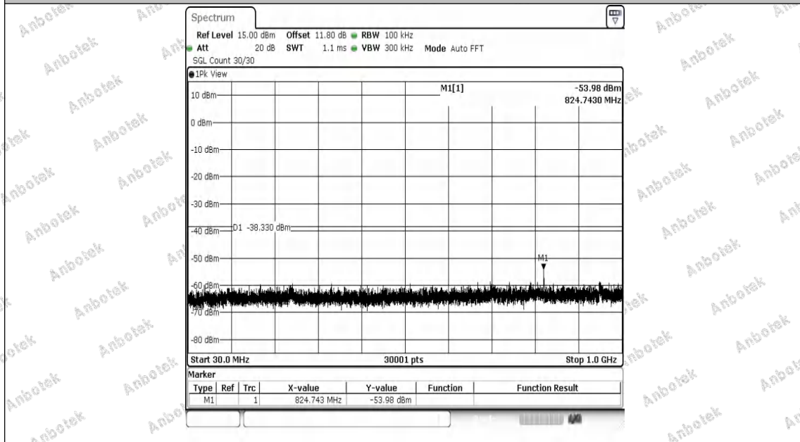
11AX20MIMO-Ant2-2412-30~1000-PASS
