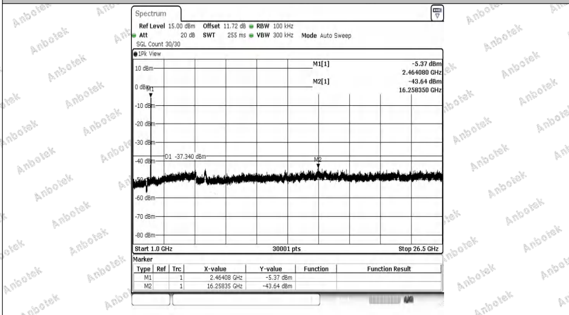
11AX20MIMO-Ant2-2462-1000~26500-PASS
