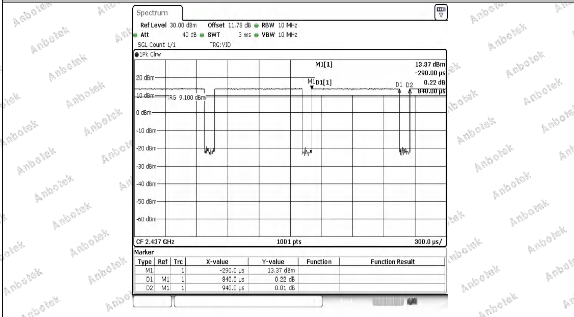
NTNV-11B-Ant2-2437
