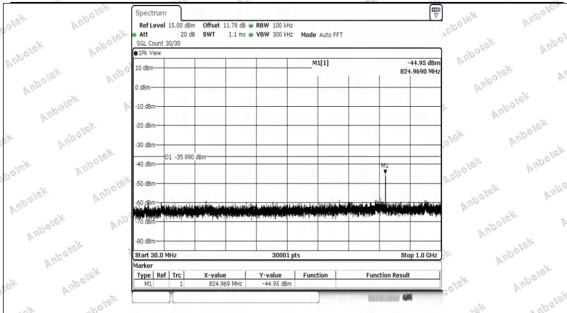
11AX20MIMO-Ant1-2412-30~1000-PASS
