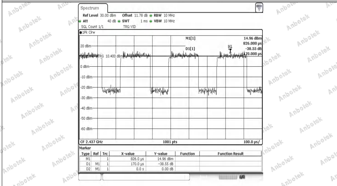
NTVN-11N20MIMO-Ant2-2437
