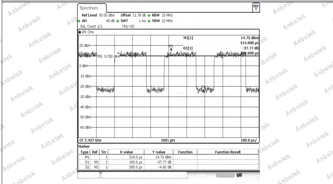
NTN-11G-Ant2-2437
