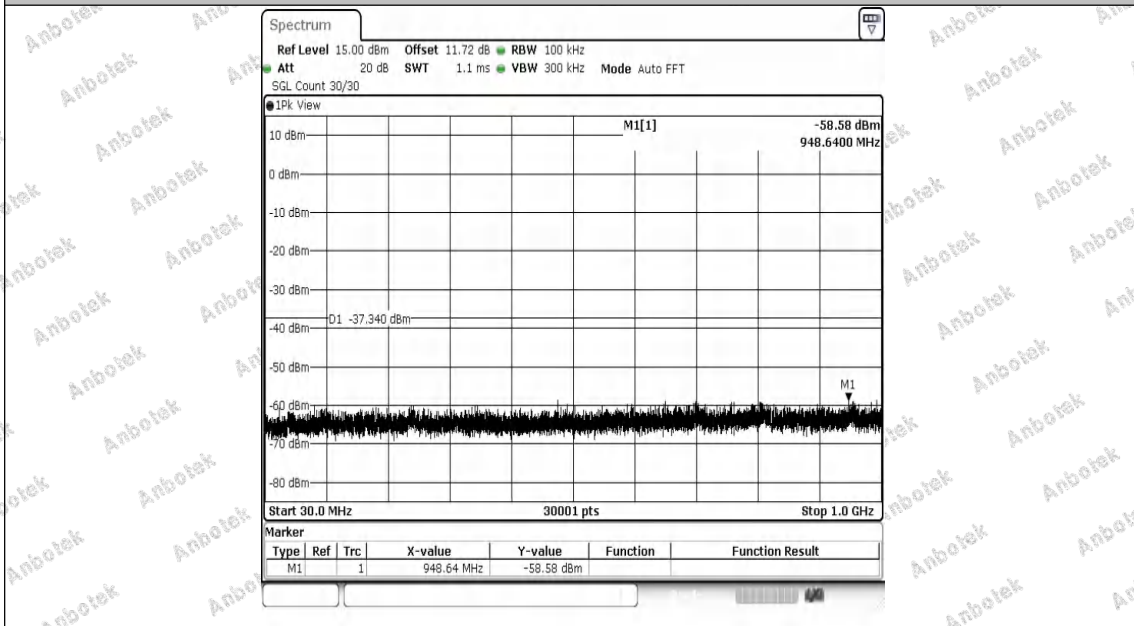
11AX20MIMO-Ant2-2462-30~1000-PASS
