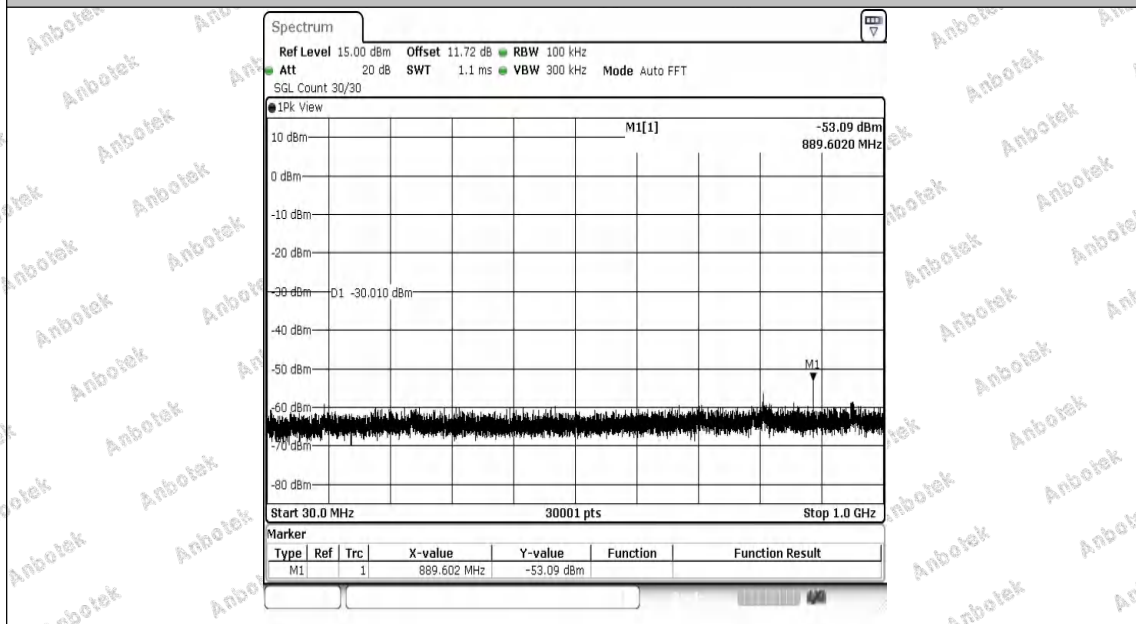
11B-Ant2-2462-30~1000-PASS
