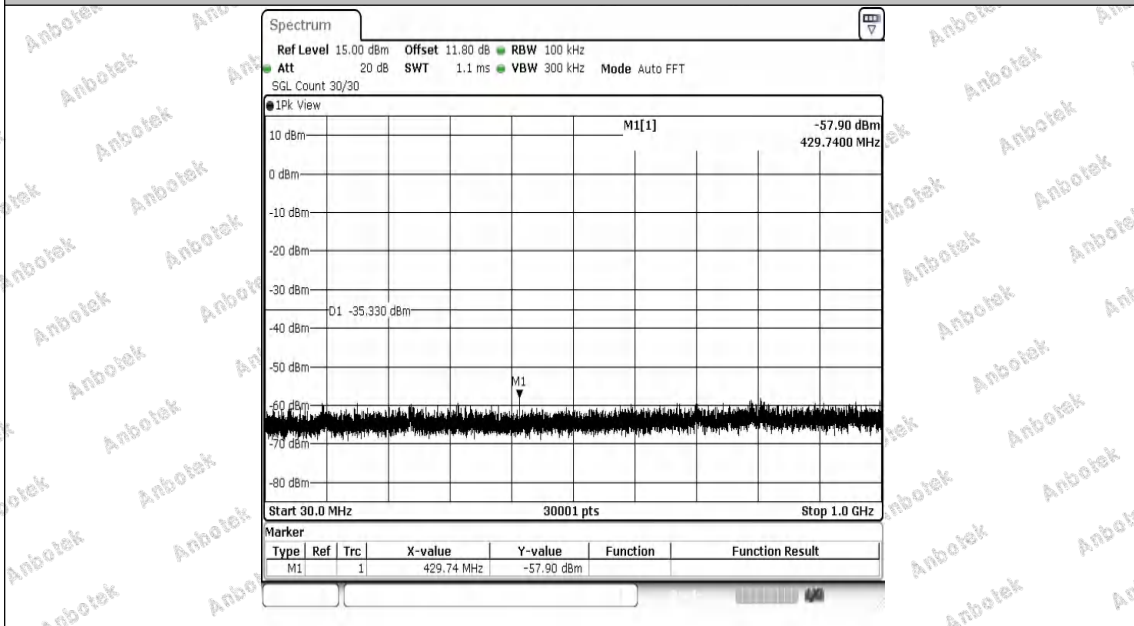
11N20MIMO-Ant2-2412-30~1000-PASS
