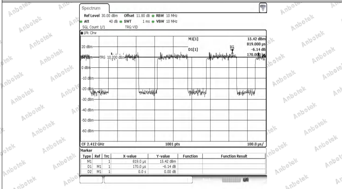
NTVN-11N20MIMO-Ant2-2412
