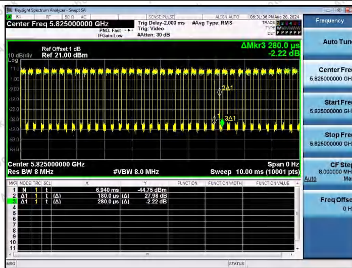
NTNV-11A-Ant1-5825
