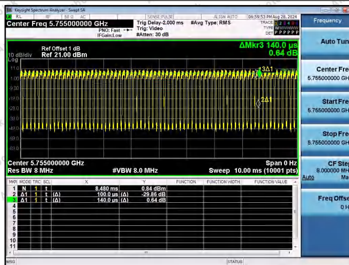
NTNV-11N40SISO-Ant1-5755
