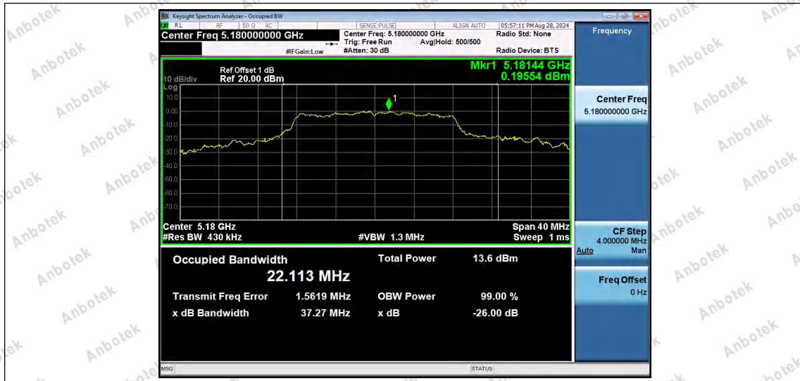
11A-Ant1-5180
