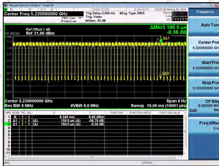
NTNV-11AC20SISO-Ant1-5220
