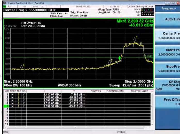
11AX20SISO-Ant1-2412-PASS
