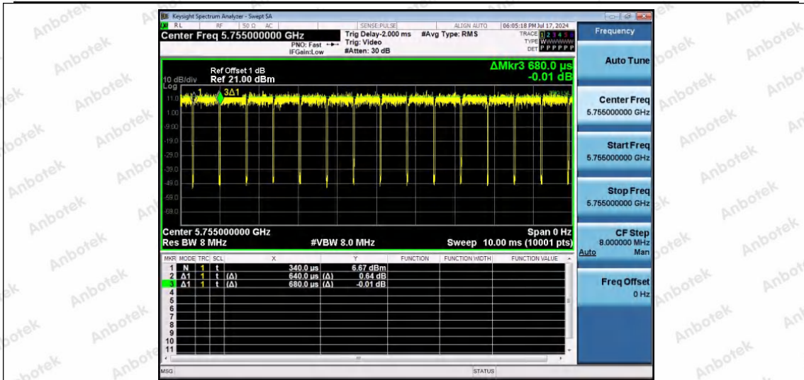
NTNV-11N40SISO-Ant1-5755
