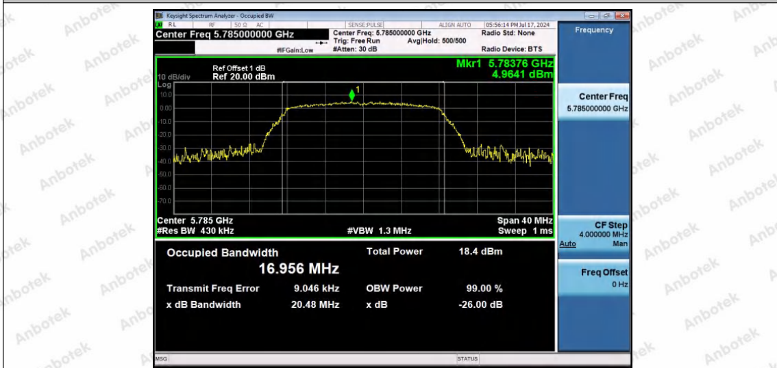
11A-Ant1-5785
