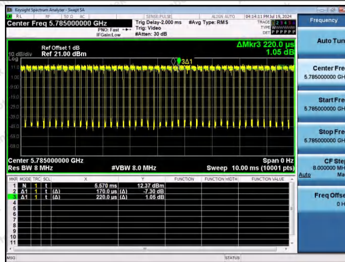
NTV-11AX20SISO-Ant1-5785
