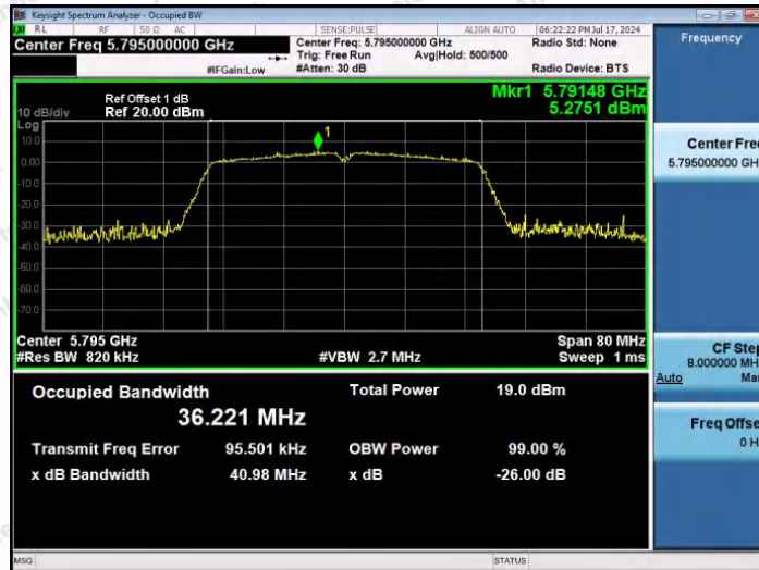
11AC40SISO-Ant1-5795
