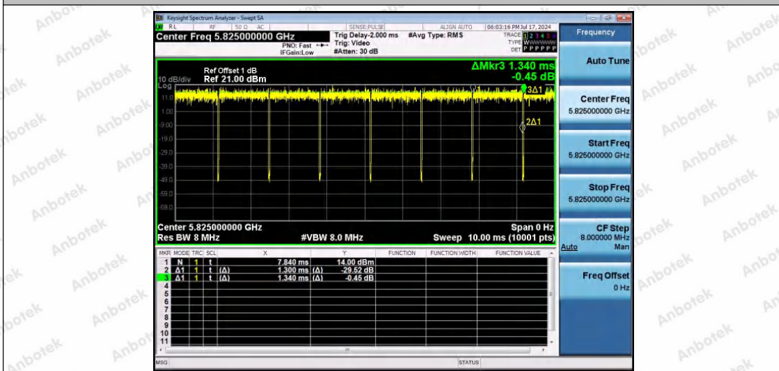
NTNV-11N20SISO-Ant1-5825
