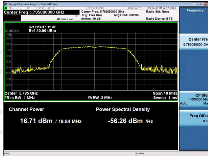
11A-Ant1-5785-PASS
