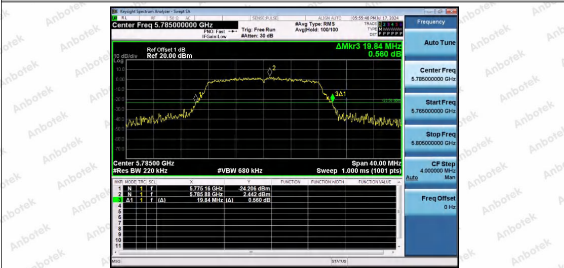
11A-Ant1-5785
