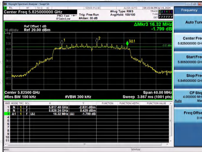
11AX20ISO-Ant1-5825-PASS
