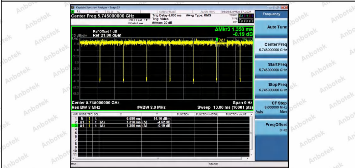
NTNV-11AC20SISO-Ant1-5745
