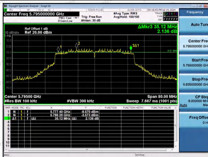
11AX40ISO-Ant1-5795-PASS
