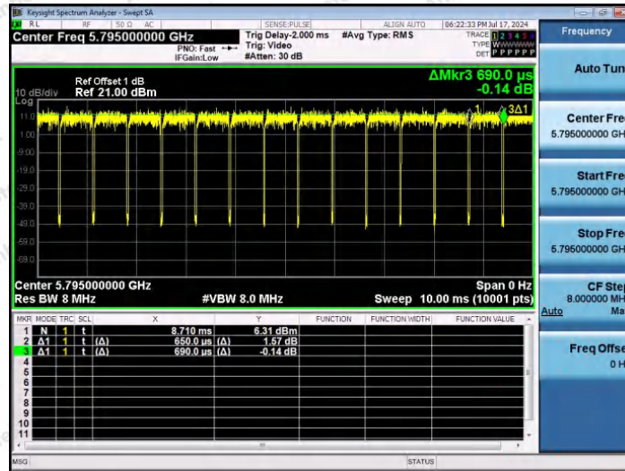
NTV-11AC40SISO-Ant1-5795
