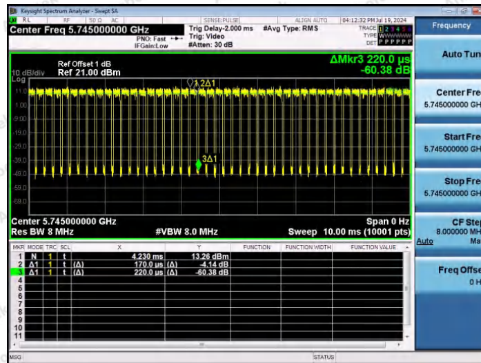
NTV-11AX20SISO-Ant1-5745
