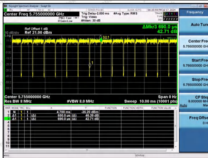
NTVN-11AC40SISO-Ant1-5755
