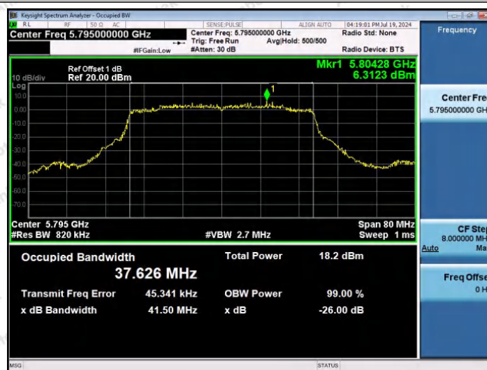
11AX40SISO-Ant1-5795
