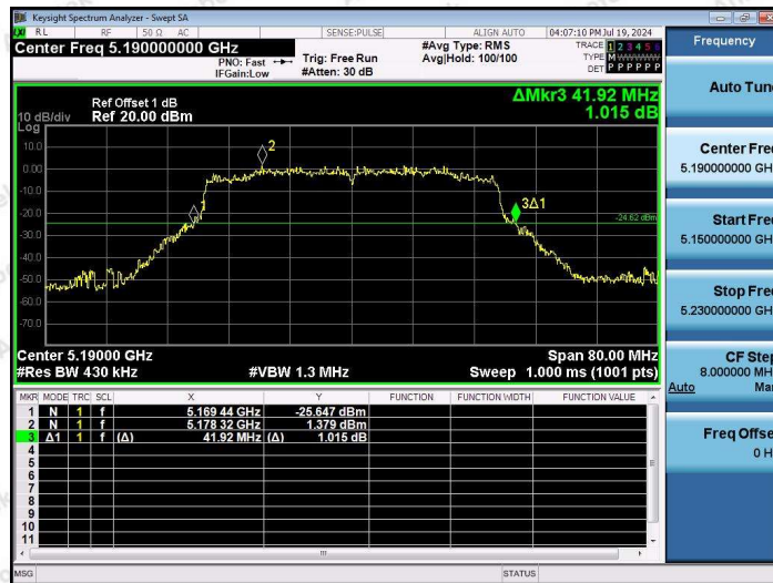
11AX40SISO-Ant1-5190
