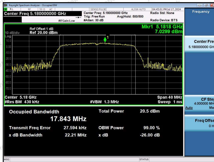
11A20SISO-Ant1-5180
