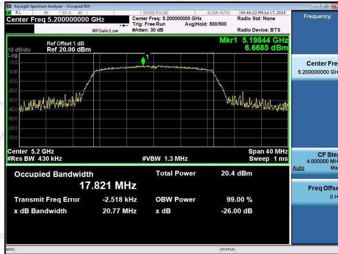
11AC20SISO-Ant1-5200
