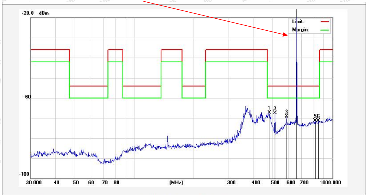
Fundamental signal
