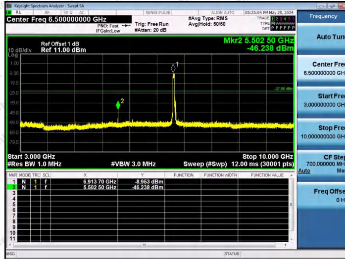
11AX80SISO-Ant1-6945-484Tone-RU65-3000~10000-PASS
