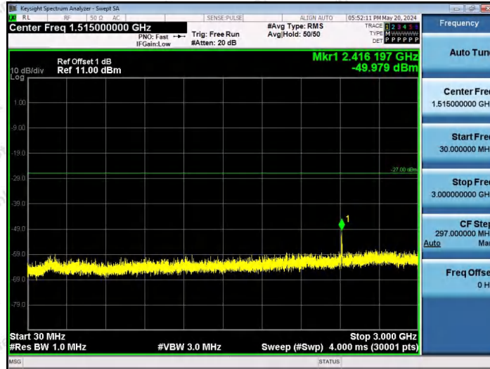
11AX80SISO-Ant1-7025-484Tone-RU66-30~3000-PASS
