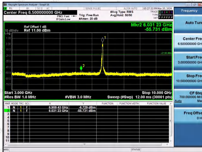
11AX80SISO-Ant1-6945-484Tone-RU66-3000~10000-PASS
