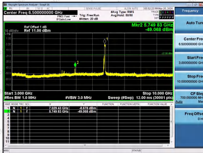
11AX80SISO-Ant1-7025-484Tone-RU66-3000~10000-PASS
