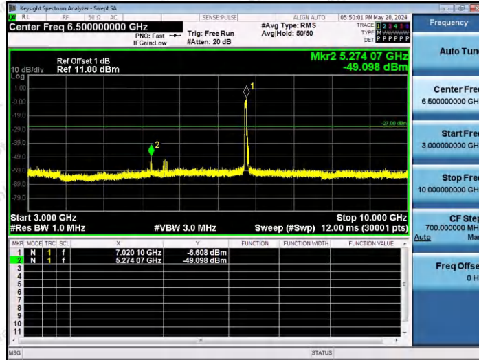
11AX80SISO-Ant1-7025-484Tone-RU65-3000~10000-PASS
