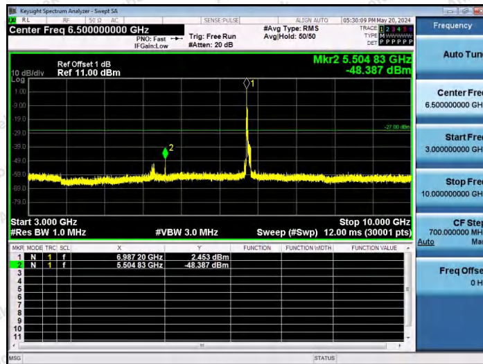
11AX80SISO-Ant1-7025-26Tone-RU0-3000~10000-PASS
