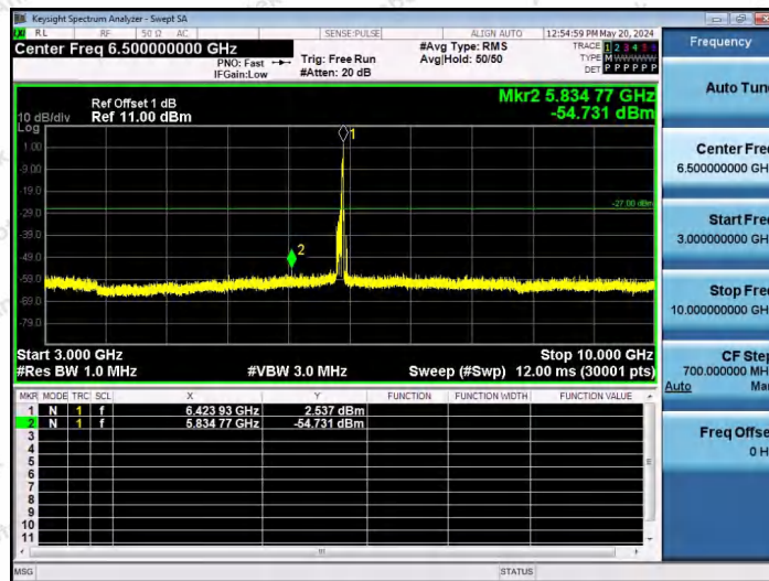
11AX80SISO-Ant1-6385-26Tone-RU36-3000~10000-PASS
