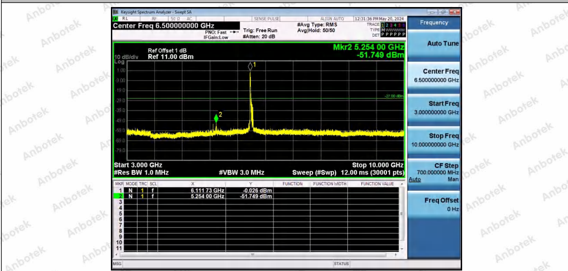
11AX80SISO-Ant1-6145-106Tone-RU53-3000~10000-PASS
