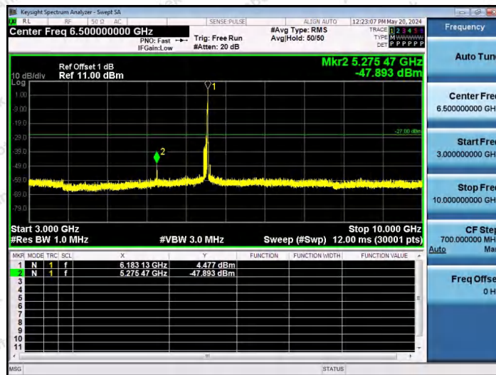
11AX80SISO-Ant1-6145-26Tone-RU36-3000~10000-PASS
