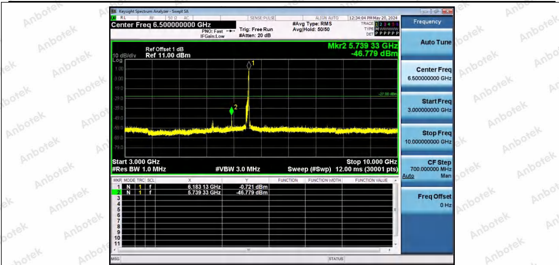
11AX80SISO-Ant1-6145-106Tone-RU60-3000~10000-PASS
