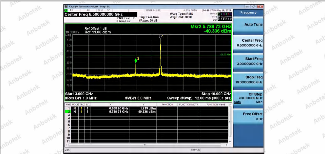
11AX40SISO-Ant1-6885-52Tone-RU37-3000~10000-PASS
