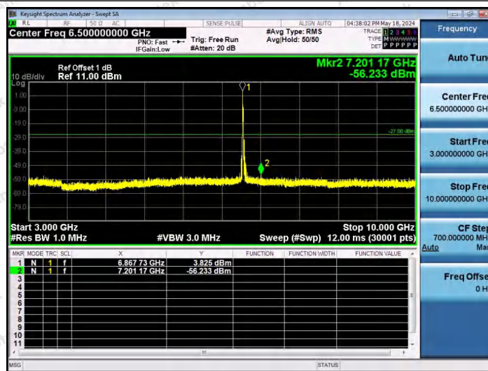
11AX40SISO-Ant1-6885-26Tone-RU0-3000~10000-PASS
