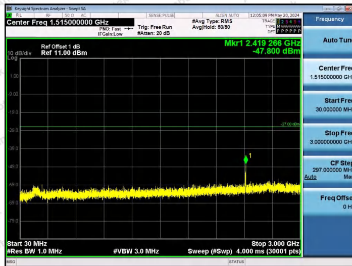
11AX80SISO-Ant1-5985-106Tone-RU60-30~3000-PASS
