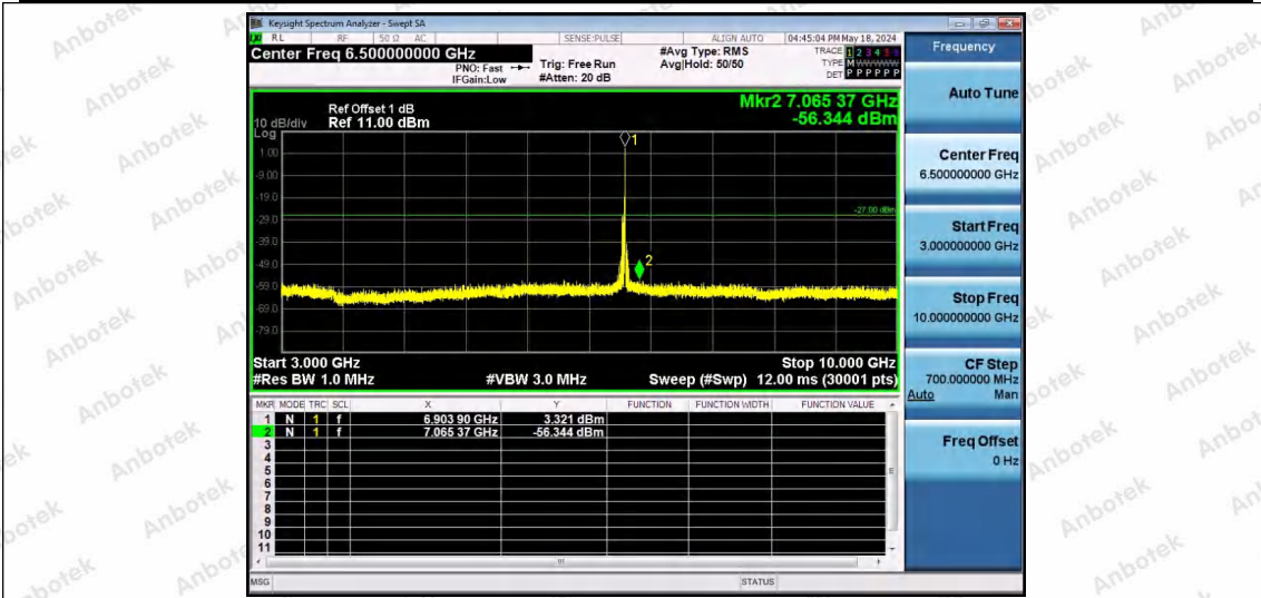
11AX40SISO-Ant1-6885-26Tone-RU17-3000~10000-PASS
