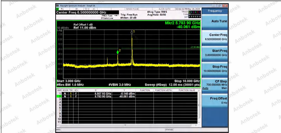
11AX40SISO-Ant1-6525-52Tone-RU37-3000~10000-PASS
