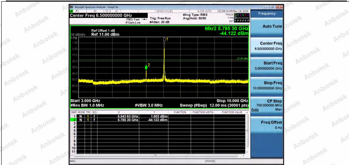
11AX40SISO-Ant1-6525-26Tone-RU17-3000~10000-PASS
