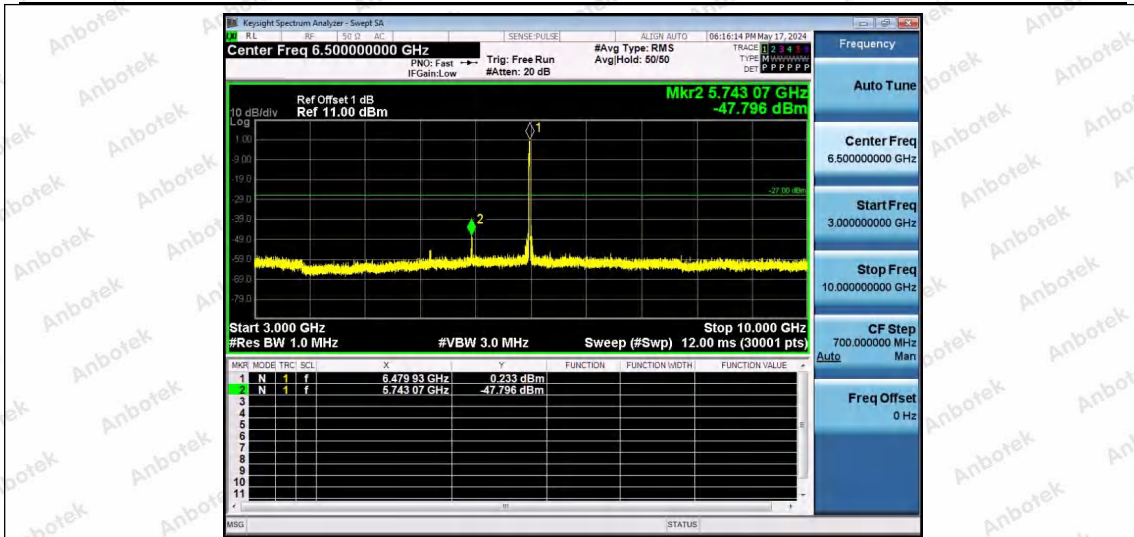
11AX20SISO-Ant1-6475-52Tone-RU39-3000~10000-PASS
