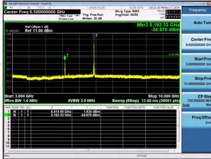
11AX20SISO-Ant1-6415-26Tone-RU4-3000~10000-PASS
