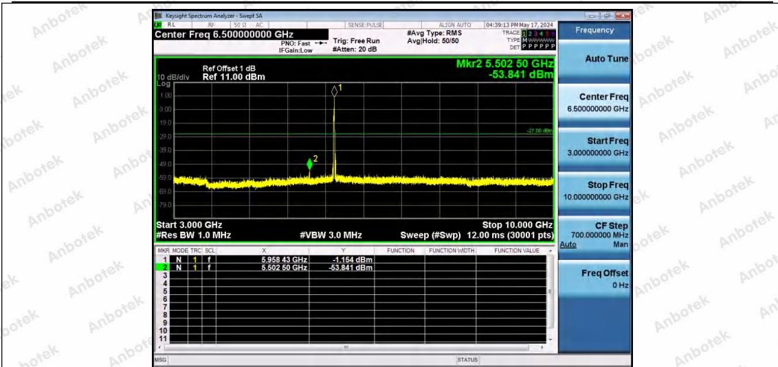
11AX20SISO-Ant1-5955-52Tone-RU39-3000~10000-PASS
