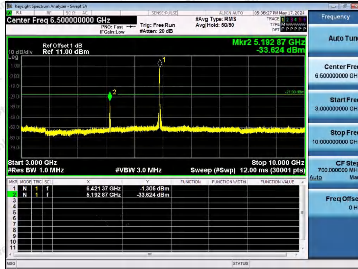
11AX20SISO-Ant1-6415-106Tone-RU54-3000~10000-PASS
