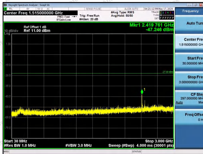
11AX20SISO-Ant1-5955-26Tone-RU0-30~3000-PASS
