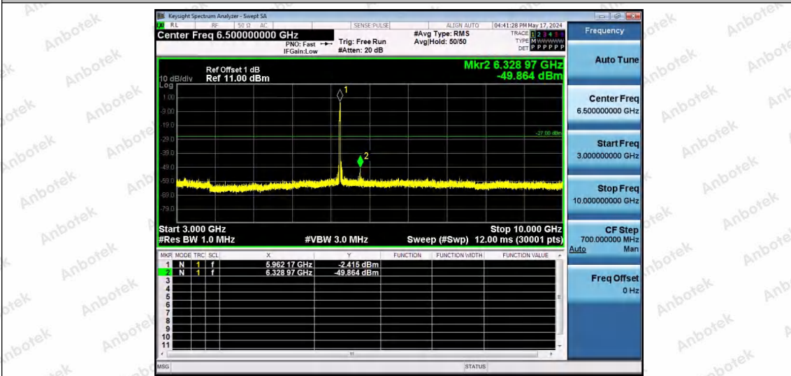
11AX20SISO-Ant1-5955-52Tone-RU40-3000~10000-PASS
