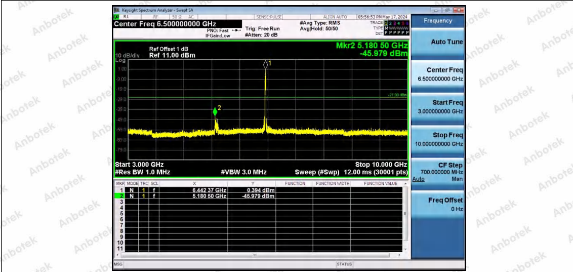
11AX20SISO-Ant1-6435-52Tone-RU40-3000~10000-PASS
