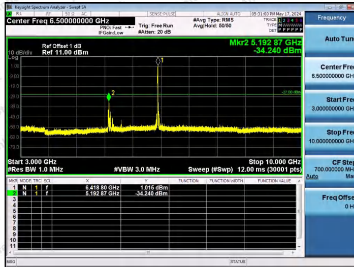
11AX20SISO-Ant1-6415-52Tone-RU39-3000~10000-PASS
