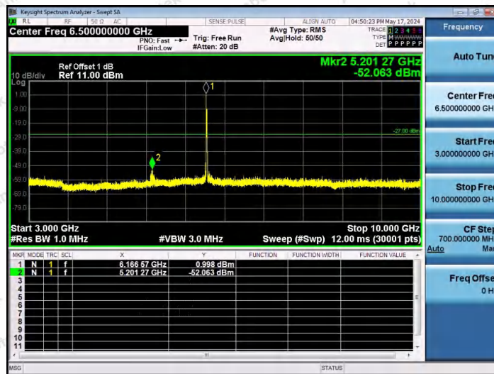
11AX20SISO-Ant1-6175-26Tone-RU0-3000~10000-PASS
