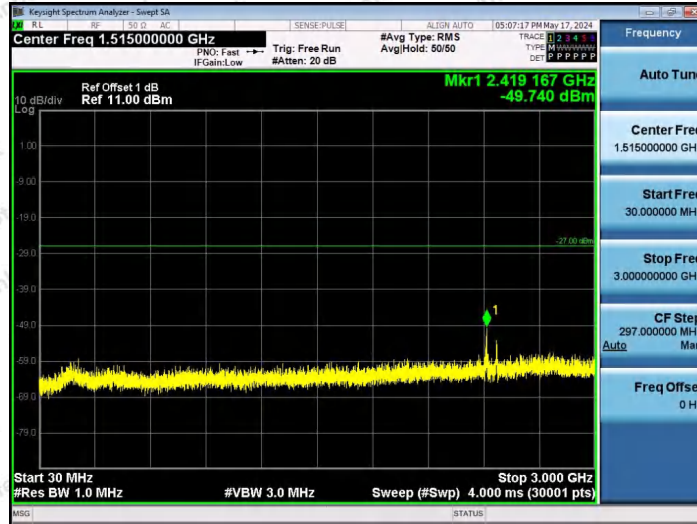
11AX20SISO-Ant1-6175-106Tone-RU53-30~3000-PASS
