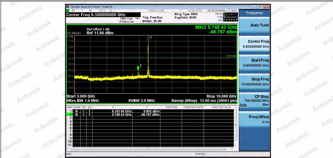
11AX20SISO-Ant1-6175-52Tone-RU40-3000~10000-PASS
