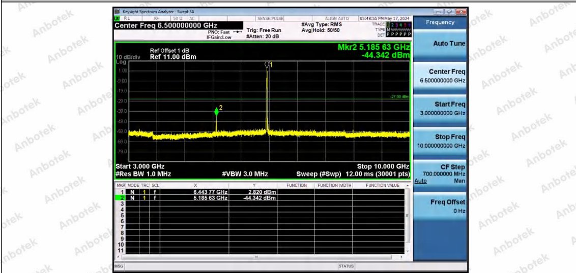
11AX20SISO-Ant1-6435-26Tone-RU8-3000~10000-PASS
