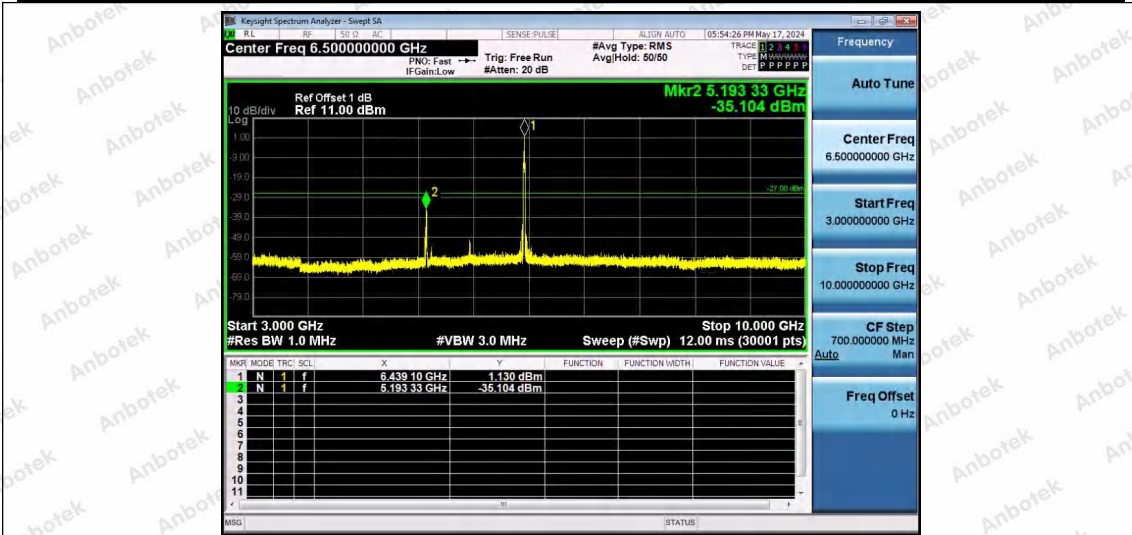
11AX20SISO-Ant1-6435-52Tone-RU39-3000~10000-PASS
