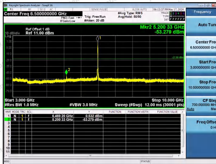
11AX20SISO-Ant1-6475-52Tone-RU37-3000~10000-PASS
