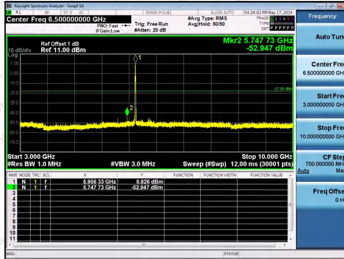
11AX20SISO-Ant1-5955-26Tone-RU4-3000~10000-PASS
