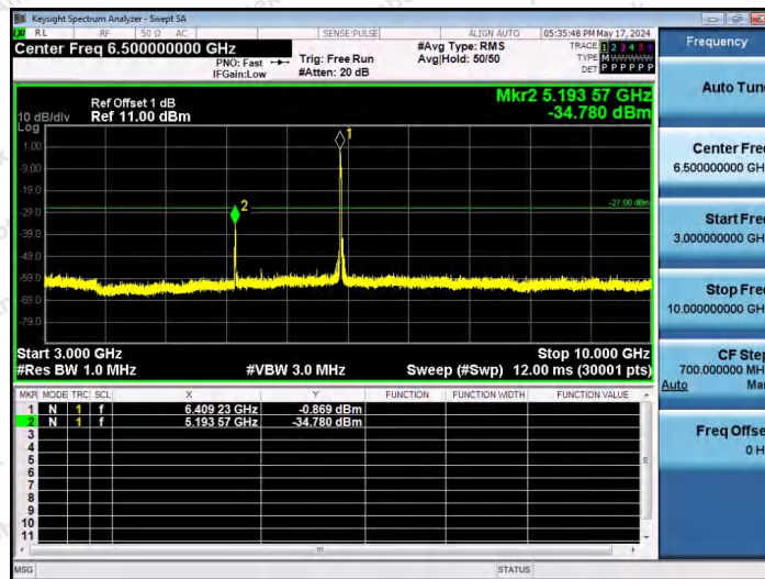
11AX20SISO-Ant1-6415-106Tone-RU53-3000~10000-PASS
