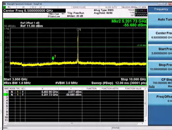
11AX20SISO-Ant1-6475-26Tone-RU8-3000~10000-PASS
