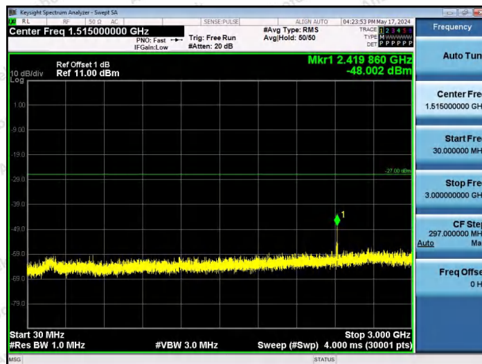
11AX20SISO-Ant1-5955-26Tone-RU4-30~3000-PASS
