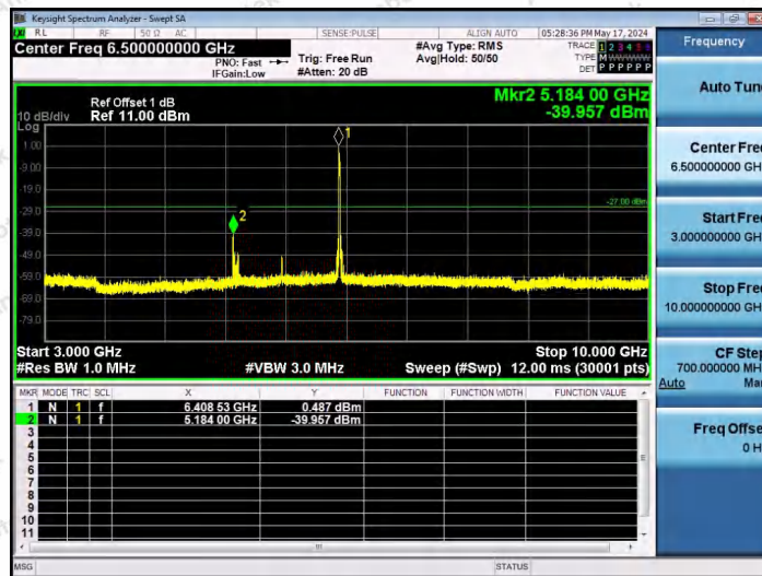
11AX20SISO-Ant1-6415-52Tone-RU37-3000~10000-PASS
