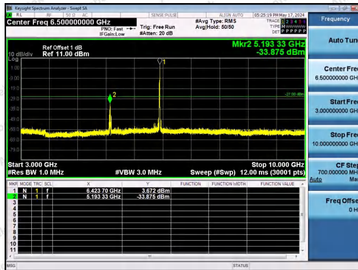
11AX20SISO-Ant1-6415-26Tone-RU8-3000~10000-PASS
