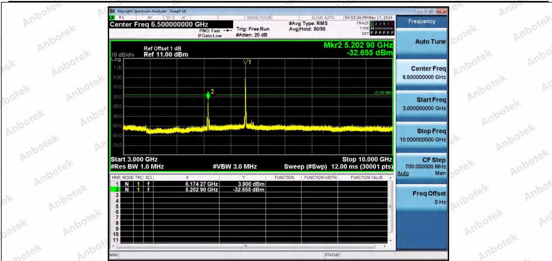
11AX20SISO-Ant1-6175-26Tone-RU4-3000~10000-PASS
