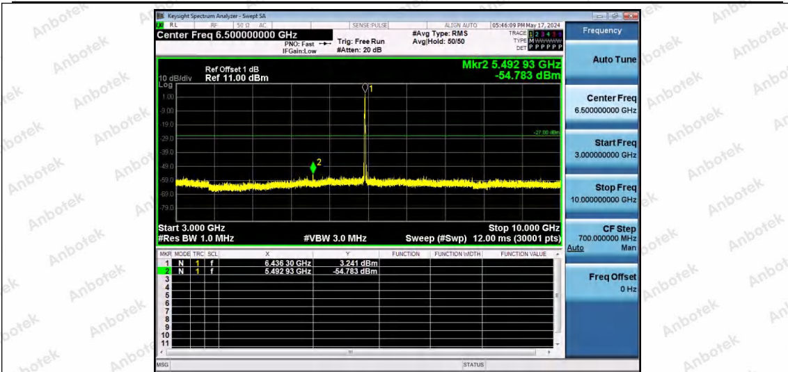
11AX20SISO-Ant1-6435-26Tone-RU4-3000~10000-PASS
