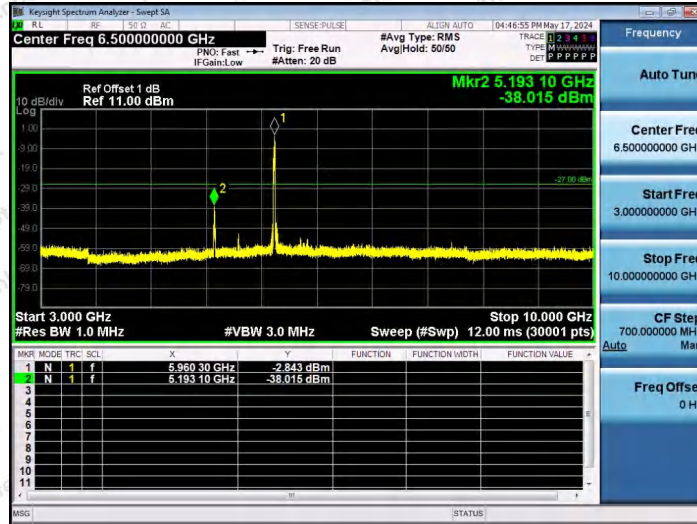
11AX20SISO-Ant1-5955-106Tone-RU54-3000~10000-PASS
