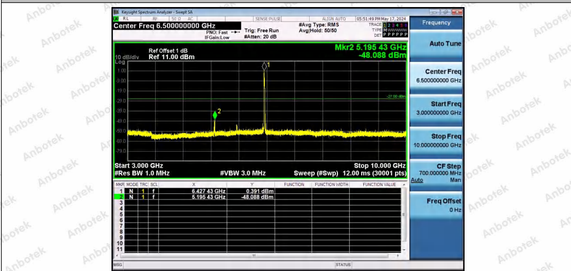
11AX20SISO-Ant1-6435-52Tone-RU37-3000~10000-PASS
