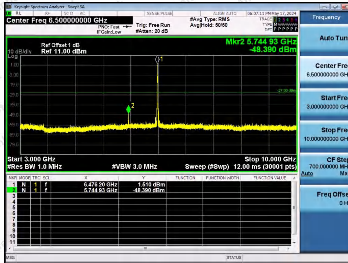
11AX20SISO-Ant1-6475-26Tone-RU4-3000~10000-PASS
