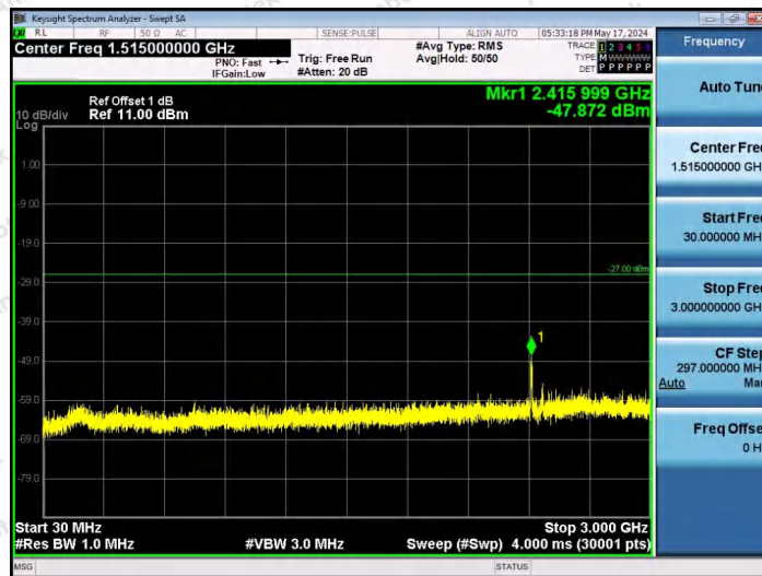
11AX20SISO-Ant1-6415-52Tone-RU40-30~3000-PASS
