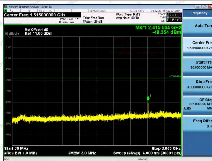
11AX20SISO-Ant1-5955-26Tone-RU8-30~3000-PASS
