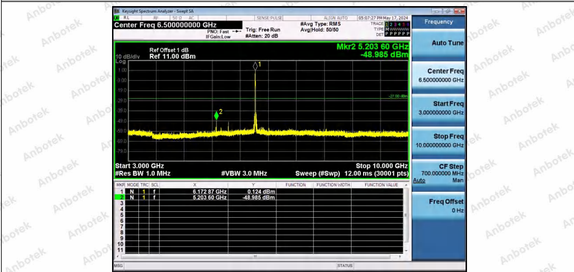
11AX20SISO-Ant1-6175-106Tone-RU53-3000~10000-PASS
