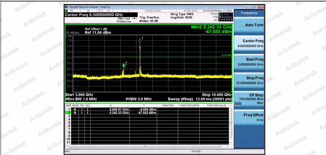
11AX20SISO-Ant1-5955-106Tone-RU53-3000~10000-PASS
