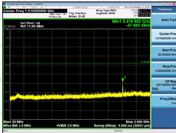
11AX20SISO-Ant1-6175-106Tone-RU54-30~3000-PASS
