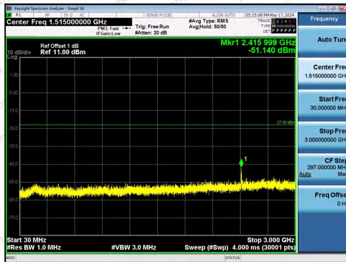
11AX20SISO-Ant1-6415-26Tone-RU8-30~3000-PASS
