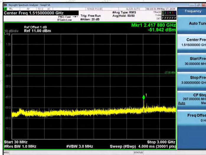
11AX20SISO-Ant1-6475-26Tone-RU8-30~3000-PASS
