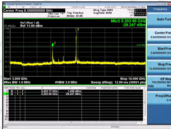
11AX20SISO-Ant1-6415-52Tone-RU40-3000~10000-PASS
