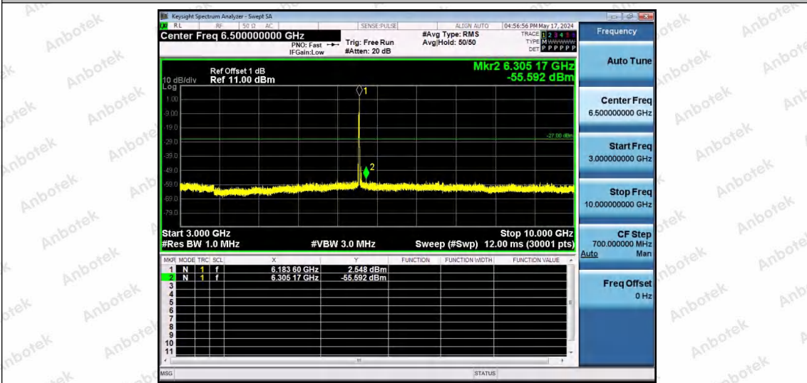
11AX20SISO-Ant1-6175-26Tone-RU8-3000~10000-PASS
