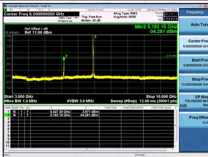
11AX20SISO-Ant1-6435-26Tone-RU0-3000~10000-PASS
