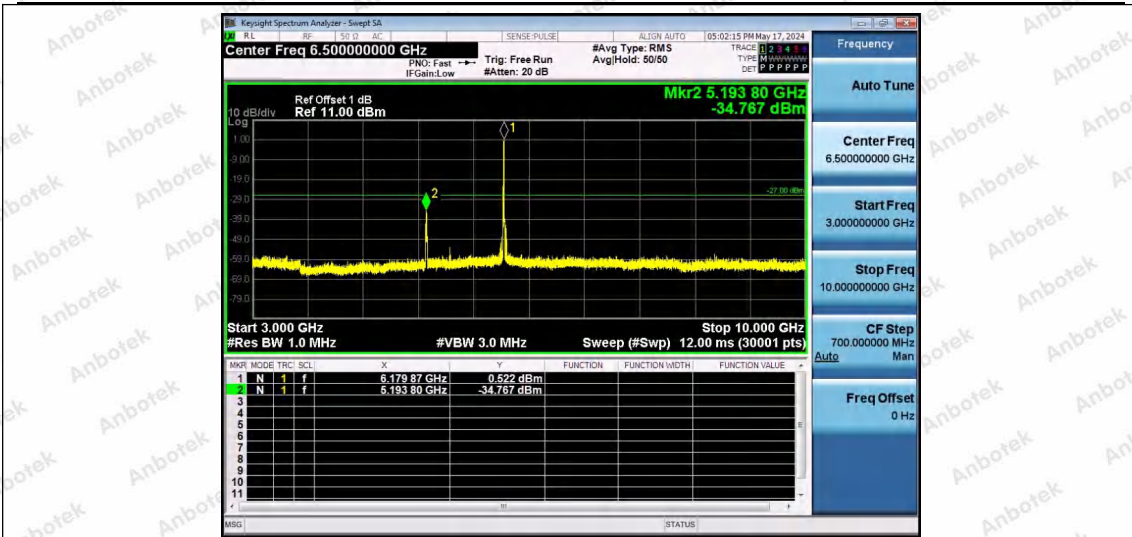
11AX20SISO-Ant1-6175-52Tone-RU39-3000~10000-PASS
