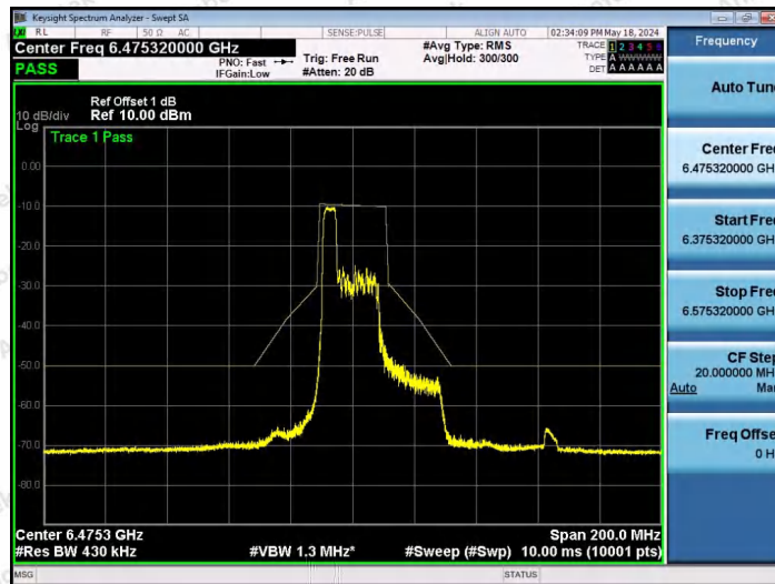
NTNV-11AX40SISO-Ant1-6485-52Tone-RU37-PASS
