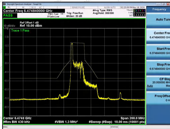
NTNV-11AX40SISO-Ant1-6485-26Tone-RU0-PASS
