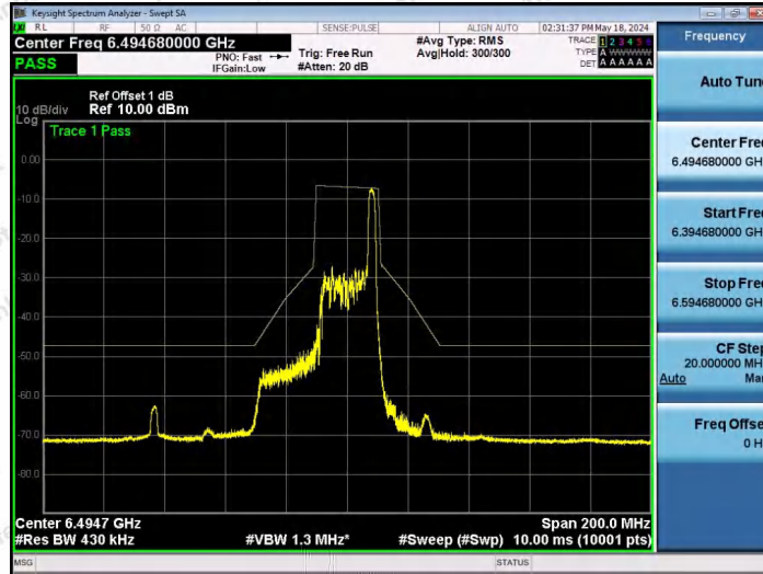
NTNV-11AX40SISO-Ant1-6485-26Tone-RU17-PASS
