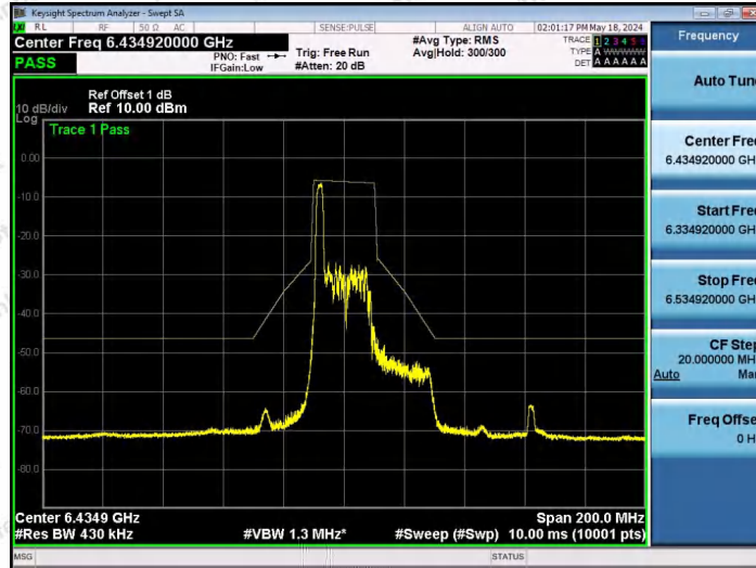
NTNV-11AX40SISO-Ant1-6445-26Tone-RU0-PASS
