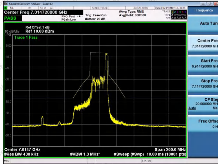
NTNV-11AX40SISO-Ant1-7005-26Tone-RU17-PASS
