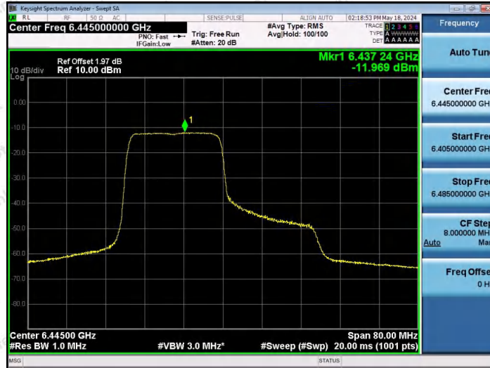
11AX40SISO-Ant1-6445-242Tone-RU61-PASS
