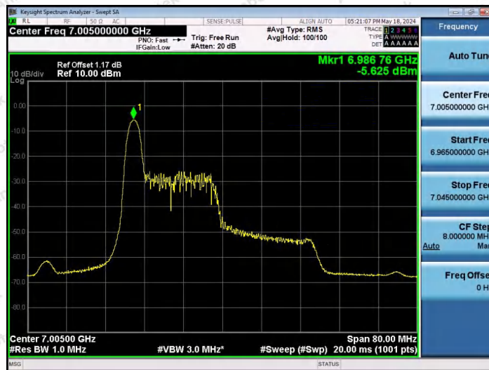
11AX40SISO-Ant1-7005-26Tone-RU0-PASS
