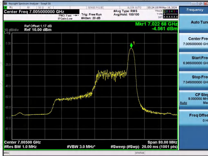
11AX40SISO-Ant1-7005-26Tone-RU17-PASS
