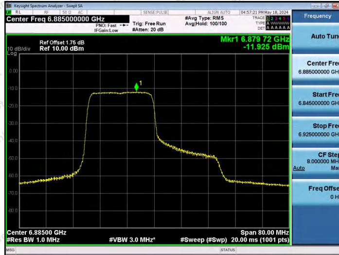
11AX40SISO-Ant1-6885-242Tone-RU61-PASS
