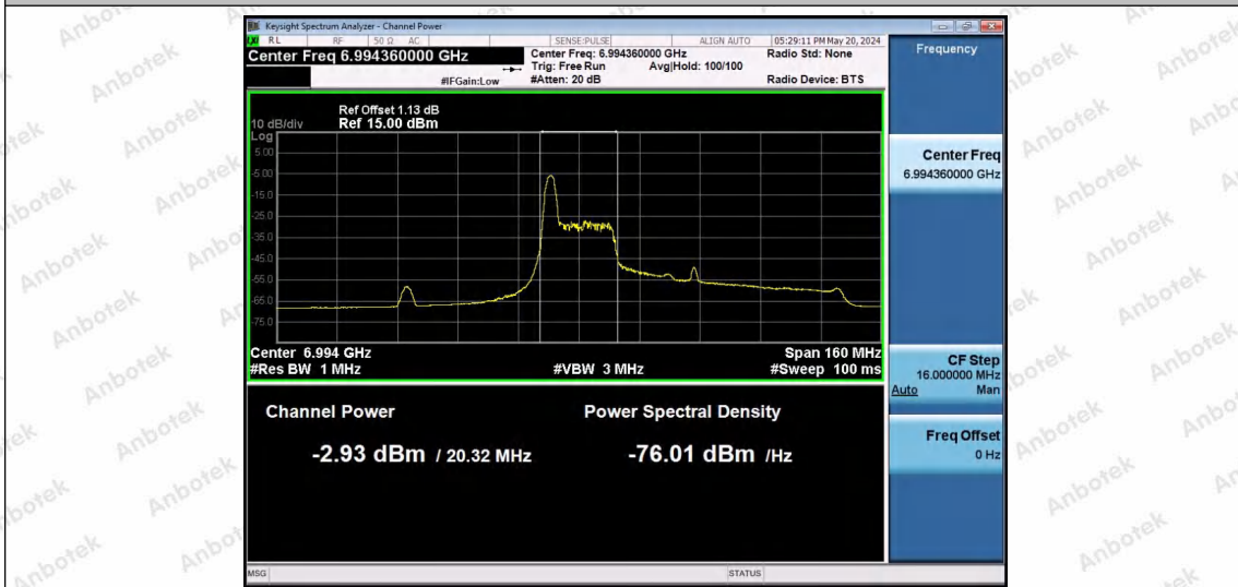
11AX80SISO-Ant1-7025-26Tone-RU0-PASS
