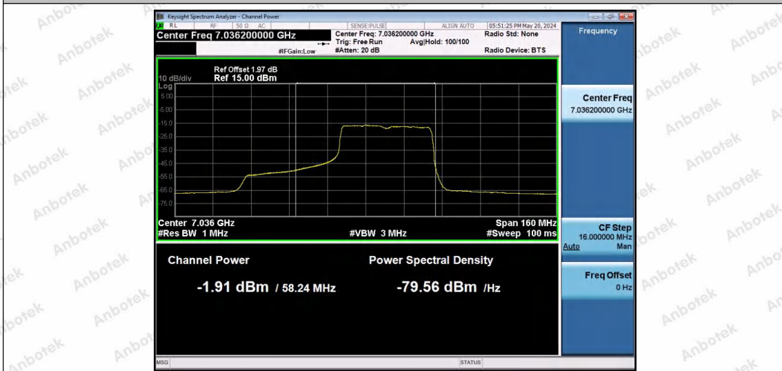
11AX80SISO-Ant1-7025-484Tone-RU66-PASS
