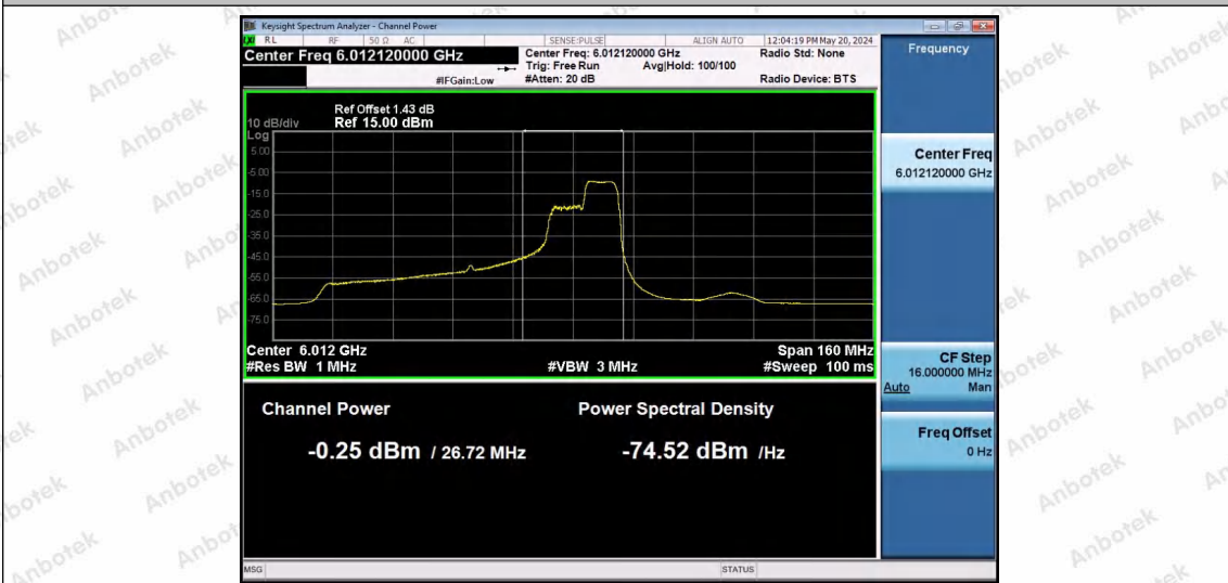
11AX80SISO-Ant1-5985-106Tone-RU60-PASS
