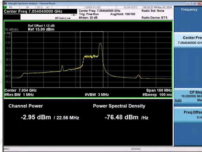
11AX80SISO-Ant1-7025-26Tone-RU36-PASS
