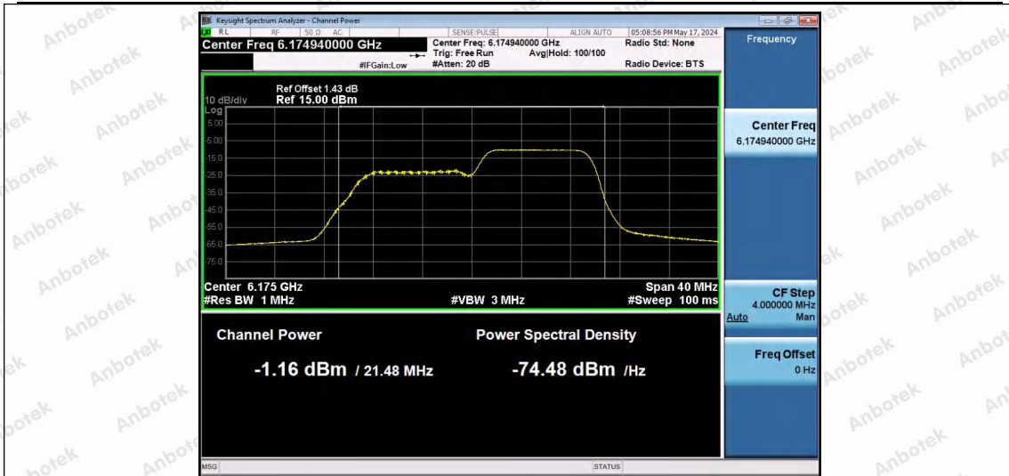
11AX20SISO-Ant1-6175-106Tone-RU54-PASS
