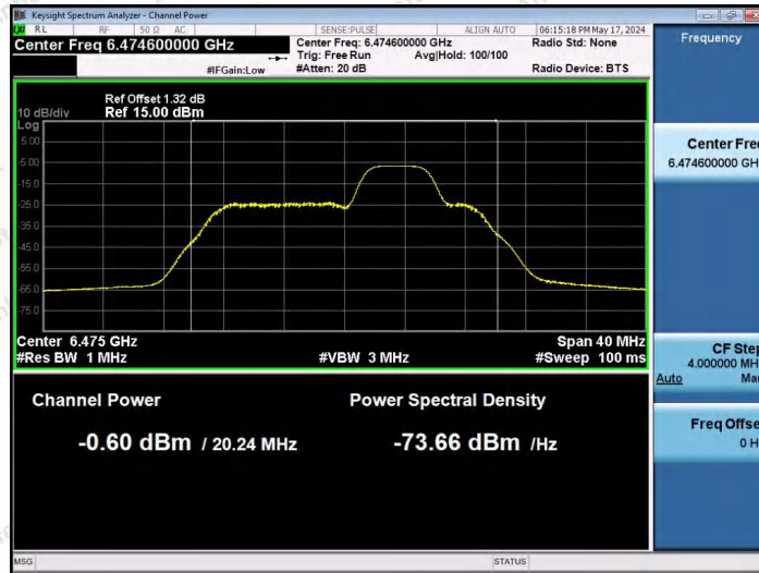
11AX20SISO-Ant1-6475-52Tone-RU39-PASS
