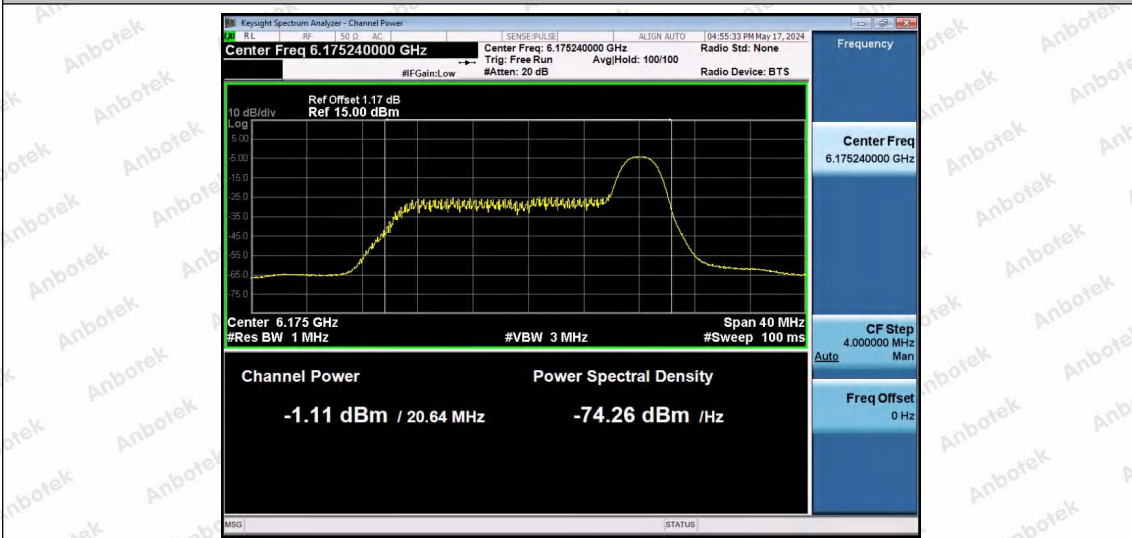
11AX20SISO-Ant1-6175-26Tone-RU8-PASS
