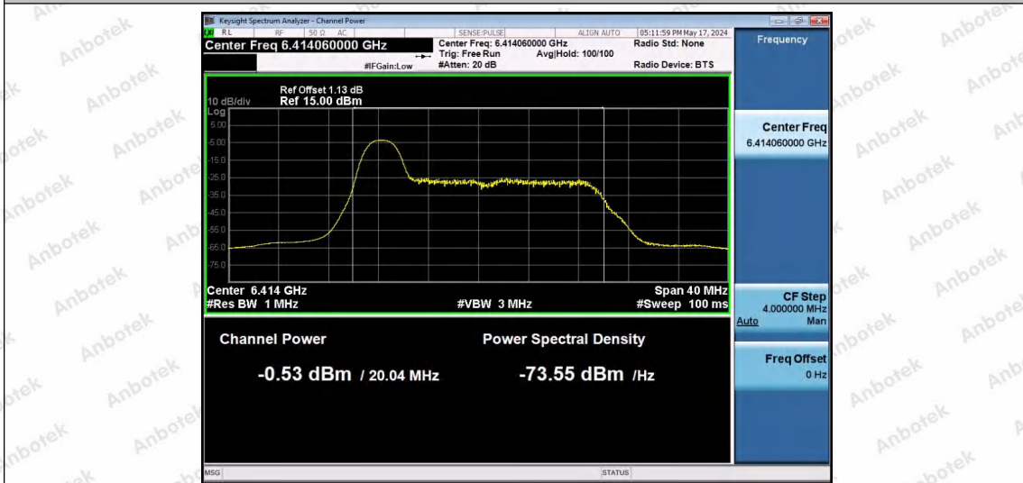
11AX20SISO-Ant1-6415-26Tone-RU0-PASS
