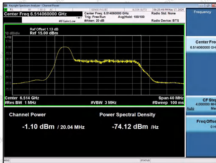
11AX20SISO-Ant1-6514-26Tone-RU0-PASS
