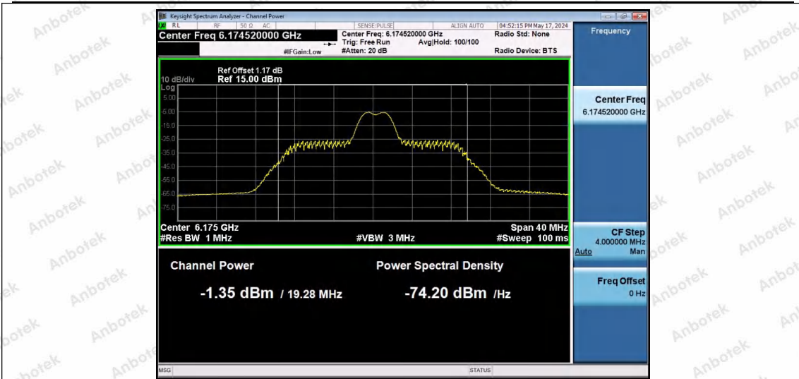
11AX20SISO-Ant1-6175-26Tone-RU4-PASS
