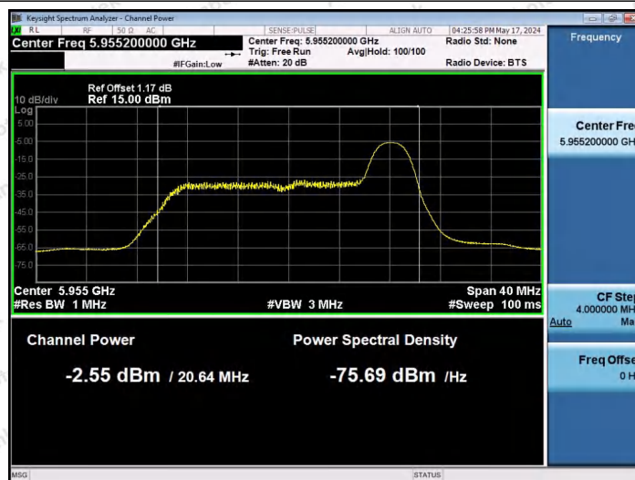
11AX20SISO-Ant1-5955-26Tone-RU8-PASS
