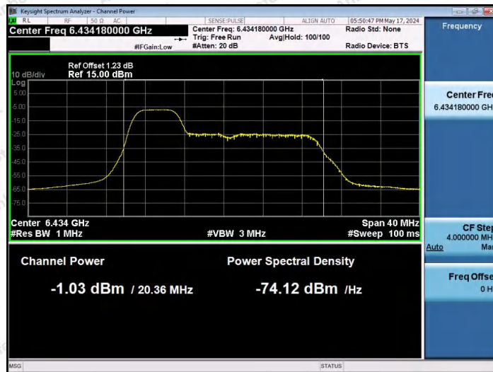
11AX20SISO-Ant1-6435-52Tone-RU37-PASS
