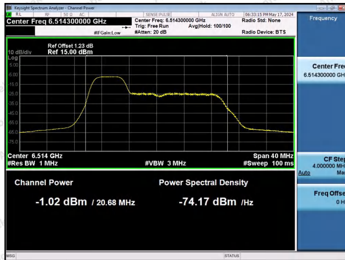
11AX20SISO-Ant1-6515-52Tone-RU37-PASS
