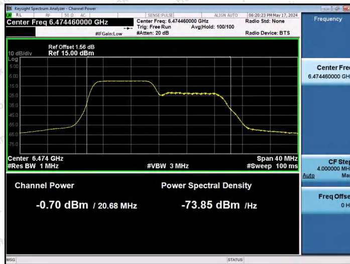
11AX20SISO-Ant1-6475-106Tone-RU53-PASS
