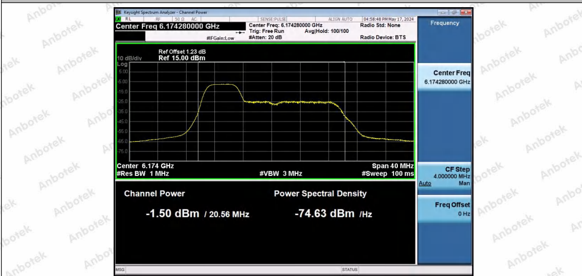
11AX20SISO-Ant1-6175-52Tone-RU37-PASS
