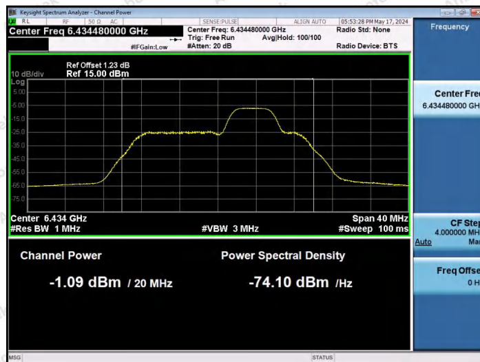
11AX20SISO-Ant1-6435-52Tone-RU39-PASS
