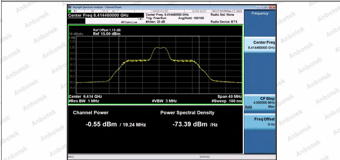
11AX20SISO-Ant1-6415-26Tone-RU4-PASS
