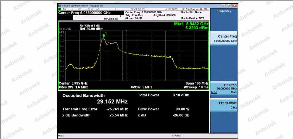
11AX80SISO-Ant1-5985-52Tone-RU37-PASS
