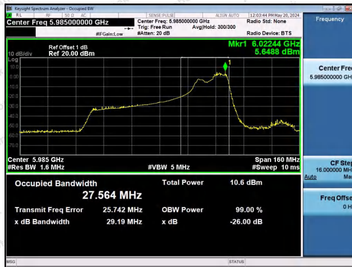
11AX80SISO-Ant1-5985-106Tone-RU60-PASS
