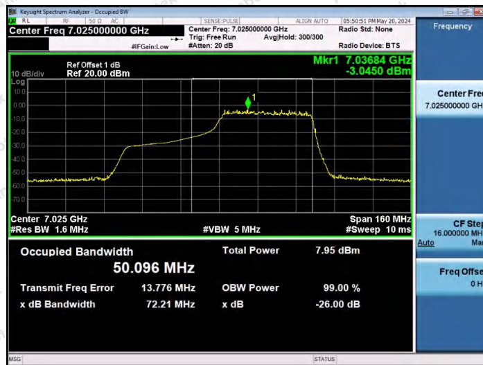
11AX80SISO-Ant1-7025-484Tone-RU66-PASS
