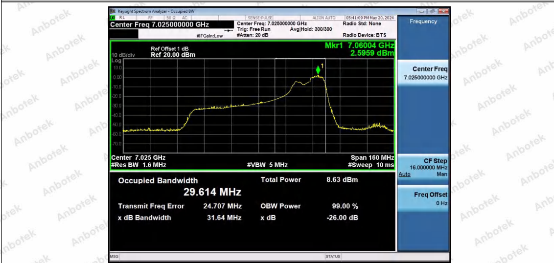
11AX80SISO-Ant1-7025-106Tone-RU60-PASS
