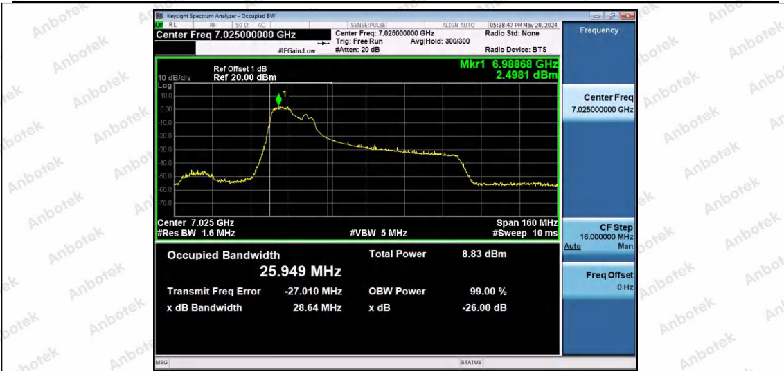
11AX80SISO-Ant1-7025-106Tone-RU53-PASS
