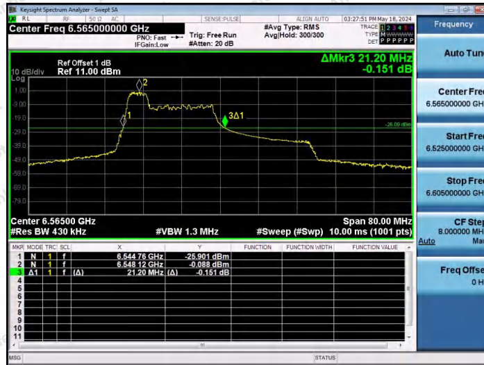
11AX40SISO-Ant1-6565-52Tone-RU37
