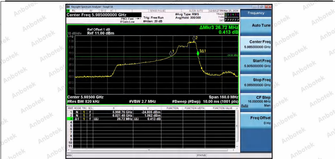
11AX80SISO-Ant1-5985-106Tone-RU60
