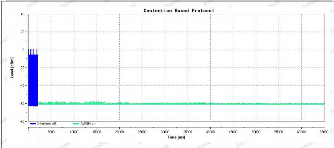
11AX20SISO-Ant1-5955-5955-PASS
