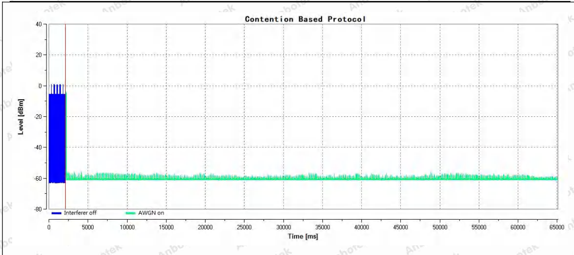
11AX20SISO-Ant1-6895-6895-PASS
