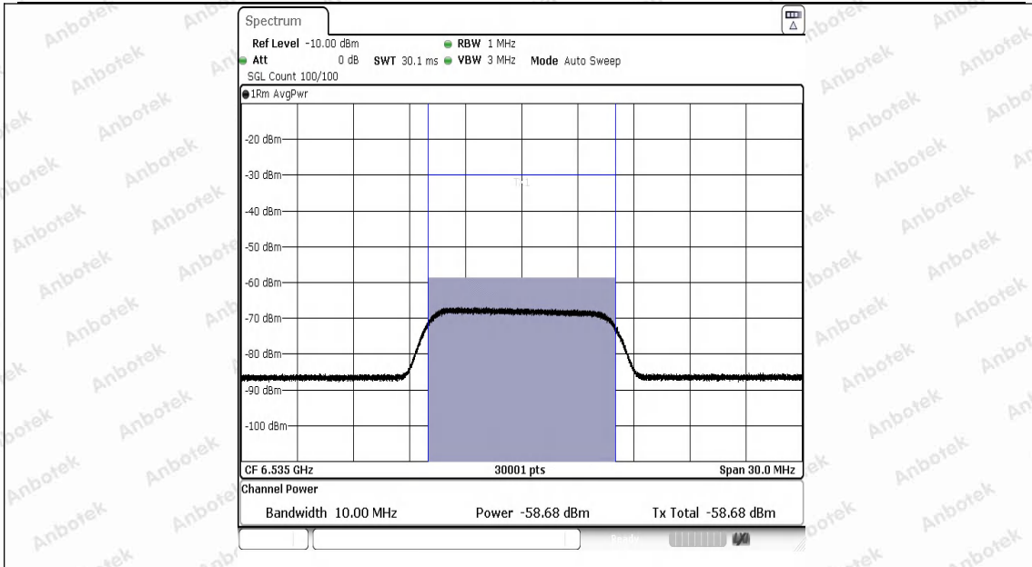
11AX20SISO-Ant1-6535-6535-PASS
