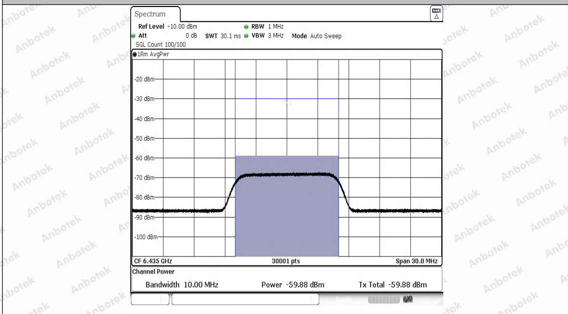
11AX20SISO-Ant1-6435-6435-PASS
