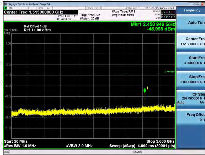
11AX40SISO-Ant1-6885-30~3000-PASS
