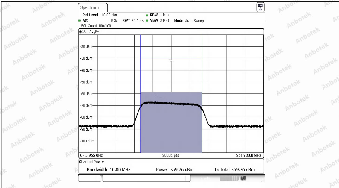
11AX20SISO-Ant1-5955-5955-PASS
