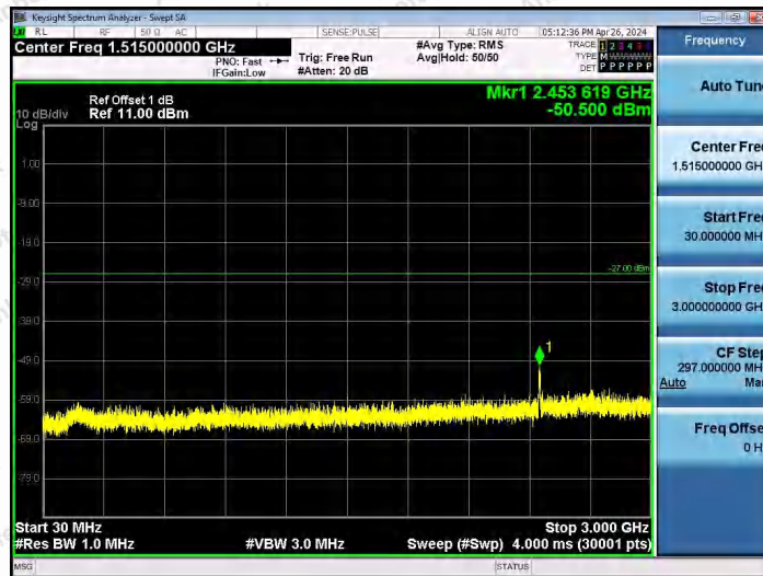
11AX40SISO-Ant1-6685-30~3000-PASS
