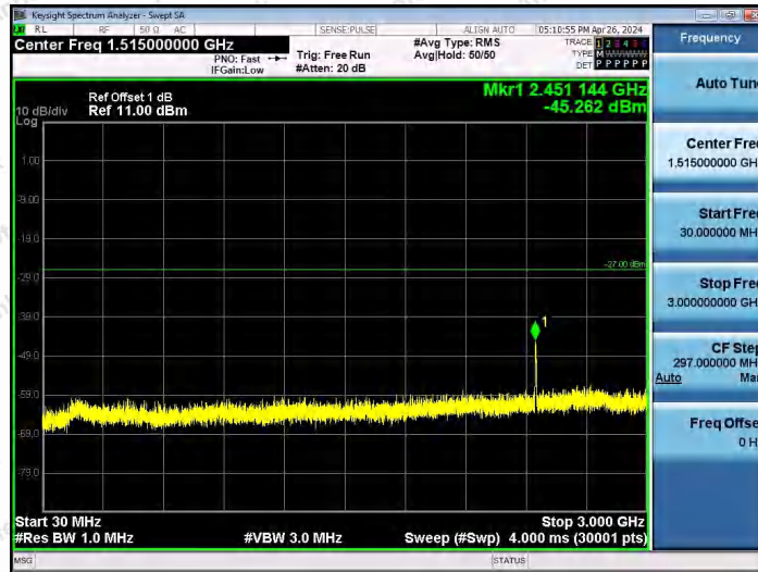
11AX40SISO-Ant1-6565-30~3000-PASS
