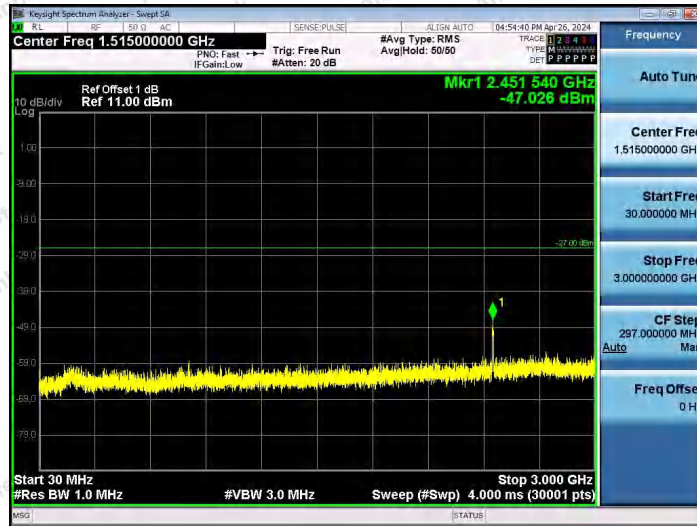
11AX40SISO-Ant1-5965-30~3000-PASS
