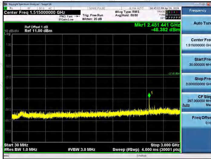
11AX20SISO-Ant1-7015-30~3000-PASS
