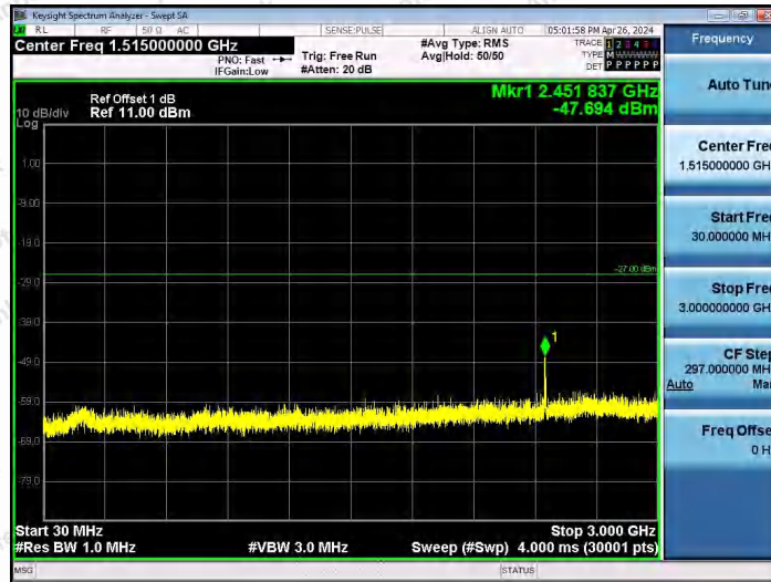
11AX40SISO-Ant1-6445-30~3000-PASS
