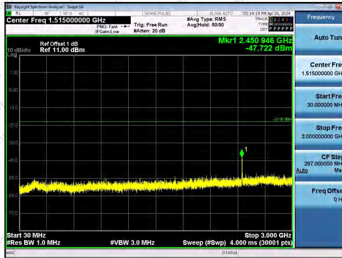
11AX40SISO-Ant1-6845-30~3000-PASS
