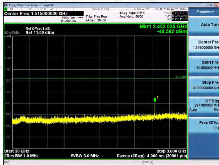
11AX20SISO-Ant1-7115-30~3000-PASS
