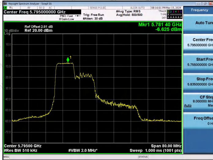
11AX40SISO-Ant1-5795-106Tone-RU53-PASS
