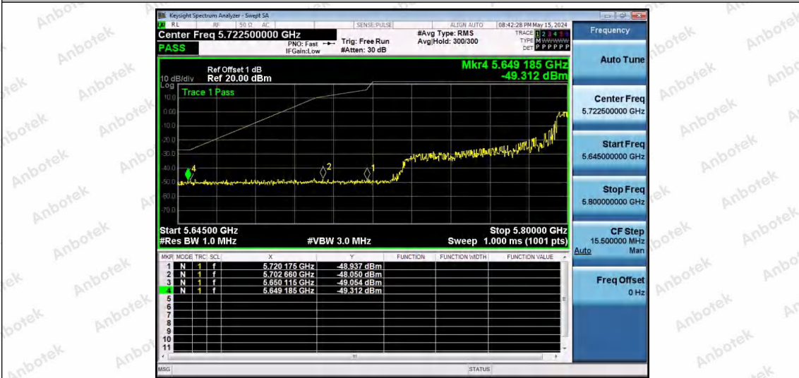
11AX80SISO-Ant1-5775-26Tone-RU36-PASS
