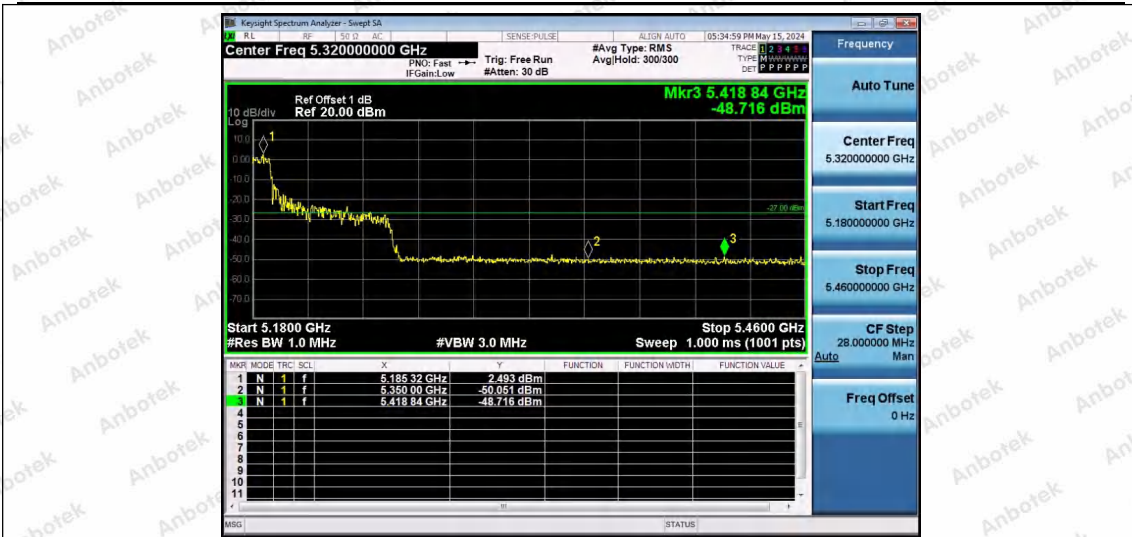
11AX80SISO-Ant1-5210-26Tone-RU0-PASS
