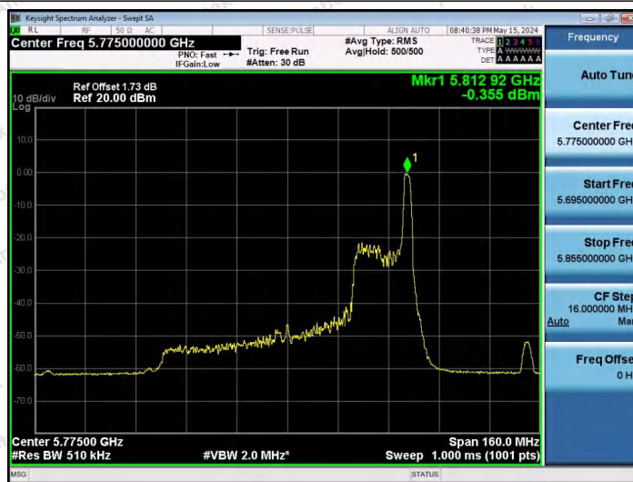
11AX80SISO-Ant1-5775-26Tone-RU36-PASS
