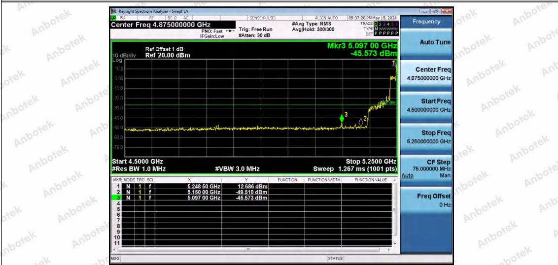
11AX80SISO-Ant1-5210-26Tone-RU36-PASS
