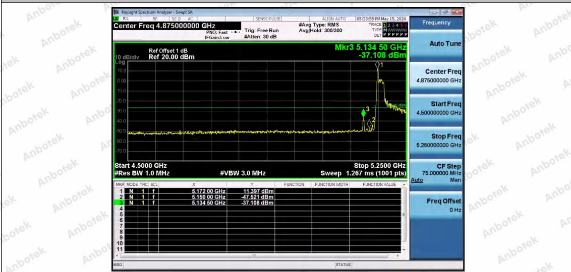
11AX80SISO-Ant1-5210-26Tone-RU0-PASS
