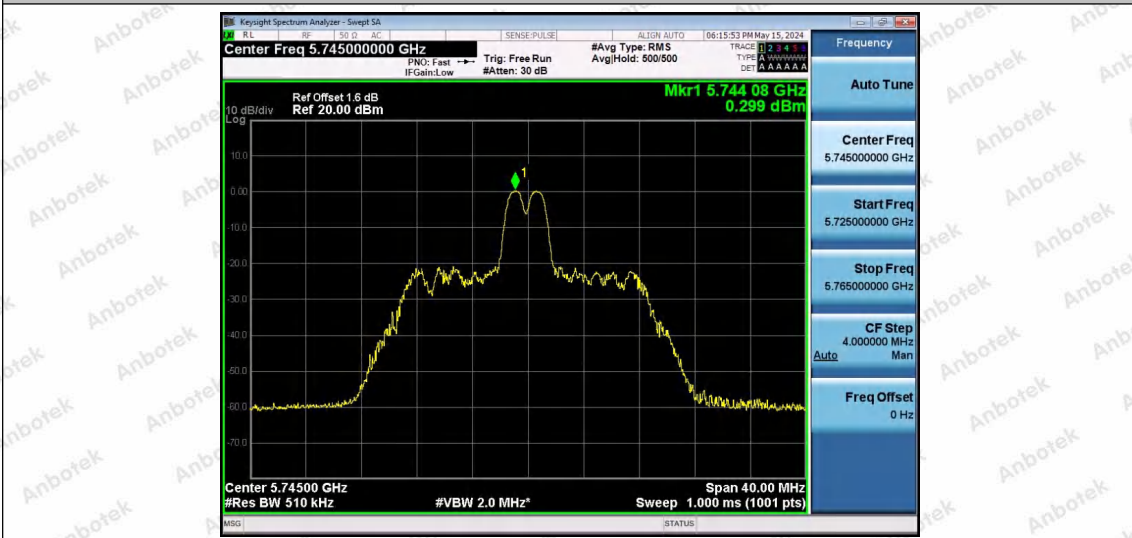
11AX20SISO-Ant1-5745-26Tone-RU4-PASS
