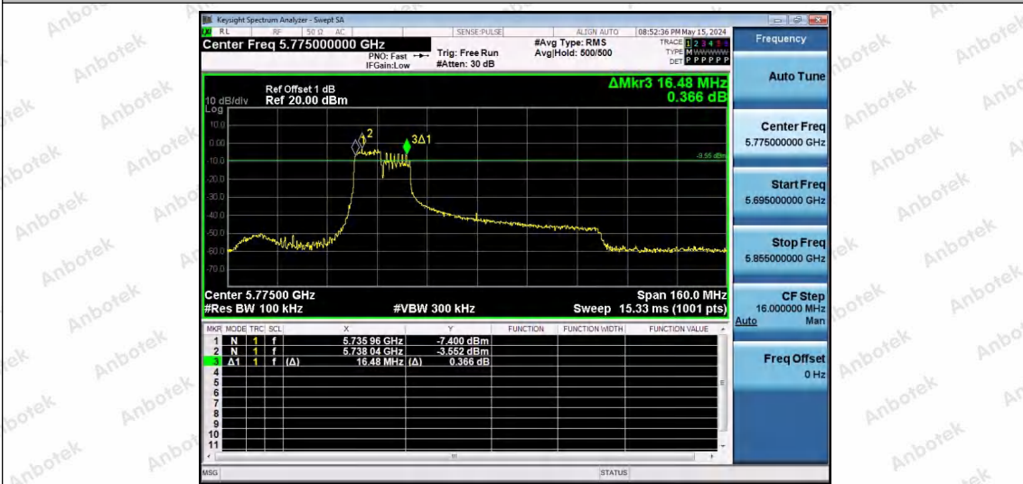
11AX80SISO-Ant1-5775-106Tone-RU53-PASS
