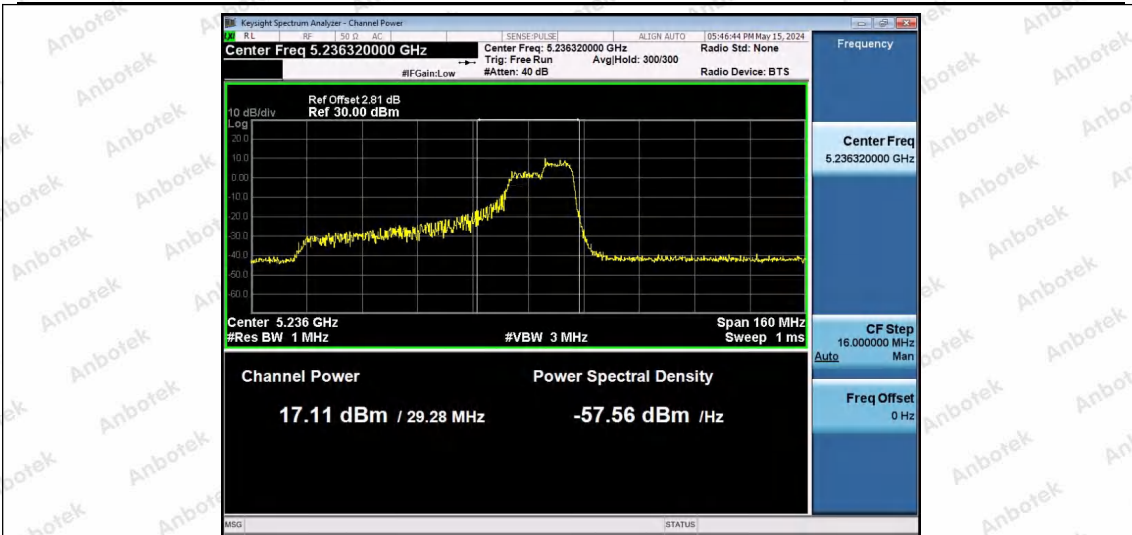
11AX80SISO-Ant1-5210-106Tone-RU60-PASS
