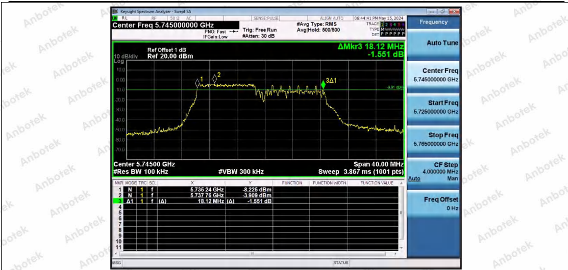
11AX20SISO-Ant1-5745-106Tone-RU53-PASS
